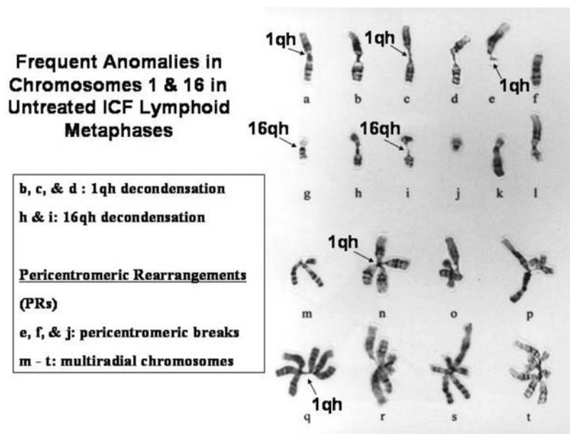
Figure 2. Examples of chromosome 1 and 16 homologues displaying pericentromeric anomalies in metaphases from untreated ICF lymphoblastoid cells. a , normal Chr1 and g , normal Chr16; b-d and h and i , different extents of decondensation of the qh region of Chr1 or Chr16; e and f , the two fragments derived from a chr16(1)(qh) in one metaphase with the 1p arm ( e ) and the acentric 1q arm ( f ) (note the decondensed qh below the centromeric constriction of the 1p arm); j , del(16)(qh) ; k , der(16)(1;16)(q10;p10) ; l , der(1)t(1;16)(p10;q10) . In m-t are multiradials from diploid cells, with the exception of q which was from a tetraploid LCL B metaphase; m , triradial(1;16)(q,q;p); n , quadriradial(1)(p,p,q,q,q); o , quadriradial(1;16)(p,q;p,q,q); p , pentaradial(1;16)(p,q;p,q,q,q); q , hexaradial(1)(p,p,q,q,q,q,q); r , hexaradial(1;16)(p,p,q,q;p,q,q,q); s , hexaradial(1;16)(p,q,q;p,q,q,q); t , octaradial(1;16)(p,p,q,q;p,q,q,q,q). Note the frequent decondensation of at least one qh region in the multiradials.
