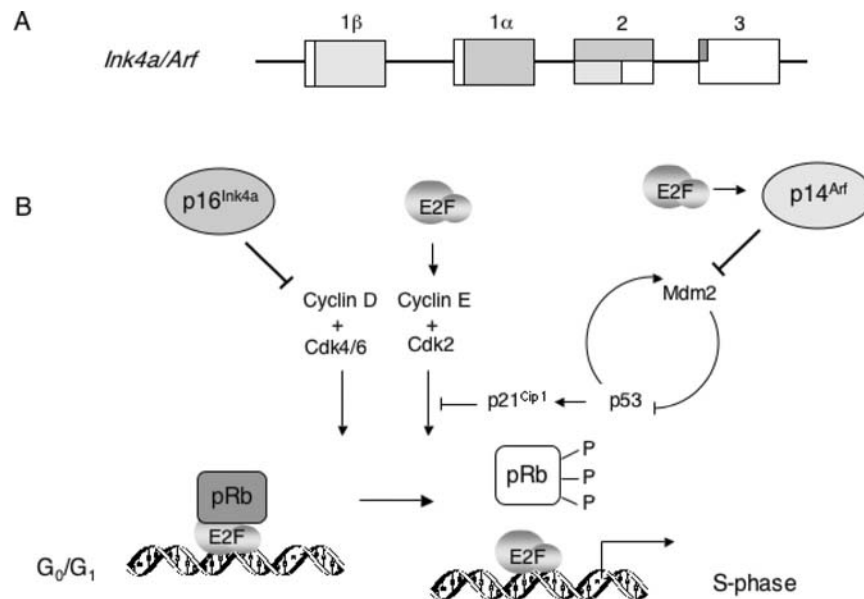
Figure 1. A. Organisation of the Ink4a/Arf locus. The Ink4a/Arf locus on human chromosome 9p21 (mouse chromosome 4) has two promoters and alternative first exons (1 \alpha and 1 \beta ) that are spliced to the same second and third exons. The \alpha transcript encodes Ink4a (darker shading) and the \beta transcript encodes Arf (lighter shading). The Arf sequences specified by exon 2 are translated in the -1 reading frame relative to that of Ink4a. B. The G_0/G_1 to S phase transition in mammalian cells. Current understanding of G_1 progression envisages sequential phosphorylation of the retinoblastoma protein (pRb) and its relatives by the cyclin D-dependent kinases Cdk4 and Cdk6 followed by cyclin E-Cdk2. This releases the repressive influence of pRb on the E2F family of transcription factors and allows the temporally ordered expression of genes required for S-phase. Cyclin E expression is E2F-dependent and the activity of Cdk2 is also modulated by the extent to which the p21 Cip1 /p27 Kip1 Cdk inhibitors are sequestered in cyclin D-dependent complexes. By binding directly to Cdk4 and 6, Ink4a prevents them from associating with D cyclins and causes redistribution of p21 Cip1 /p27 Kip1 onto cyclin E-Cdk2. Levels of p21 Cip1 are also regulated by the p53 transcription factor. The activity of p53 is in turn controlled by Mdm2, an E3 ubiquitin ligase that promotes the proteasome-mediated destruction of p53 as well as directly blocking its transcription activity. As the expression of Mdm2 is p53 dependent, there is a feedback loop through which p53 activity is tightly constrained. Arf interferes with this balance by binding to Mdm2 and inhibiting its ubiquitin ligase activity, thereby stabilising p53. Inactivation of pRb also impacts on this pathway because expression of Arf is activated by E2F. In a further feedback loop, p53 appears to repress the transcription of Arf.
