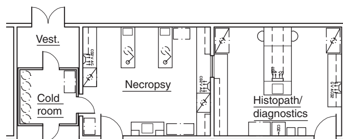
Fig. 19-6 Histopathology/diagnostic laboratory suite.
