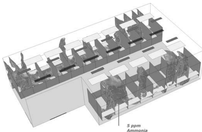
Fig. 35-4 Isosurface of 5 ppm of ammonia in a kennel.
