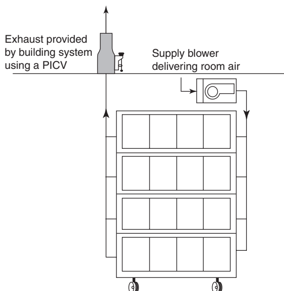
Fig. 20-16 Schematic and photograph of an individually ventilated cage rack of the room supply, direct exhaust type. In the system shown, exhaust is provided by the building's system and therefore, no rack exhaust blower is provided. Exhaust stability is ensured with the use of a PICV. Schematic courtesy of Phoenix Corporation, Inc.
