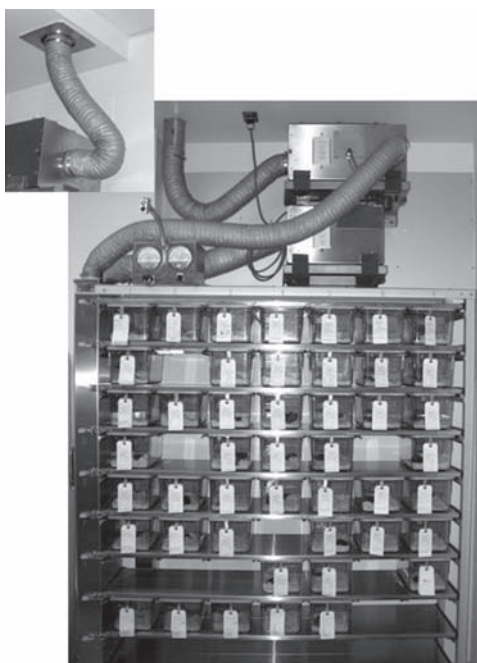
Fig. 20-17 Schematic and photograph of an individually ventilated cage rack of the room supply, direct exhaust type. In the system shown, exhaust is provided by an exhaust blower on the rack and delivered to the building's exhaust system through a direct connection. A thimble connection (inset) can also be used. Schematic courtesy of Phoenix Corporation, Inc.
