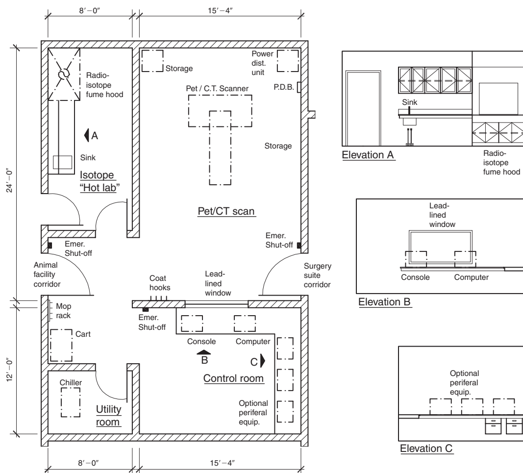
Fig. 19-21 Positron emission tomography/computed tomography (PET/CT) suite.
