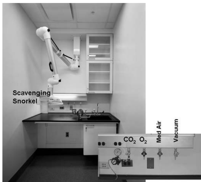
Fig. 20-8 A typical rodent procedure laboratory containing a scavenging snorkel arm, sink, various gases for anesthesia ( O_2 and medical air) and euthanasia ( CO_2 ), and vacuum. A knee-hole in the casework is for seated bench work.
