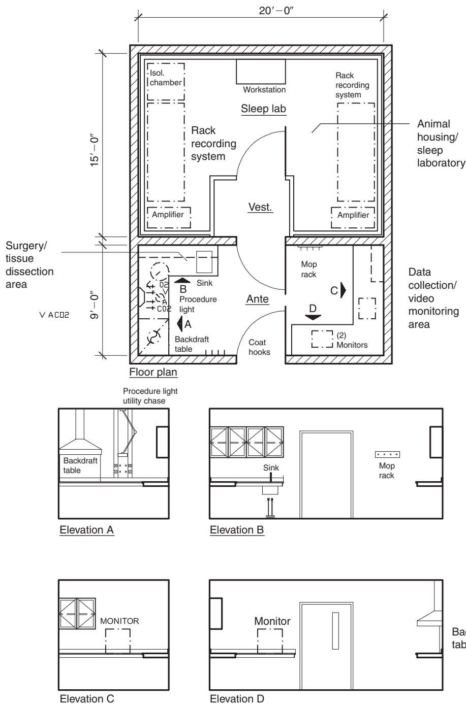
Fig. 19-16 Sample rodent sleep laboratory.
