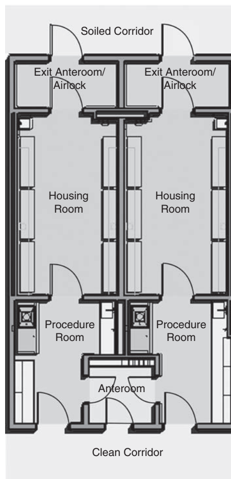
Fig. 25-12 Containment facility housing/procedure suite.
