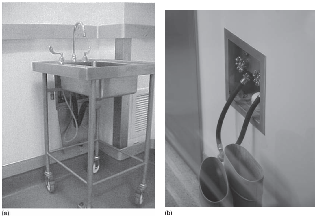
Fig. 18-8 Flexibility afforded by providing plumbing for portable sinks: (a) a portable sink connected to the plumbing; (b) the plumbing without the sink connected. This allows for the use of a sink in the room when needed, without having a permanently mounted sink there.
