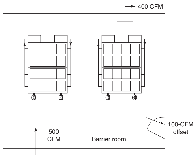
Fig. 34-4 Volumetric offset method of controlling room directional airflow.
