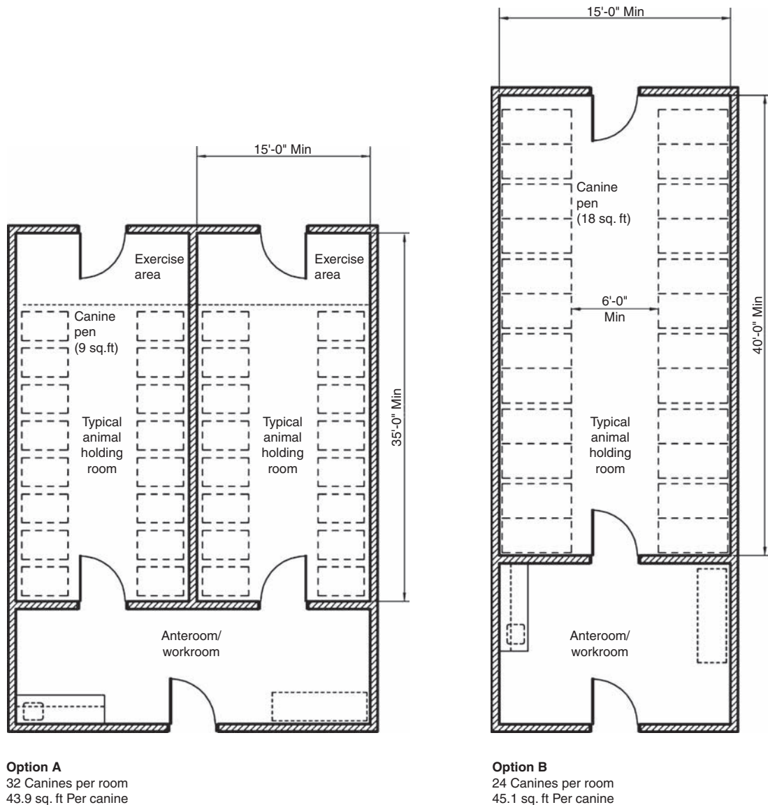
Fig. 4-10 Canine suite diagrams.
