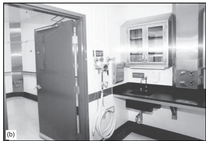
Fig. 19-12 (a) Procedure laboratory/anteroom. (b) Dedicated procedures laboratory. This is a view of an anteroom looking into an animal holding room (opened door). Wall-mounted upper cabinets and lower work surface with sink, and a stainless-steel utility (moisture-resistant electrical outlets, air, vacuum, carbon dioxide and natural gas) service chase are shown. Note that none of the casework extends to the finished floor, which facilitates cleaning.
