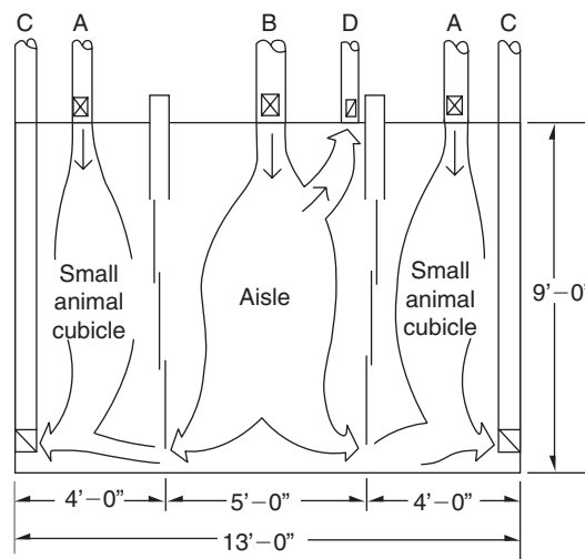
Fig. 15-6 Option 2 ventilation pattern for small animal cubicles: A, building air supply to cubicles; B, building air supply to aisle; C, to building exhaust from animal cubicles; D, to building exhaust from animal procedure area. Also illustrated is a three-panel vertical stacking door for each cubicle.
