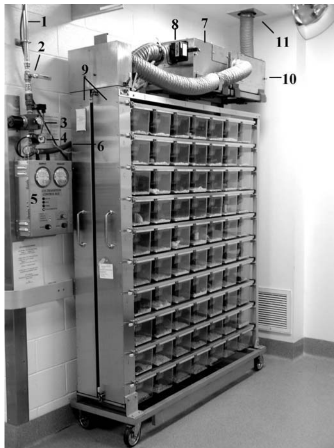
Fig. 20-14 Automated individually ventilated rack system for euthanasia: 1, building CO 2 supply; 2, manual ball valve; 3, high-pressure regulator; 4, solenoid-controlled female-valved coupler; 5, CO 2 transition control box; 6, high-pressure CO 2 hose; 7, supply blower; 8, motorized gate damper; 9, supply and exhaust plenums; 10, exhaust blower; and 11, thimble connection. Reproduced from McIntyre et al. (2007).
