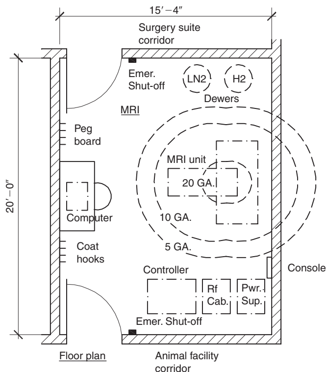
Fig. 19-20 Magnetic resonance imaging (MRI) room.
