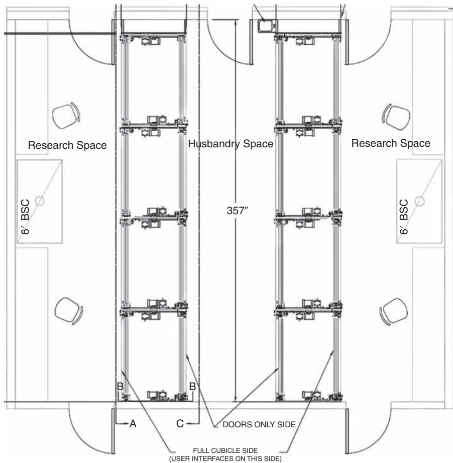
Fig. 15-2 Animal cubicles that open from both sides.
