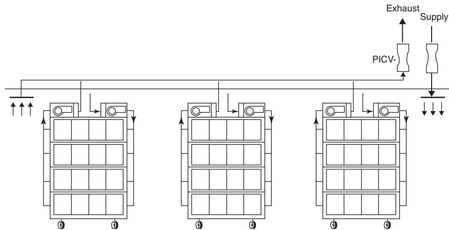
Fig. 20-21 Schematic of room supply, direct exhaust individually ventilated cage racks in which the exhaust blowers are direct connected to the building's system. The exhaust duct into which the racks empty effluent also provides room exhaust. The duct is served by a single PICV set to meet the exhaust requirement of all the racks in addition to the room. Changes in individual rack exhaust volumes which may occur are offset by changes in the room exhaust volume.
