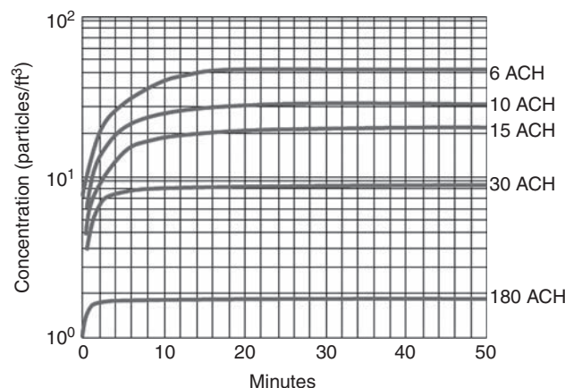
Fig. 25-13 Effect of ventilation rate in air changes per hour (ACH) on particle concentration in a space with continuous particle emission.
