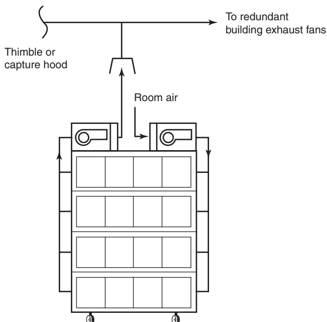
Fig. 34-7 Option 1: supply – room air via filter/fan module for each rack; exhaust thimble (decoupled) connection to building exhaust.
