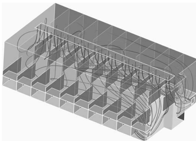
Fig. 35-3 Path lines migrating through a kennel.
