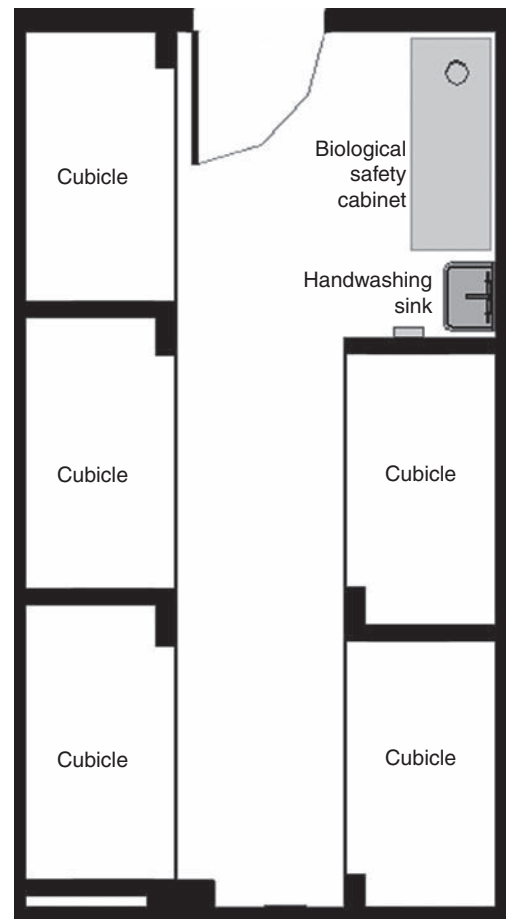
Fig. 25-10 Cubicle room layout.
