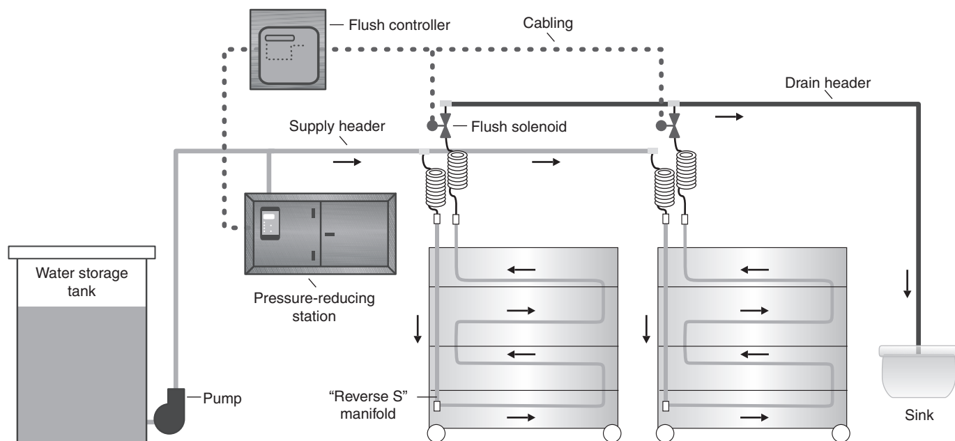
Fig. 32-8 A schematic drawing of a non-recirculating system that features the capability to flush the rack manifolds. This figure also demonstrates the “reverse S” design feature for rack manifolds.
