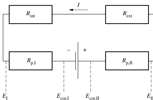
Figure 7.4 Electrical equivalent circuit of corrosion cell.
