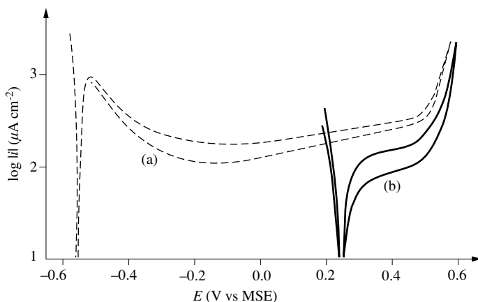
Figure 6.5 Anodic polarization curve of Fe-66Ni-16Mo in 50% \text{H}_2\text{SO}_4 in absence (a) and in presence (b) of 42g \text{Fe}_2(\text{SO}_4)_3 ; Sweep rate is 0.33 mV/s, T = 125^\circ\text{C} [2].
