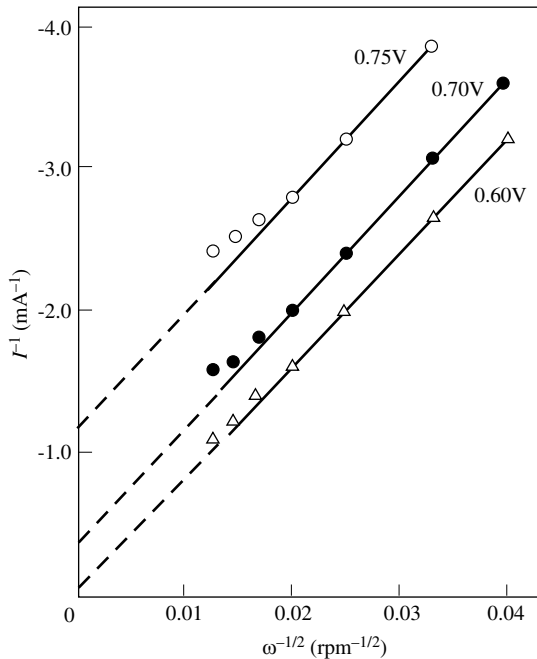
Figure 4.30 Koutecky-Levich plot for reduction of \text{Fe(CN)}_6^{3-} to \text{Fe(CN)}_6^{4-} on a 0.385 \text{ cm}^2 platinum rotating disk electrode under mixed control in 0.5\text{M K}_2\text{SO}_4 , at 28^\circ\text{C} . The reciprocal of the measured current is shown as a function of \omega^{-1/2} for three potentials [12].
