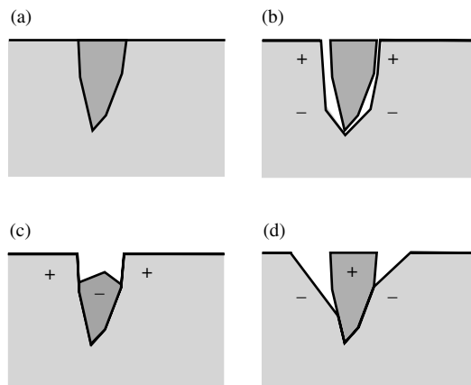
Figure 7.54 Effect of inclusions on pit initiation: (a) unattacked surface with an inclusion; (b) formation of an aeration cell in the space between an inert inclusion and the metal; (c) anodic dissolution of the inclusion; (d) formation of a corrosion cell between the cathodic inclusion and the metal.
