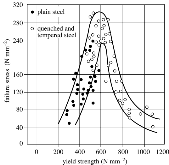
Figure 11.27 Failure stress versus yield strength for carbon steels. The failure stress was measured by placing the specimens in a 5% NaCl solution saturated with \text{H}_2\text{S} for 100 hours at ambient temperature [12].
