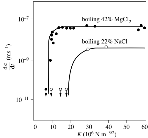
Figure 11.13 Crack-propagation rate versus stress intensity factor for a type-304 austenitic stainless steel: (o) boiling 22% NaCl solution (105 °C); (•) boiling 42% MgCl solution (130 °C).
