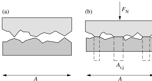
Figure 10.5 Contact of two rough surfaces of ductile materials.
