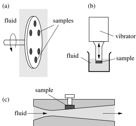
Figure 10.36 Experimental study of cavitation corrosion: (a) rotating disk in the turbulent-flow regime; (b) vibrating device; and (c) Venturi system.
