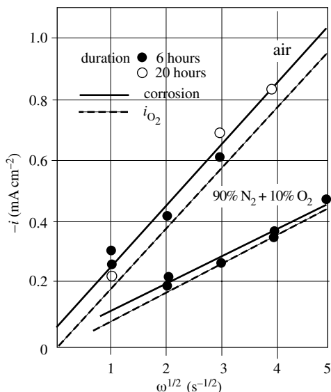
Figure 4.39 Variation of corrosion rate and of cathodic limiting current with rotation rate in air and in N 2 + 10% O 2 . The rates after 6 and 20 hours are shown. Dashed line: limiting current density of the oxygen reduction measured under comparable conditions. Electrolyte: 0.2M Na 2 SO 4 , pH 2.7.
