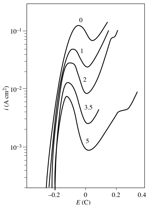
Figure 6.14 Polarization curves of Fe-13Cr- x Mo stainless steels in 1M HCl, showing the effect of alloyed molybdenum on the passivation current density. T = 30^\circ\text{C} , x = 0, 1, 2, 3.5, 5\% [9].
