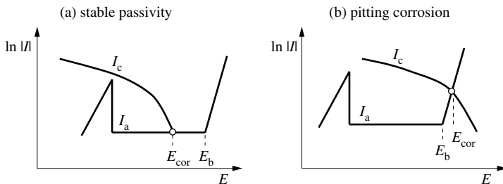
Figure 7.48 Evans diagram of a passive electrode showing the sensitivity to pitting corrosion (schematic): (a) E_{\text{cor}} < E_b ; and (b) E_{\text{cor}} > E_b .
