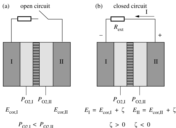
Figure 7.14 Principle of aeration cells operating under (a) open and (b) closed circuit conditions. R_{ext} corresponds to the external resistance.
