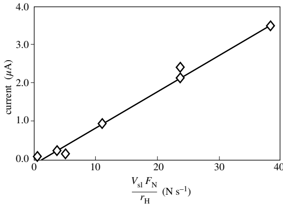
Figure 10.24 Average current measured during rubbing of Ti6Al4V alloy against an aluminium oxide ball plotted against the parameter v_{sl}F_N/r_H . Electrolyte: 0.9 w% NaCl. Applied potential: 0.5 V vs. Ag/AgCl [13].
