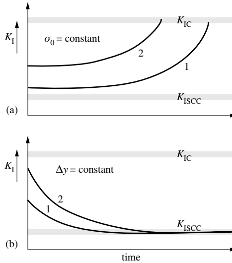
Figure 11.15 Variation of stress intensity at crack tip as a function of the testing time: (a) constant load; and (b) constant deformation. The labels 1 and 2 refer to two tests that differ by the magnitude of the applied load or deformation.
