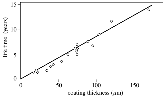
Figure 12.14 Lifetimes of zinc coatings on steel exposed to a polluted atmosphere as a function of their thickness [8].
