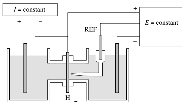
Figure 11.30 Two-compartment electrochemical cell used for the measurement of the hydrogen permeability of metals (schematic).
