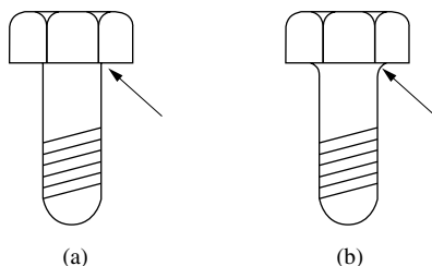
Figure 12.2 Reduction of the risk of stress corrosion cracking of a bolt: (a) high local stress; and (b) reduced local stress.
