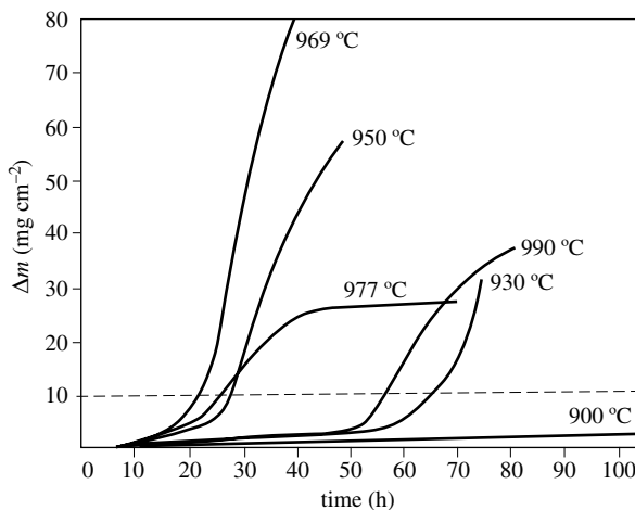
Figure 9.38 Effect of temperature on initiation time for hot corrosion of a Ni-Cr alloy (IN-738). P O 2 = 1 bar, 1 mg cm -2 Na 2 SO 4 [22].
