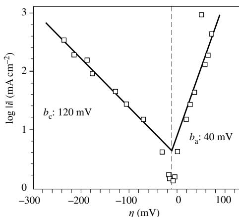
Figure 5.1 Polarization curve of copper in 0.5 M H 2 SO 4 + 0.075 M CuSO 4 .
