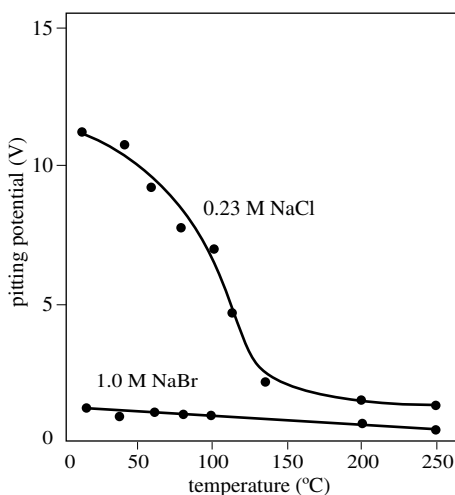
Figure 12.12 Pitting potential of titanium in 0.53 M NaCl and in 1 M NaBr as a function of the temperature [7].
