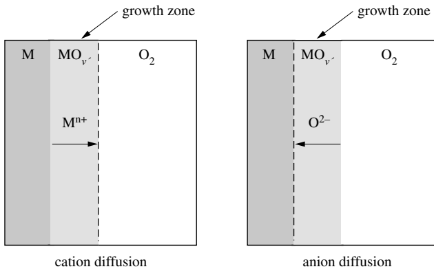
Figure 9.10 Oxide-layer growth by diffusion of cations or anions.
