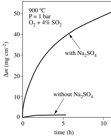
Figure 9.37 Effect of Na 2 SO 4 on the rate of nickel oxidation at 900 °C, O 2 + 4% SO 2 , P = 1 bar [21].
