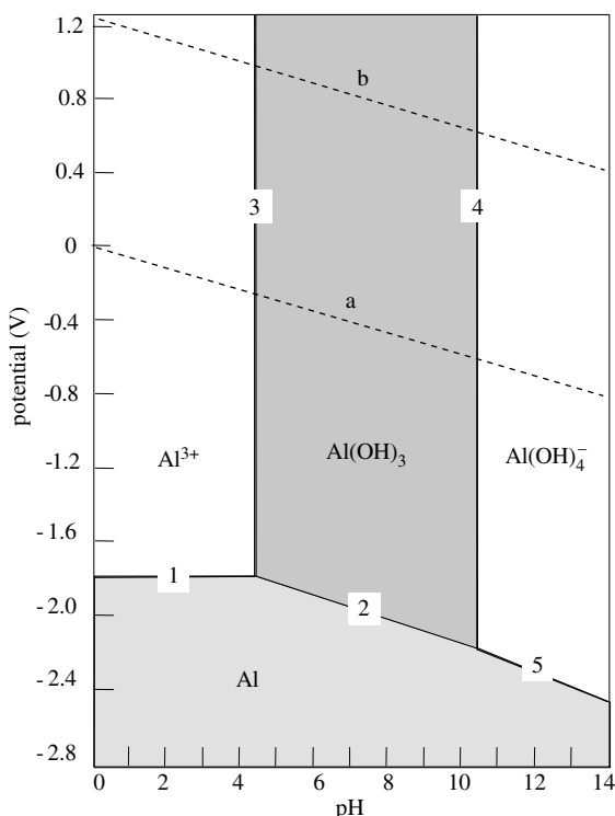
Figure 2.18 Potential-pH diagram for aluminum ( T = 25^\circ\text{C} ). The concentration of the dissolved ionic species, \text{Al}^{3+} and \text{Al(OH)}_4^- are equal to 10^{-6} \text{ mol l}^{-1} . The numbers refer to the reactions given in Table 2.17.
