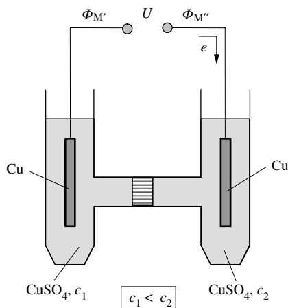
Figure 2.25 A concentration cell.
