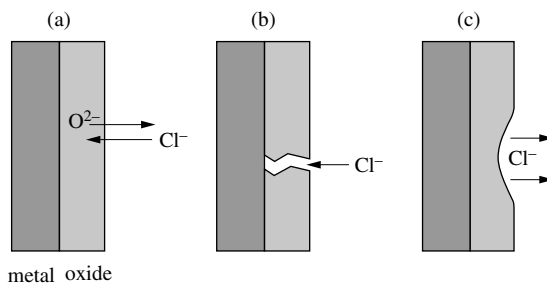
Figure 6.40 Proposed anodic depassivation mechanisms in presence of chloride: (a) anion penetration into the film by exchange with \text{O}^{2-} ; (b) electrolyte penetration at the metal surface through film defects; (c) film dissolution caused by local anion adsorption.
