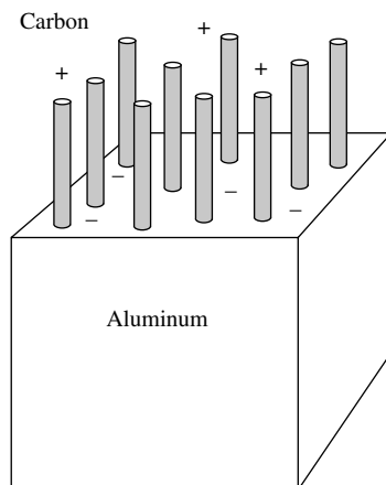
Figure 7.25 Corrosion cell formed between graphite fibers and an aluminum matrix (schematic).
