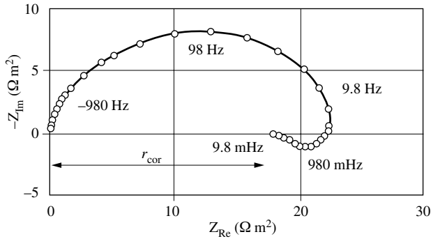
Figure 5.31 Nyquist diagram of the impedance of an iron electrode in deaerated 0.5 M \text{H}_2\text{SO}_4 [13].
