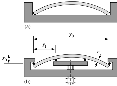
Figure 11.7 Bending tests for stress corrosion cracking.
