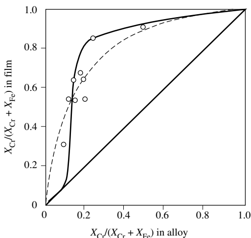
Figure 6.20 Average chromium content of passive film of Fe-Cr alloys, measured with XPS, as a function of Cr concentration in the alloy. Solution is 0.5M \text{H}_2\text{SO}_4 . The dashed curve is calculated using equation (6.13) [13,15].
