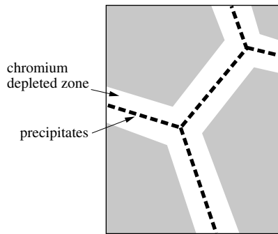
Figure 7.39 Chromium depletion at grain boundaries due to the precipitation of chromium carbides (schematic).
