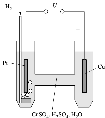
Figure 2.7 The \text{H}_2 / \text{Cu} electrochemical cell.
