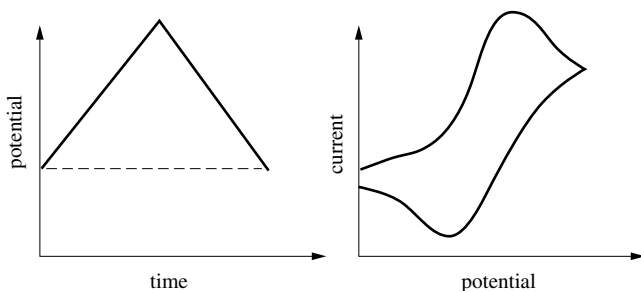
Figure 5.17 Cyclic voltammogram.
