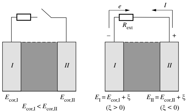
Figure 7.2 Corrosion cell due to contact of two different metals: (a) open circuit and (b) closed circuit configurations. R_{\text{ext}} corresponds to the external resistance.
