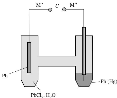
Figure 2.23 The lead/ lead amalgam cell.
