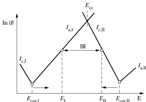
Figure 7.3 Evans diagram of a corrosion cell.
