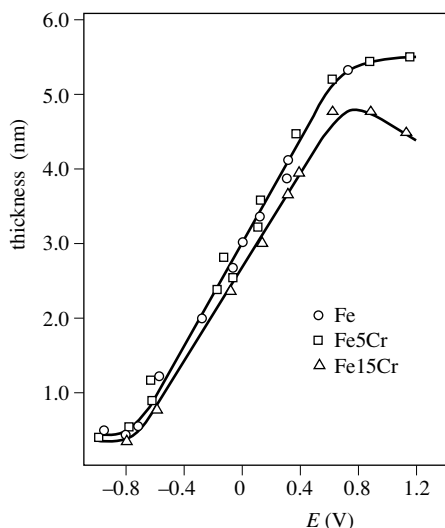
Figure 6.26 XPS film thickness on Fe and Fe-Cr alloys at different potentials [24].
