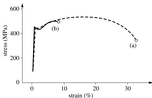
Figure 11.19 Stress-strain curve of cold rolled steel with and without hydrogen embrittlement: (a) stress-strain curve measured in air with a strain rate of 10^{-3} \text{ mm s}^{-1} ; (b) stress-strain curve measured in seawater in the presence of \text{H}_2\text{S} at a strain rate of 10^{-4} \text{ mm s}^{-1} .
