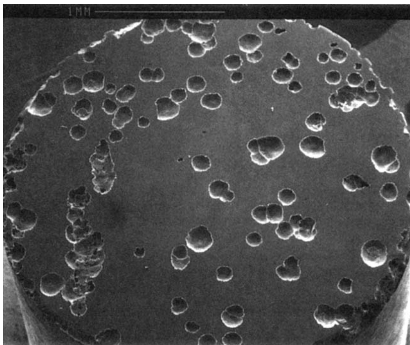
Figure 6.38 Surface pitting of an Fe-24Cr alloy resulting from anodic polarization in 1M HCl above the pitting potential.
