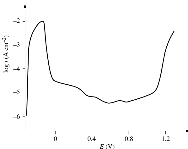
Figure 6.2 Polarization curve of Fe-17Cr stainless steel in 0.5 \text{ M H}_2\text{SO}_4 . Sweep rate is 0.02 \text{ V/min} . [1].
