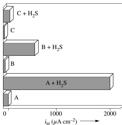
Figure 11.31 Hydrogen permeation through a Fe membrane in the presence and absence of \text{H}_2\text{S} as measured in a two-compartment cell. Electrolytes are (A) 4.7 M \text{HCl} ; (B) 2.5 M \text{H}_2\text{SO}_4 ; (C) 2.4 M formic acid + 200 \text{mg l}^{-1} of \text{Cl}^- [13].
