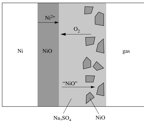
Figure 9.40 Mechanism of hot corrosion of Ni involving fluxing of oxides in molten sodium sulfate.
