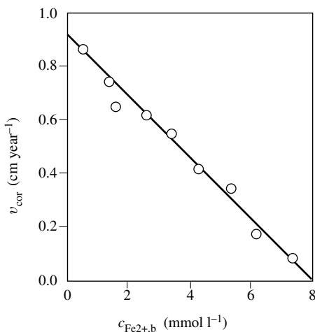
Figure 4.48 Corrosion controlled by mass transport of anodic reaction products: corrosion rate of steel in 68% H_2SO_4 at 60 °C as a function of Fe^{2+} bulk concentration. The rotation rate is 900 rpm, and the cylinder diameter is 1.9 cm [20].
