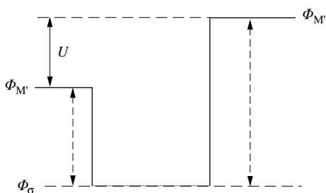
Figure 2.6 Levels of electric potential in an electrochemical cell without a liquid junction.
