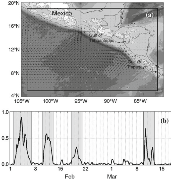
Fig. 1 (a) Map of the numerical model domain. Black arrows correspond to temporal wind average from February 1 to March 18, 2005. The time series of the magnitude of the wind stress in 95°W and 15°N are shown in (b), which corresponds to the maximum wind variability. We can identify four periods with strong wind ( shaded in gray ). The units are [N m -2 ]
