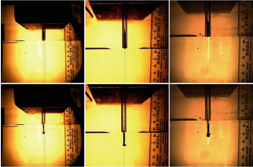
Fig. 5 In these pictures are shown the initial ( upper ) and final shapes ( lower ) of different mercury jets impinging on water at 10°C temperature. The details of each jet are the next: from left to right , 2 cm (Fr: 94.19, We: 192.73 and Re: 33,148), 2.5 cm (Fr: 111.75, We: 228.67, and Re: 36 106) and 3 cm (Fr: 106, We: 216.7 and Re: 35,150)
