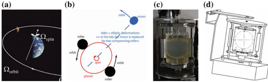
Fig. 1 Experimental set-up. The picture in (a) highlights the existence of two different rotation rates: the spin rate of the studied planet, and the orbital rate of the body responsible for the tidal deformation. As shown in the equatorial cross-section (b), this companion body is replaced in our set-up by two symmetric rollers. c and d show the experimental set-up
