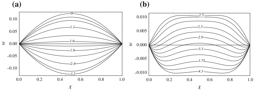
Fig. 3 Hydrodynamic velocity profiles for half of a period a R\omega = 1 , b R\omega = 100 . Labels indicate dimensionless temporal evolution, t .
