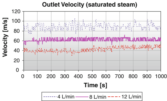
Fig. 4 Outlet steam velocity
