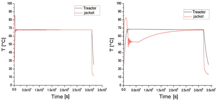
Fig. 3 Reactor and jacket temperatures as a function of time for rpm = 50. Reactor size 100 L (left) and 1,000 L (right)
