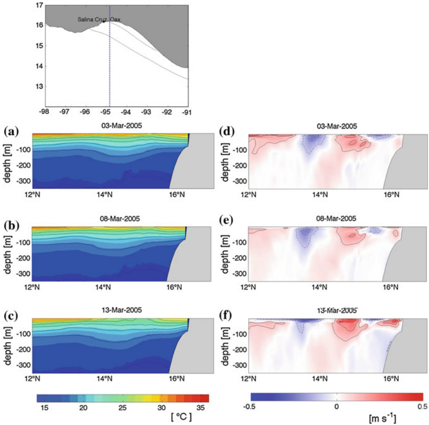
Fig. 7 Meridional section along 95.0°W of temperature (a–c) zonal component of velocity (d–f)
