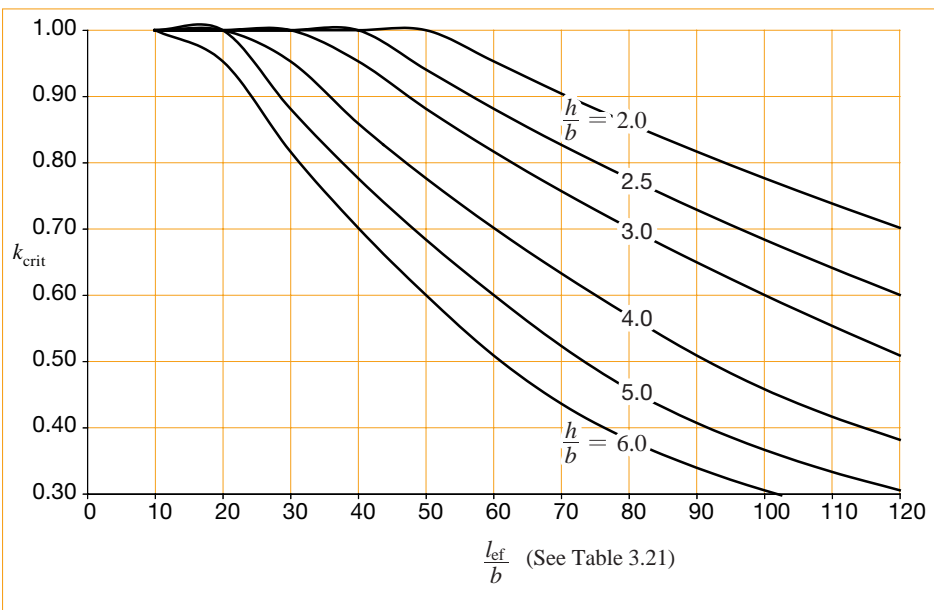
Fig 3.3 Values of k_{crit} for solid hardwood strength classes D30 to D70 (derived from EC5 6.3.3(4))
