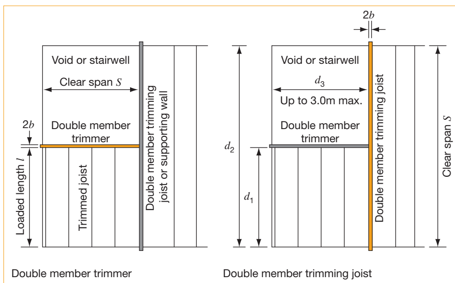
Fig 8.1 Plan showing dimensions for a trimmer and a trimming joist
