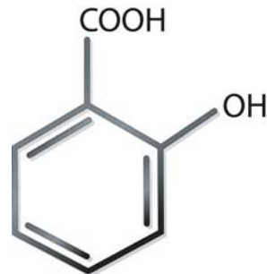
Fig. 6.1. Chemical structure
