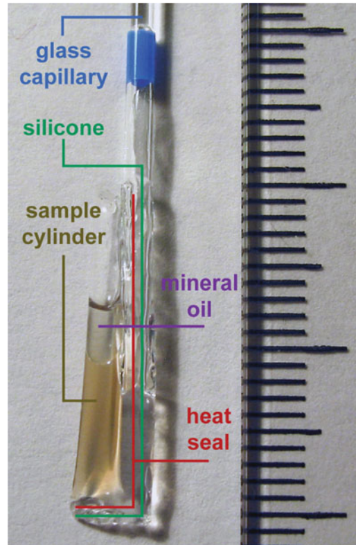
Fig. 3. Sample preparation of egg extracts in transparent plastic cylinders. The photo shows a polytetrafluorethylen (PTFE) cylinder loaded with Xenopus laevis egg extract. The cylinder is formed using a 25- \mu m-thin transparent plastic foil. The bottom part and lateral part of the plastic cylinder are sealed by welding using hot air. The seams are reinforced by transparent silicone glue. The heat seals prevent contact of the silicone glue with the specimen inside the plastic cylinder. A glass capillary is glued to the cylinder with transparent silicone glue and acts as a sample holder in the light sheet microscope. A layer of mineral oil is added on top of the egg extract to prevent degradation by exposure to air. Scale: major tick mark spacing = 10 mm, minor tick mark spacing = 1 mm.
