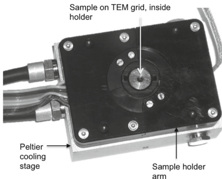
Fig. 11. Image of the packaged FEI Wet STEM detector assembled and with a TEM grid inside.
