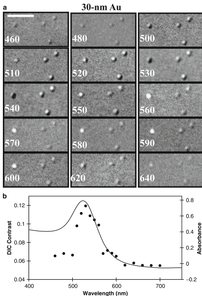
Fig. 5. Typical DIC spectrum of 30-nm gold nanoparticles. (a) Wavelength-dependent DIC images of gold nanoparticles immobilized on glass substrate. (b) Plots of the calculated DIC contrast ( dots ) of single nanoparticles and the UV-VIS absorption ( curve ) of the bulk gold nanoparticle solution vs. the illumination wavelength. Scale bar represents 1 \mu\text{m} .
