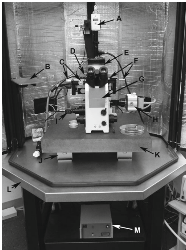
Fig. 2. MFP-3D-BIO AFM setup as configured in our laboratory for macromolecular and cell biology applications includes (a) Top View camera for probe viewing and alignment; (b) MFP-3D-BIO stainless steel platform for mounting cantilever holder on head; (c) optical ( x,y ) alignment controls which move the entire base plate to translate the cantilever and specimen to field of view with bottom view cameras via objectives; (d) x,y scanner; (e) MFP-3D-BIO Head; (f) sample ( x,y ) alignment controls which move the sample relative to the cantilever; (g) IX71 Olympus inverted optical microscope; (h) Hamamatsu video camera for highest resolution viewing and recording; (i) Composite camera for lower resolution viewing and image capture; (j) isolation module ( \times 2 ); (k) granite slab; (l) TMC BCH-45 acoustic enclosure platform; and (m) vibration isolation electronics controller. The ARC2 with Hamster, Fiber-Lite, Hamamatsu, X-cite, and heater controllers are not shown.
