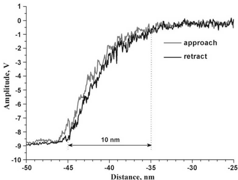
Fig. 6. Amplitude-distance curve acquired in buffer on a glass slide with an MAC Lever. Trace ( light grey line ) and retract ( black line ) are collected using the same cantilever as in Fig. 2.
