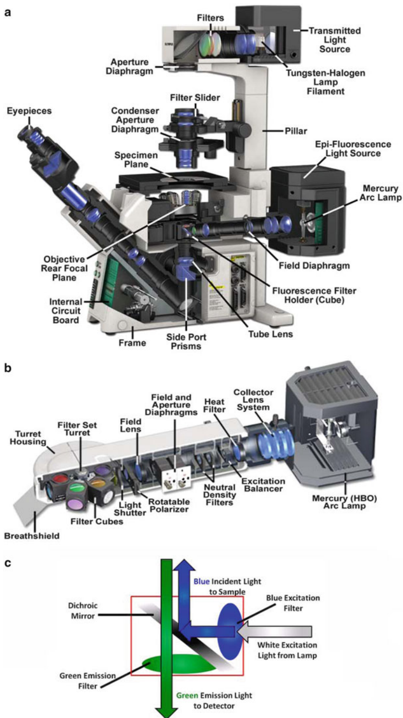
Fig. 1. (a) Cut through of an Olympus IX81 fully motorized epi-fluorescence microscope showing details of the fluorescence light path. (b) Detailed view of the epi-illumination arm for the IX81 microscope showing components of the fluorescence light path. Images (a, b) are courtesy of Michael Davidson, Florida State University, National High Magnetic Field Laboratory, Tallahassee, FL. (c) Schematic of a fluorescence cube for EGFP imaging. Blue light is selected from the white incident light from the lamp using a blue band pass excitation filter. The blue light reflects off the dichroic mirror and is directed upwards to the objective lens then focused on the sample. Green emission light from the sample passes through the dichroic mirror and through a green band pass emission filter to the detector. The emission filter also reduces image background by rejecting any reflected blue incident light.
