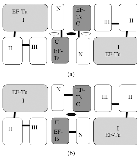
Fig. 9.16 The interaction between EF-Tu and EF-Ts in the crystal structures of (a) E. coli (Kawashima et al. , 1996) and (b) T. thermophilus . In both cases the N-terminal region (N) interacts with the G-domain of EF-Tu and the C-terminal region (C) interacts with domain III of EF-Tu (Wang et al. , 1997). The structures of EF-Ts that interact with EF-Tu are related, even though they belong to one molecule in the case of E. coli and to two molecules in the case of T. thermophilus . The filled symbol between the subunits signifies a molecular twofold axis, and the open symbol represents a local pseudo-twofold symmetry axis.
