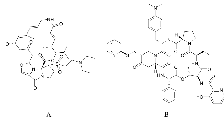
Fig. 10.11 Dalfopristin and quinupristin are streptogramins of types A and B, respectively (drawn by Andreas Ehnbohm).
