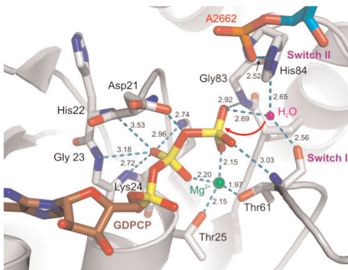
Plate 9.11 A GTP molecule placed as the GDPCP molecule in EF-Tu, when bound to the ribosome (Voorhees et al. , 2010). In this conformation the water molecule donates hydrogen bonds to the carbonyl oxygen of Thr61 in switch I and to the \gamma -phosphate of GTP. The water molecule has therefore exhausted its potential to act as a donor of hydrogen bonds. The phosphate of A2662 in the SRL of the 23S RNA accepts a hydrogen bond from His84 of switch II and positions it next to the water molecule at the \gamma -phosphate. His84, which is in a negatively charged environment, must then be protonated to be able to hydrogen-bond to the water molecule. The histidine therefore does not activate the water molecule but positions it at the \gamma -phosphate to donate a proton to it in association with the in-line attack. (Reprinted with permission from Liljas et al. , (comments on ‘The mechanism for activation of GTP hydrolysis on the ribosome,’ Science 333 : 37. Copyright 2011, AAAS.)
