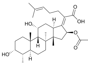
Fig. 10.14 Fusidic acid (drawn by Andreas Ehnbohm).
