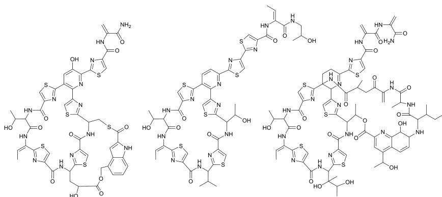
Fig. 10.13 The chemical formulae of nosiheptide, micrococcin and thiostrepton, which prevent EF-G from binding properly to the ribosome (drawn by Andreas Ehnbohm).
