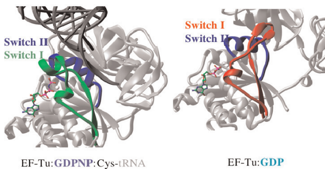
Plate 9.9 Left: The conformation of switches I and II in EF-Tu in the GTP conformation. Right: The conformation of switches I and II in EF-Tu in the GDP conformation. (Illustration kindly provided by M. Laurberg.)
