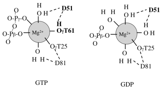
Fig. 9.7 The coordination around the magnesium ion in the GTP and GDP states of EF-Tu. The \gamma - and \beta -phosphates of the nucleotide bind to the magnesium ion. Thr25 of the \text{PO}_4 loop is a constant ligand to the magnesium ion, and Asp51 of switch I and Asp81 of switch II always interact with the magnesium ligands. Thr61 of switch I binds to the magnesium only in the GTP state.
