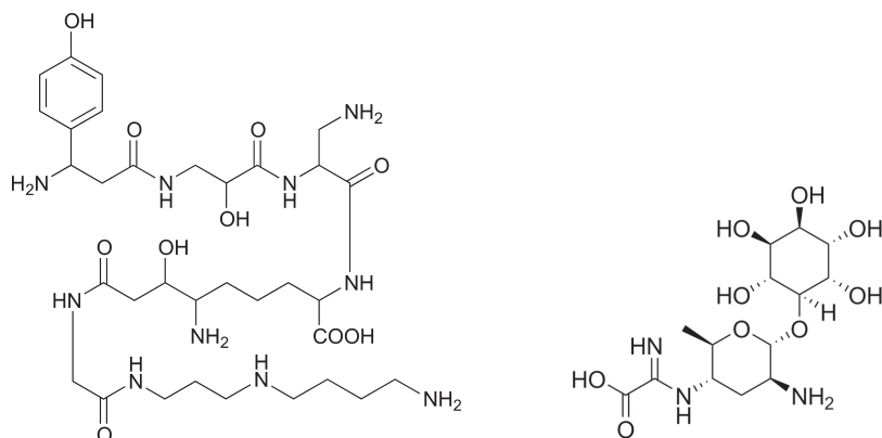
Fig. 10.2 Left: Edeine (drawn by Andreas Ehnborn). Right: Kasugamycin (from Wikipedia).
