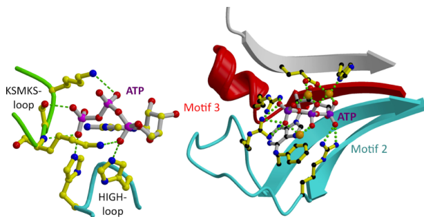
Plate 5.3 The binding of ATP to tRNA synthetases. Left: TyrRS (class Ic) with conserved residues of the KMSKS loop (green) and HIGH loop (blue) interacting with the ATP. Right: ProRS (class IIa). Residues of motifs 2 (blue) and 3 (red) interact with the ATP. The brown bolls represent magnesium ions. (Courtesy of Stephen Cusack.)
