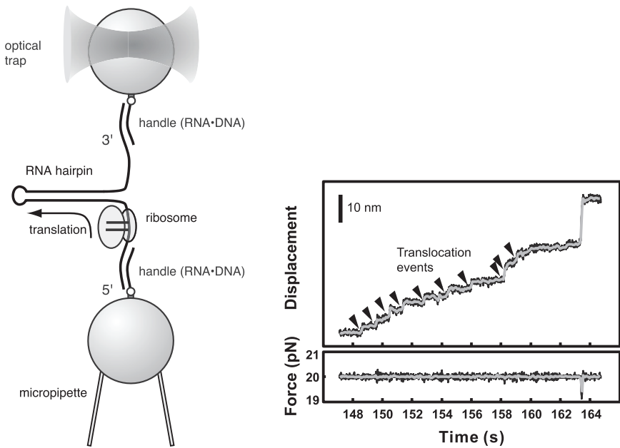
Fig. 3.1 Force measurements performed on a translating ribosome. Left: One end (the upstream end of the mRNA) is immobilized with a micropipette while the optical trap pulls on the other end (the downstream end of the mRNA). Right: When the ribosome translocates, the loop of the mRNA melts and the distance between the two ends increases. (Reproduced with permission from Aitken et al. , Single ribosome dynamics and the mechanism of translation, Annu Rev Biophys 39:491–513. Copyright 2010, Annual Reviews Inc.)
