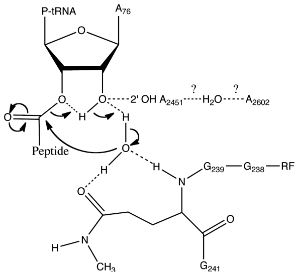
Fig. 11.11 The possible interactions in the PTC during peptide hydrolysis. (Reprinted with permission from Jin et al. , Structure of the 70S ribosome bound to release factor 2 and a substrate analog provides insight into catalysis of peptide release. Proc. Natl. Acad. Sci. USA 107 : 8593–8598. Copyright 2010, National Academy of Sciences.)
