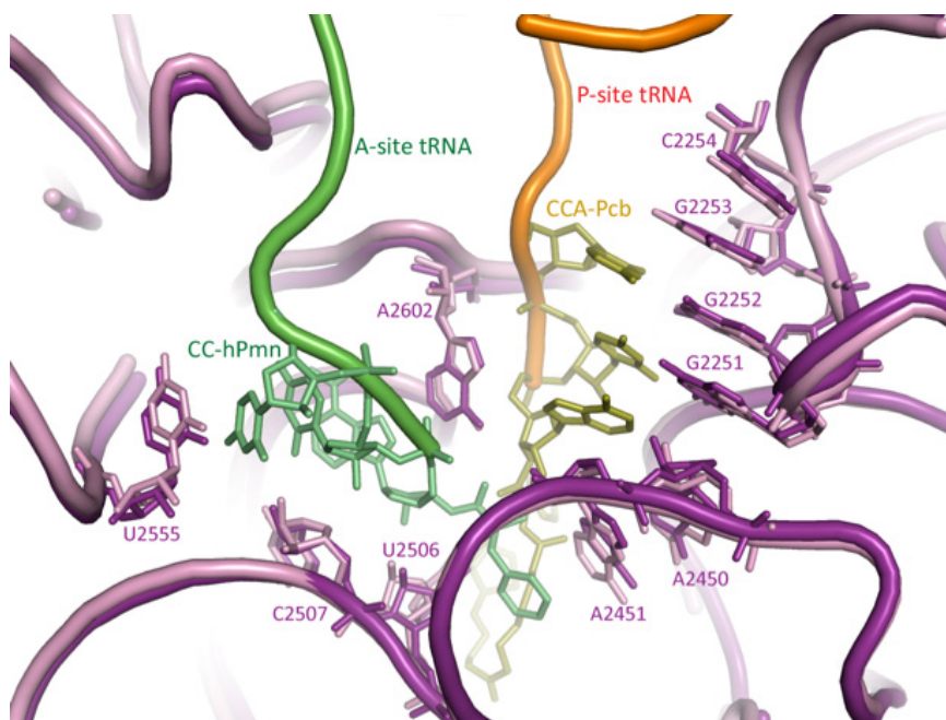
Plate 8.8 The structure of the PTC from Hm 50S subunits and from Tt 70S ribosomes are very similar (Voorhees et al. , 2009). (Drawing by Saraboji Kadhivrel.)
