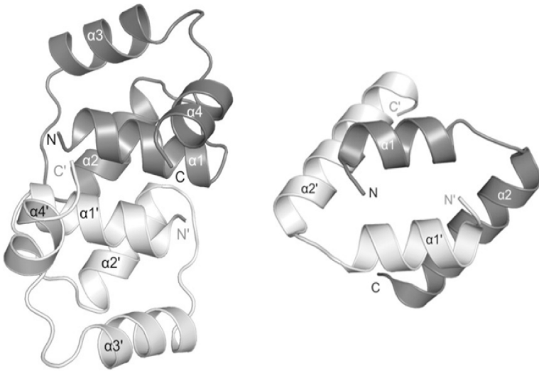
Fig. 7.7 The structure of the N-terminal part of a dimer of the archaeal protein P1/2 compared to bacterial L12. One monomer in white and the second one in gray. We are in both cases looking down the twofold axis of the dimer. Apart from the helical structure, it is difficult to identify a structural similarity. (Illustration by Saraboji Kadhivel.)
