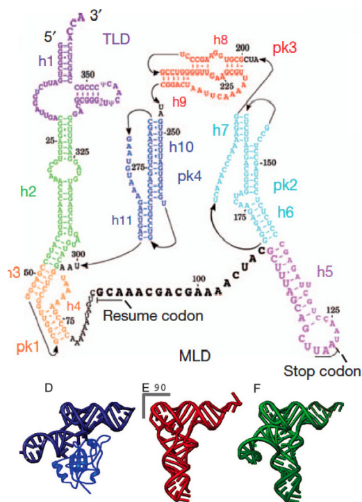
Plate 9.18 Top: The secondary structure of tmRNA. (Reprinted with permission from Ramrath et al. , The complex of tmRNA–SmpB and EF-G on translocating ribosomes, Nature 485 : 526–530. Copyright 2012, Nature.) Bottom: The structure of the TLD of tmRNA together with SmpB compared with a normal tRNA and a tRNA with a long variable arm. (Reprinted with permission from Bessho et al. , Structural basis for functional mimicry of long-variable-arm tRNA by transfer-messenger RNA, Proc Natl Acad Sci USA 104 : 8293–8298. Copyright 2007, The National Academy of Sciences of the USA.)
