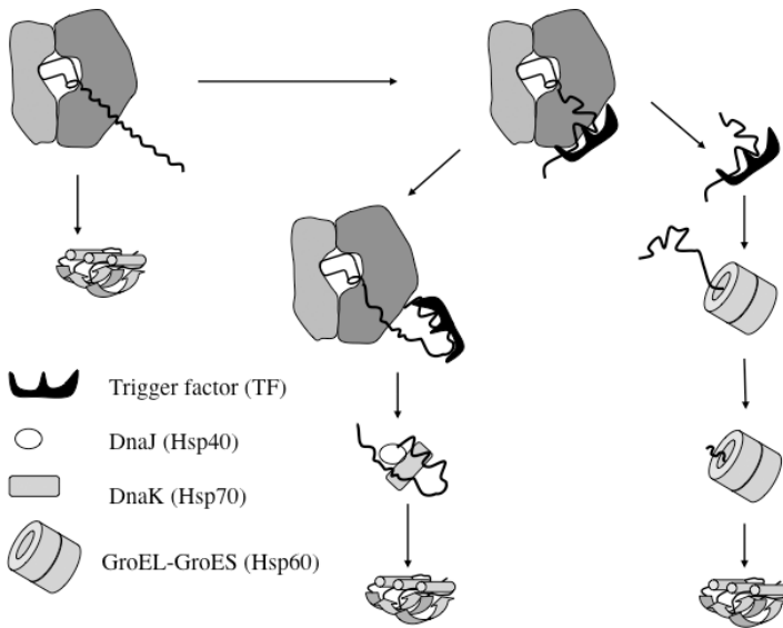
Fig. 12.1 Different folding pathways of the NC. The polypeptide may fold spontaneously, after interaction with trigger factor or after ATP-dependent folding assisted by chaperones DnaK/DnaJ (Hsp70/Hsp40) or GroEL/GroES.
