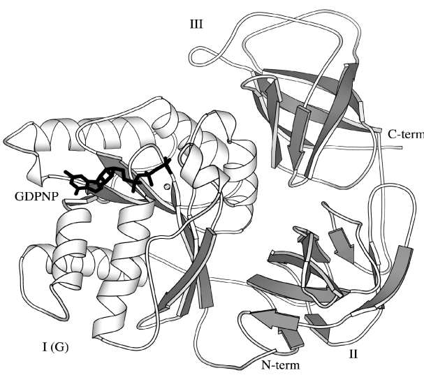
Fig. 9.2 The structure of EF-Tu, the first G-protein to be characterized (Kjeldgaard et al. , 1993). The domains are denoted I (the G-domain), II and III. In its complex with a GTP analog like GDPNP, it adopts a closed conformation. A magnesium ion is seen as a small gray circle between the \beta - and \gamma -phosphates. (Figure kindly provided by Dr. M. Fodje.)
