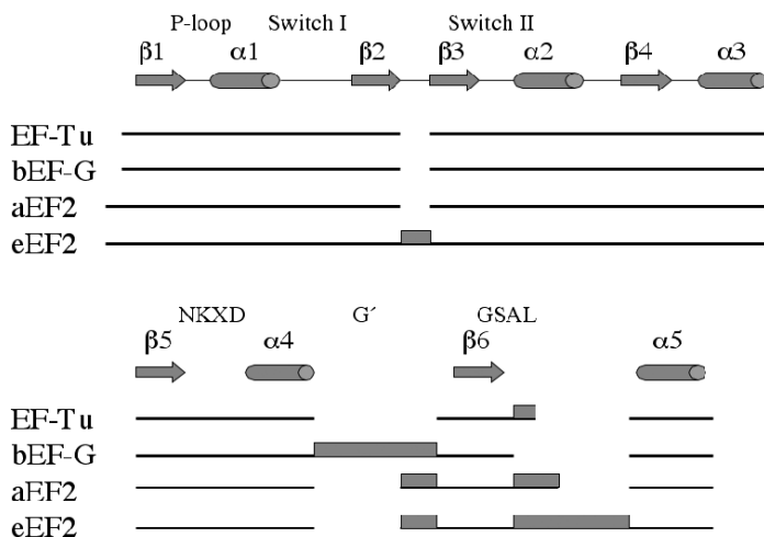
Fig. 9.21 Different inserts into domain I of EF-G and EF2 from bacteria, archaea and eukaryotes compared to EF-Tu. While bacterial EF-G has a long insert called G' before \beta -strand 6, eukaryal EF2 has a short insert here and a longer one after \beta 6 . Archaeal EF2 has short inserts in both places (Ævarsson, 1995).
