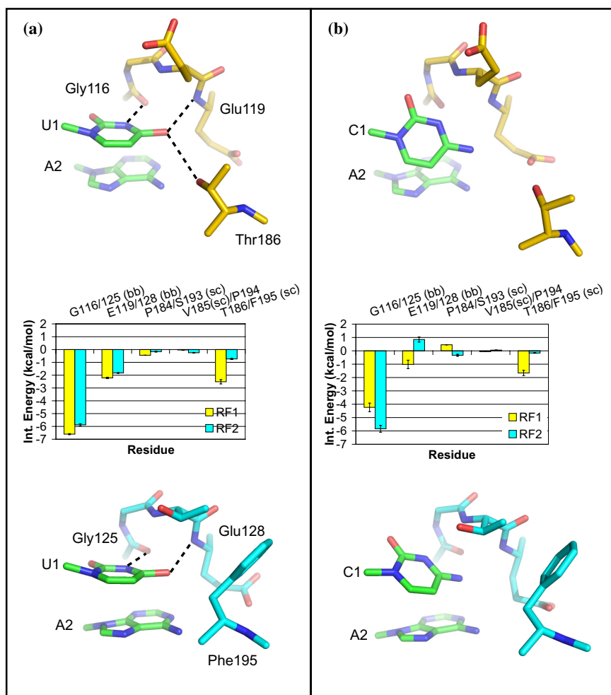
Plate 11.3 Reading of the first position of a stop codon. U is recognized (a) and C is discriminated against (b) by RF1 (yellow, top) and RF2 (cyan, bottom). Hydrogen bonds are indicated by dashed lines. The interaction energies between release factor residues (sidechains sc; backbone bb) and the base in the first codon position. (Reprinted with permission from Sund et al. , Principles of stop-codon reading on the ribosome. Nature 465 : 947–951. Copyright 2010, Nature Publishing Group.)
