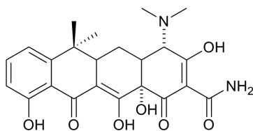
Fig. 10.3 Tetracycline (drawn by Andreas Ehnobom).
