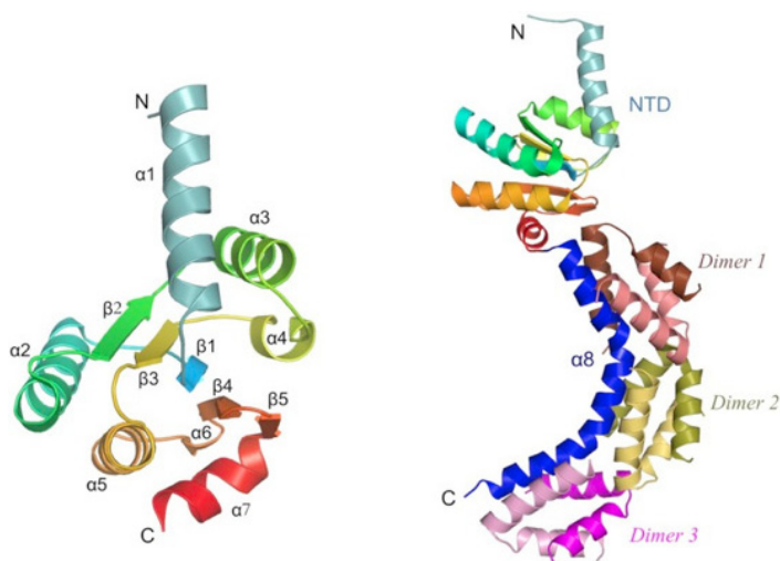
Plate 7.3 Left: The structure of the globular part of L10 from T. maritima (Diakonou et al. , 2005). Right: The L10 structure including the C-terminal \alpha helix ( \alpha 8 ) to which three dimers of L12 bind. (Illustration by Saraboji Kadhivrel.)
