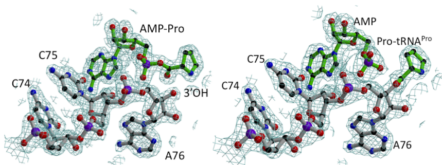
Plate 5.6 Crystal structures in the case of ProRS (class IIa). Left: The activated Pro residue is placed next to the CCA end of tRNA Pro . Right: The aminoacylation is complete and the Pro residue is attached to the 3' end of the tRNA, with the resulting AMP molecule still attached. (Courtesy of S. Cusack.)
