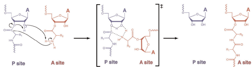
Plate 11.2 The possible mechanism of peptide transfer by the ribosome. The acceptor ends of the tRNAs in the P site (left) and A site (right). The 2'OH of A76 of the P site tRNA hydrogen-bonds to the \alpha -amino group of the aminoacyl residue bound to the A-site tRNA and extracts a proton from the amino group to enable it to form a tetrahedral intermediate with the carbonyl carbon between the nascent polypeptide and the P site tRNA. After peptidyl transfer the peptide is bound to the A site tRNA and the proton transfer is completed with both the 2' and 3' OHs of A76 in the P site being protonated. (Reprinted with permission from Simonovic & Steitz, A structural view on the mechanism of the ribosome-catalyzed peptide bond formation, Biochim Biophys Acta 1789 : 612–623. Copyright 2009, Elsevier.)
