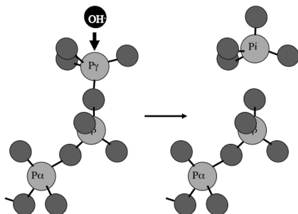
Fig. 9.8 GTP hydrolysis. An activated water molecule makes a linear attack on the \gamma -phosphate. Whether the reaction is associative, going over a pentavalent phosphor atom, or dissociative is debated (Wittinghofer, 2005).
