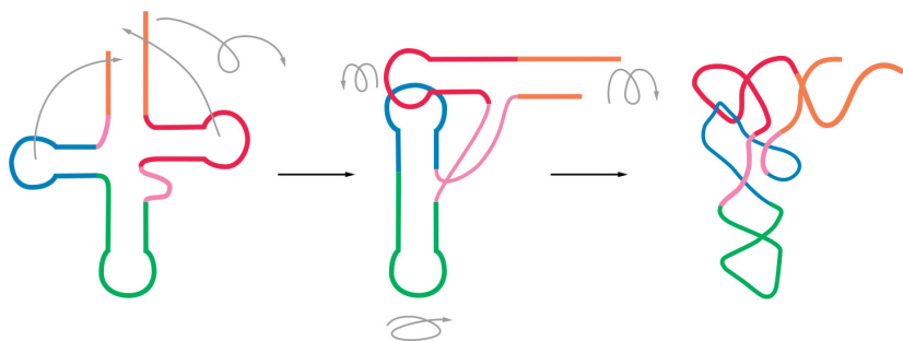
Plate 5.1 A schematic representation of the way the cloverleaf structure is organized in three dimensions. (Copied with permission from Liljas et al. , 2009, Textbook of Structural Biology .)
