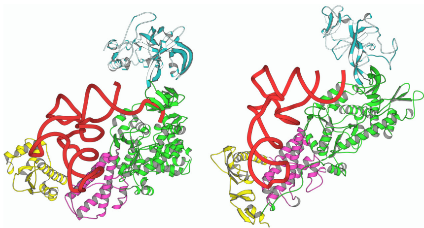
Plate 5.7 Left: LeuRS has no contact with the anticodon of the bound tRNA. However, the long variable loop (left part of the tRNA) is part of the tRNA recognition. The CCA end and the amino acid are in contact with the catalytic domain (green). The editing domain is in cyan. Right: IleRS with Ile-tRNA. The anticodon is recognized by the synthetase. Here the CCA end and the amino acid are close to the editing domain. (Courtesy of Lars Liljas.)
