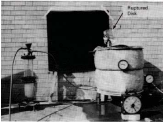
Figure 8c The remains of the ruptured disc at the top of the vessel leave no doubt that there was an explosion inside the vessel.
