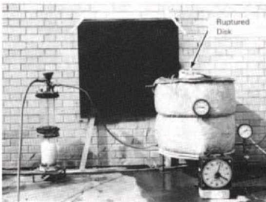
Figure 8b A spark plug in the vessel was energized in the interval between this and the previous picture. Note the ruptured disc on the top of the vessel failing due to the internal explosion.
