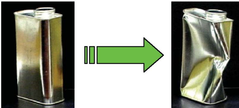
Figure 9b Result of condensation. This can was filled with steam and then closed. The steam condensed, and the resulting vacuum caused the damage shown.
