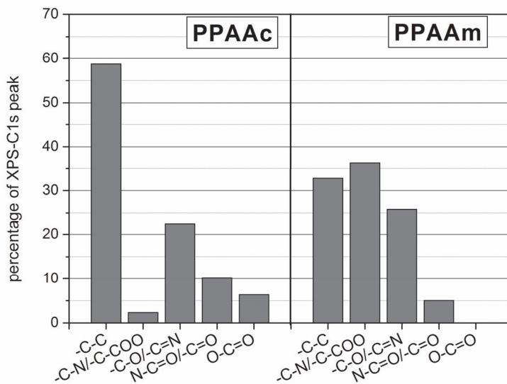
Fig. 13. Percentages of bonding components in C1s peak after film preparation on polished titanium for PPAAm (right) and PPAAc (left).
