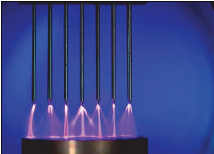
Fig. 3. b. View on a multi-tip pulsed corona discharge tested at LAPLACE-PRHE Laboratory.
