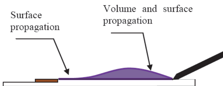
Fig. 5. c. Schematic cross section of the surface discharge in the case of PMMA insulator from (Gardou et al 2009).
