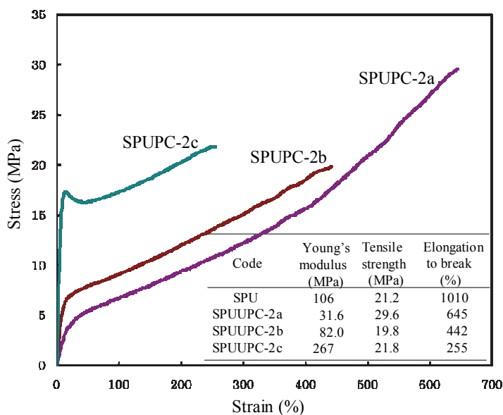
Fig. 6. Stress-strain behaviors of SPUPC films.
