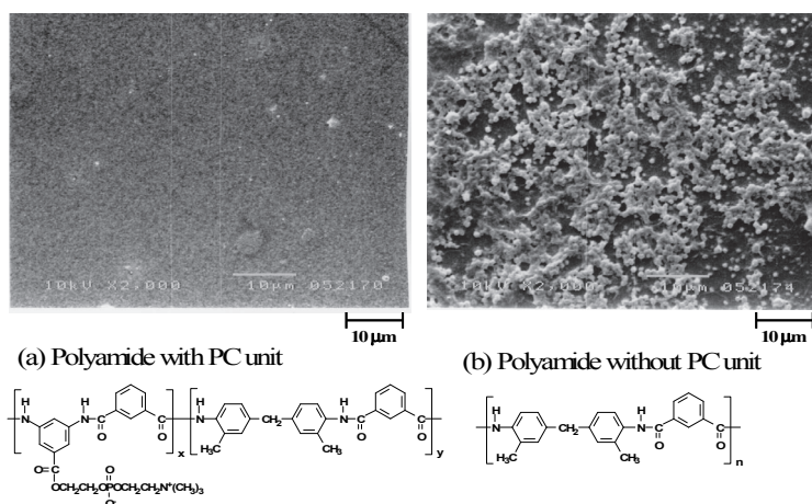
Fig. 1. SEM pictures of polyamide film surfaces with and without PC unit after contact with human PRP for 60 min at 37 °C. (x 2,000)
