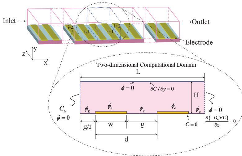
Fig. 1. Schematic view of DEP microfluidic device considered for manipulating the particles. Enlarged view shows the two-dimensional computational domain considered for analysis
