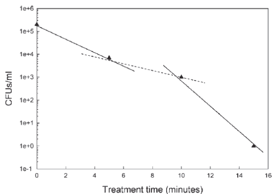
Fig. 4. Example of a three-phase survival curve: inactivation of Pseudomonas aeruginosa with an atmospheric pressure glow discharge in a helium/air mixture [Reprinted with permission from (Laroussi, 2005)].
