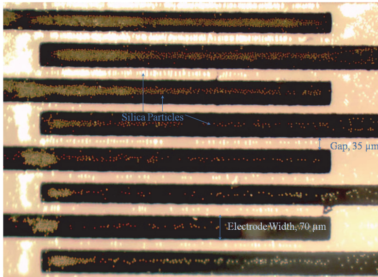
Fig. 13. Negative DEP effect on silica particles
