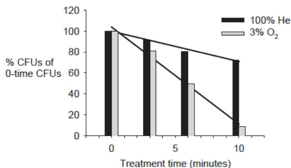
Fig. 5. Percent of surviving Bacillus spores as a function of plasma treatment time for pure helium (black) and a helium/oxygen mixture (97% He-3% O_2 ) [Reprinted with permission from (Laroussi&Leipold, 2004)].
