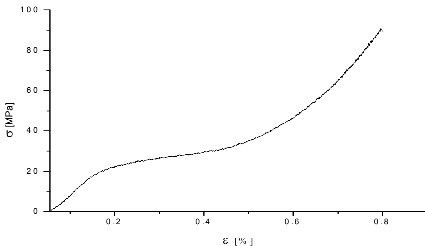
Fig. 12. Typical non-linear elastic behavior of HAp-based, organic-inorganic composites.
