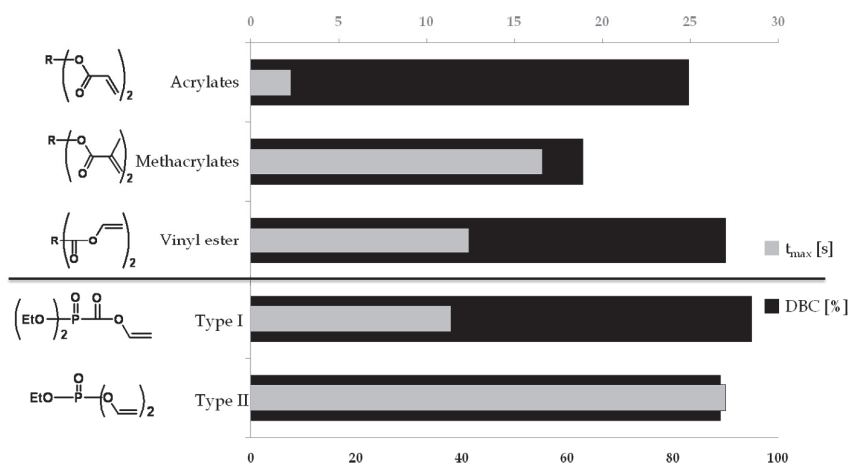
Fig. 4. Photo-Differential Scanning Calorimetry data for the phosphomonomers, Type I and II, as well as for reference acrylates and methacrylates
