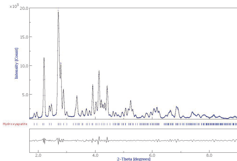
Fig. 5. Reitveld refinement of sum of all data with texture parameters
