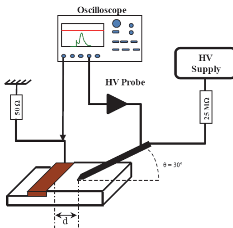
Fig. 5. a. Experimental setup of surface corona discharge with an inclination angle of 30^\circ between the anodic needle and the dielectric surface ( d being the gap separation between the tip of the needle and the cathode copper) from Merbahi et al 2011
