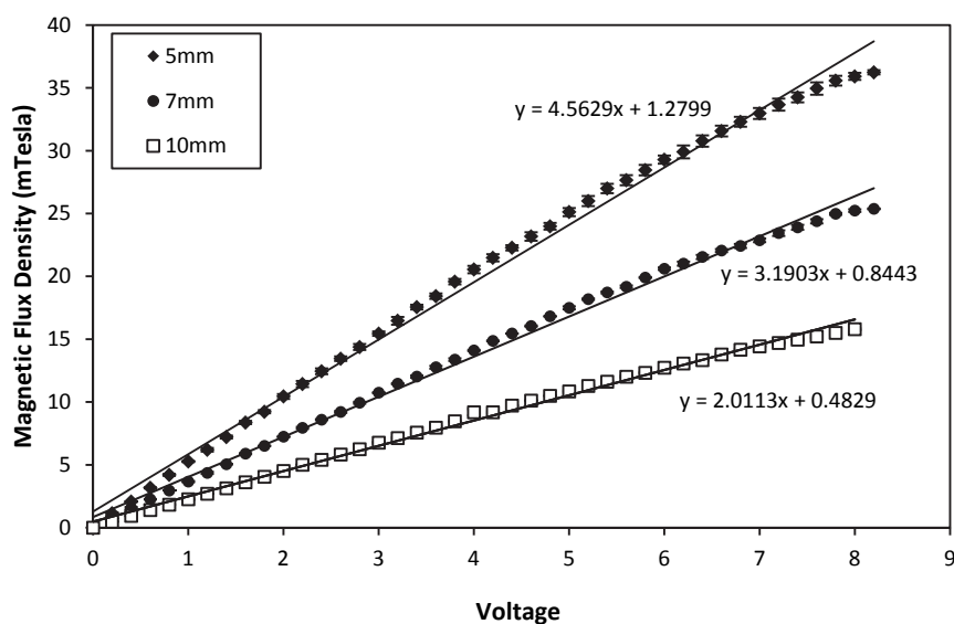
Fig. 3. Seawater calibration curve ( n = 3 , \pm standard error). Distances reported are MagPI probe from a sensor connected to a Gauss meter.
