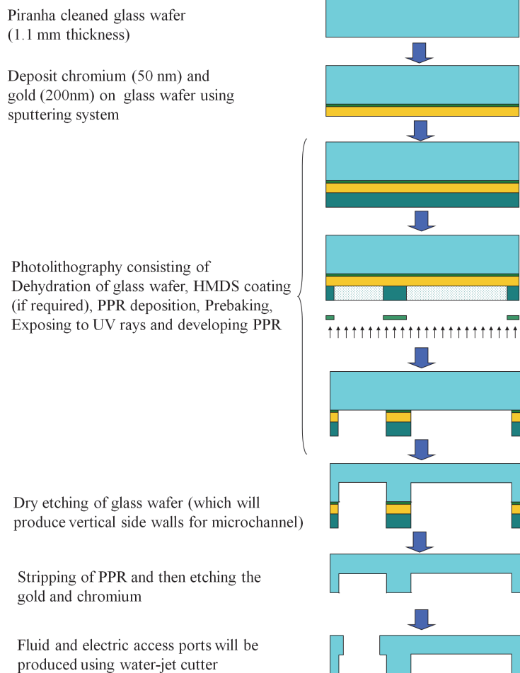
Fig. 9. Process flow for fabrication of microchannels
