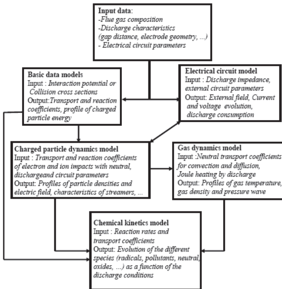
Fig. 8. Diagram showing the coupling between the different models which can be used to describe the electro-hydrodynamic and reaction kinetics phenomena and processes in the case of atmospheric pressure non thermal plasmas generated by corona or DBD discharges (Yousfi et al 2010)
