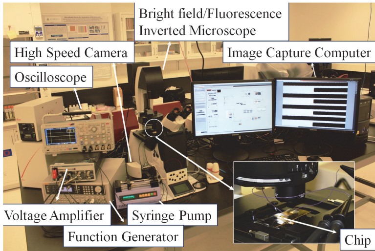
Fig. 11. Testing set-up for DEP experiments
