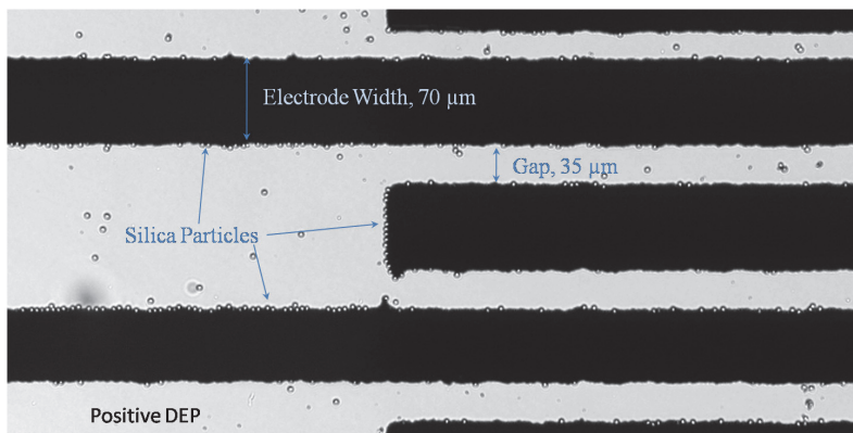
Fig. 12. Positive DEP effect on silica particles
