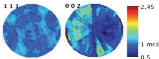
Fig. 9. Pole figures at 2,4 mm from the interface with the face uncoated
