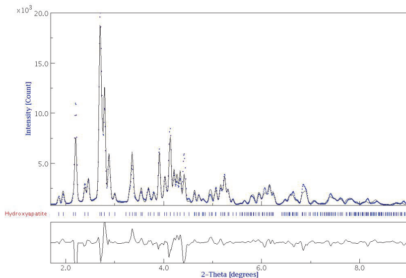
Fig. 4. Reitveld refinement of sum of all data
