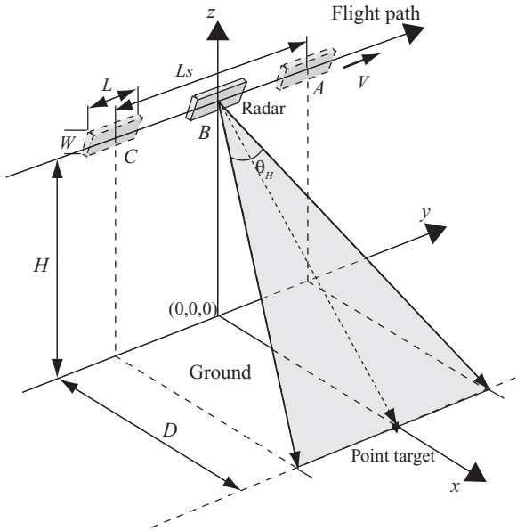
FIGURE 6.7 Configuration of a broadside SAR system.
