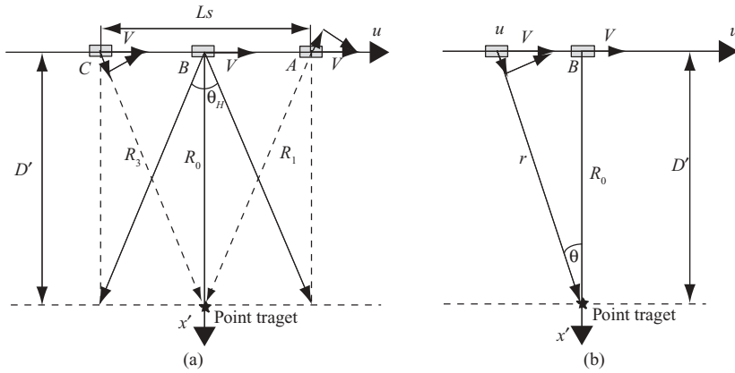
FIGURE 6.8 A simplified broadside SAR system.
