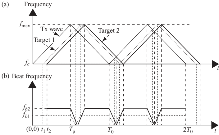
FIGURE 5.30 Time–frequency relationship of Tx and echo signals from two stationary targets.
