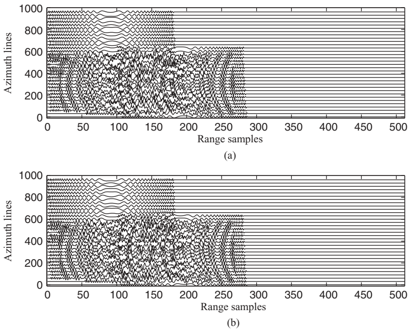
FIGURE 9.19 Waveforms of received signal from Fig. 9.16.
