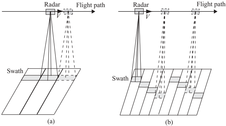
FIGURE 6.1 Configurations of (a) a stripmap SAR and (b) a scan SAR.
