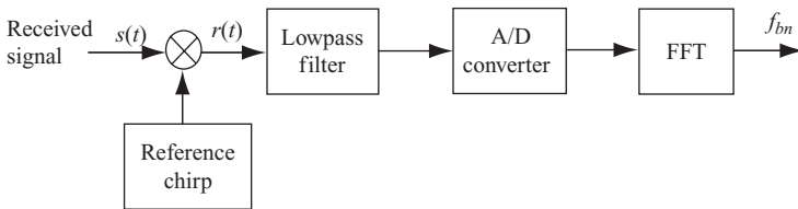
FIGURE 5.29 Block diagram of dechirp processing.
