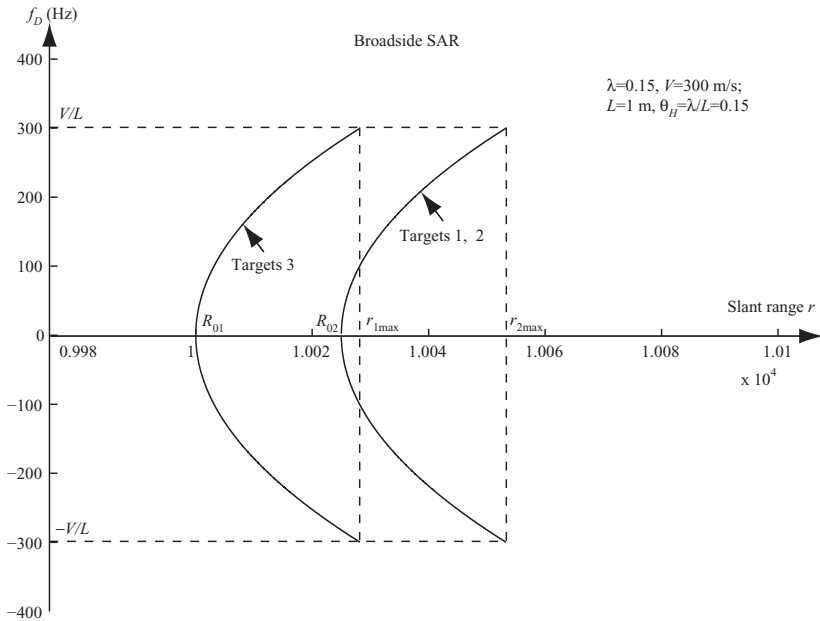
FIGURE 6.17 Doppler frequency versus slant range for multiple targets.
