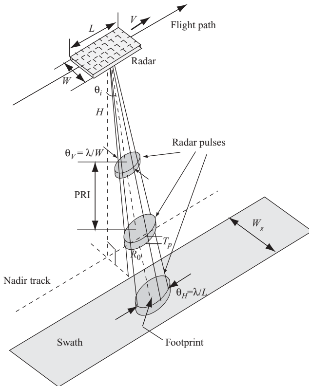
FIGURE 6.3 Geometry of stripmap imaging radar.
