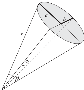
FIGURE 3.12 Antenna radiation pattern approximated as an elliptical area.
