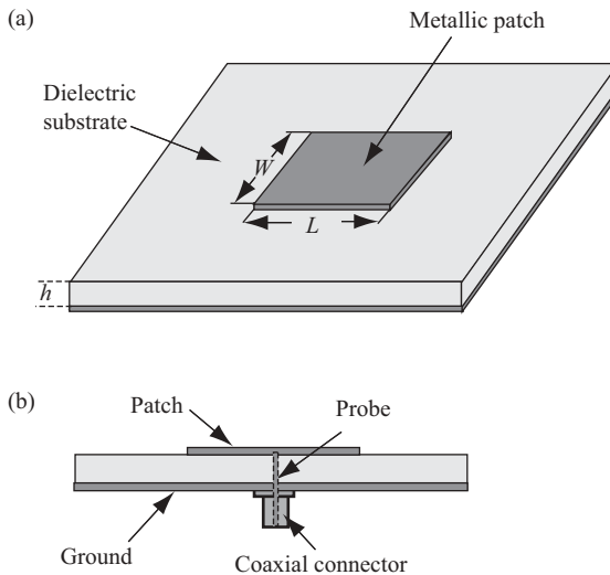
FIGURE 3.15 Printed patch antenna.
