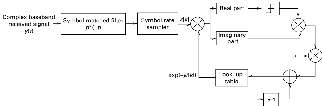
Figure 4.10 Discrete time decision-directed Costas loop for BPSK modulation.
