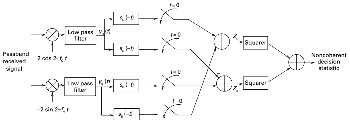
Figure 4.6 Computation of the noncoherent decision statistic for a complex baseband signal s . The optimal noncoherent receiver employs a bank of such processors, one for each of M signals, and picks the maximum of M noncoherent decision statistics.
