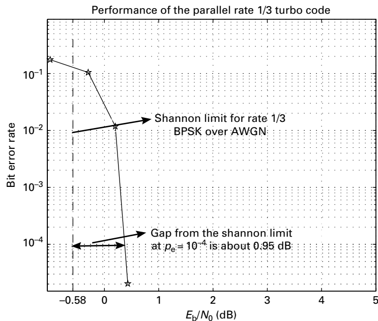
Figure 7.12 Bit error rate for a rate 1/3 parallel concatenated turbo code obtain by concatenating two identical rate 1/2 [7, 5] convolutional codes. The block length is 2^{14} \approx 16000 .
