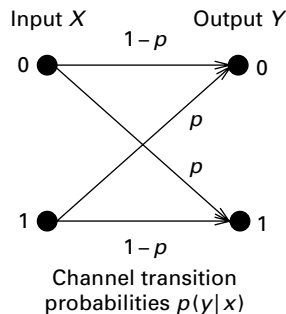
Figure 6.3 Binary symmetric channel with crossover probability p .
