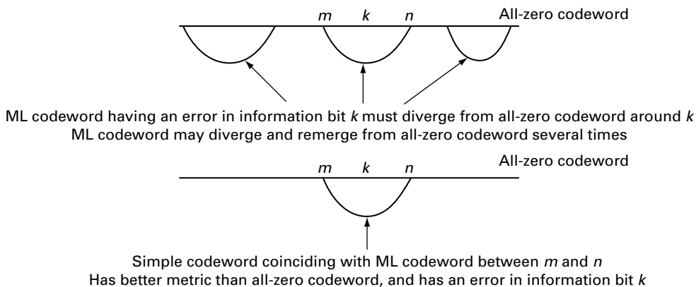
Figure 7.6 Transmitted all-zero codeword and ML codeword as paths on the trellis. In the scenario depicted, the input bit u[k] corresponding to the ML codeword is incorrect. I also show the simple codeword which coincides with the ML codeword where it diverges from the all-zero path around bit k , and coincides with the all-zero codeword elsewhere.
