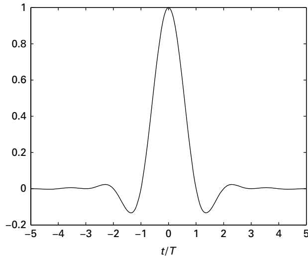
(b) Time domain pulse (excess bandwidth \alpha = 0.5 )
