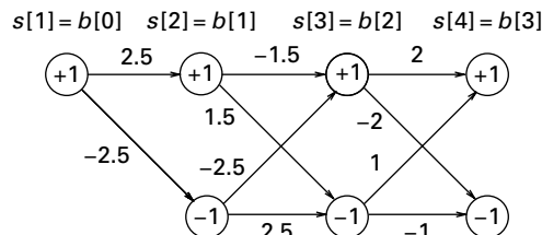
Figure 5.5 First few trellis branches for the running example.
