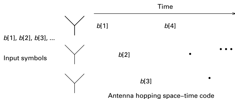
Figure 8.23 Antenna hopping space–time code.
