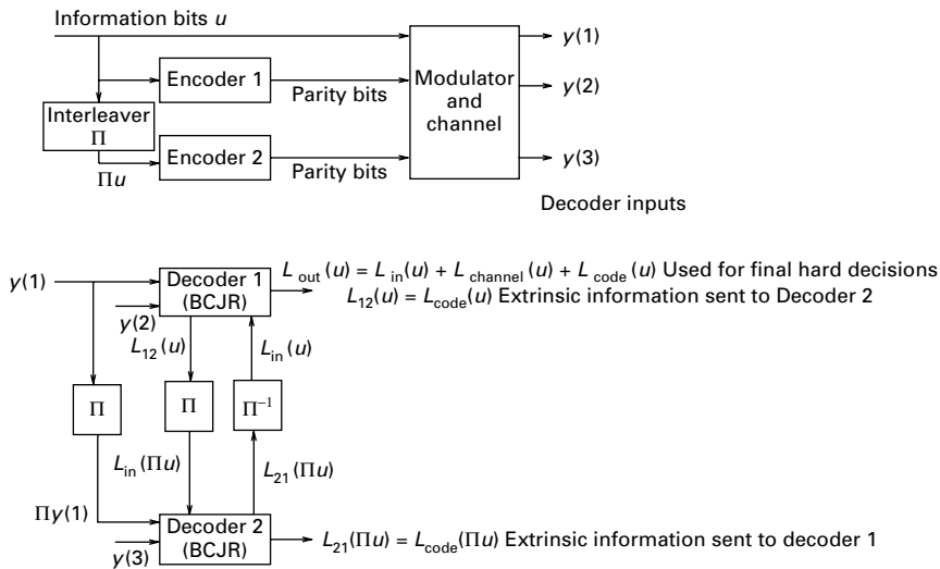
Figure 7.10 Encoder and decoder for a parallel concatenated turbo code.
