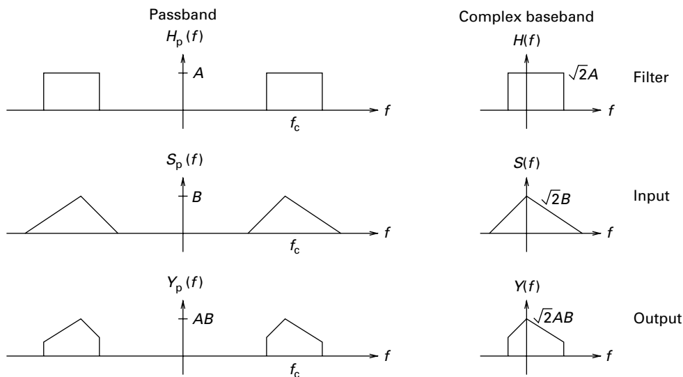
Figure 2.10 The relationship between passband filtering and its complex baseband analog.
