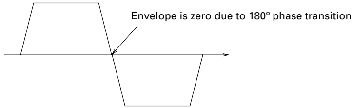
Figure 8.13 The envelope of a PSK signal passes through zero during a 180° phase transition, and gets distorted over a nonlinear channel.
