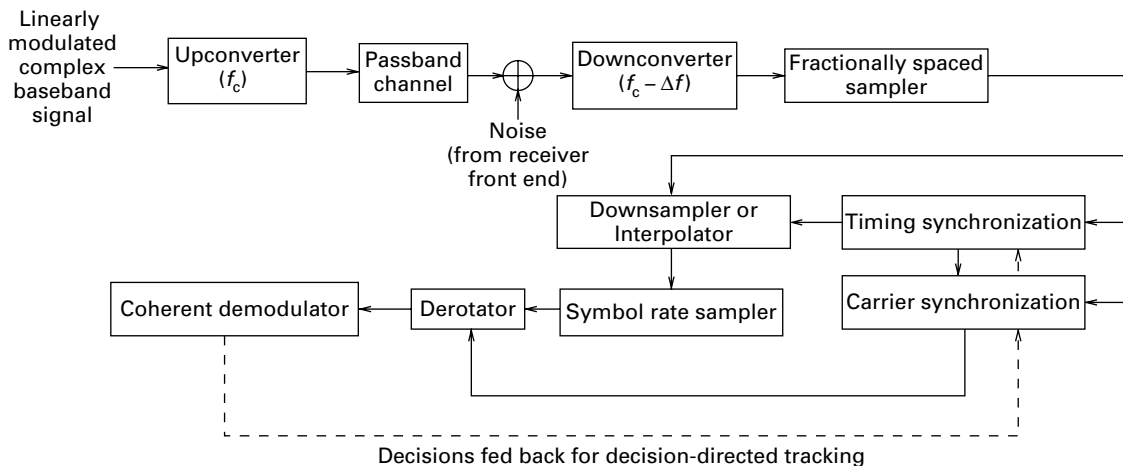
Figure 4.1 Block diagram of key transceiver blocks for synchronization and demodulation.
