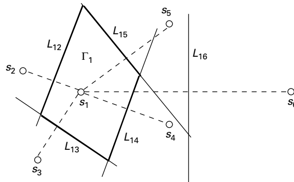
Figure 3.11 Maximum likelihood (ML) decision region \Gamma_1 for signal \mathbf{s}_1 .
