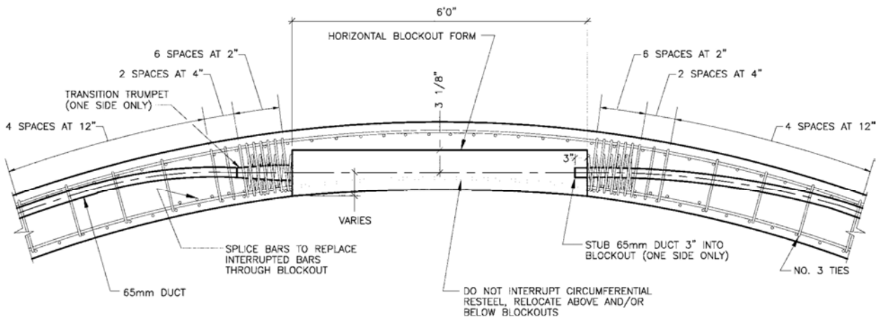
Fig. 5.3—Blockout detail.
