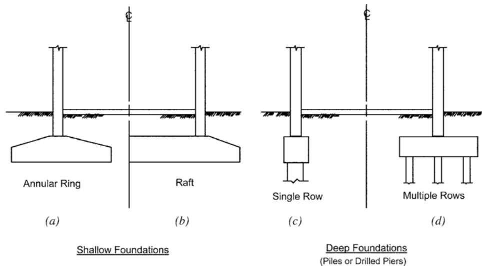
Fig. 5.1—Foundation types.
