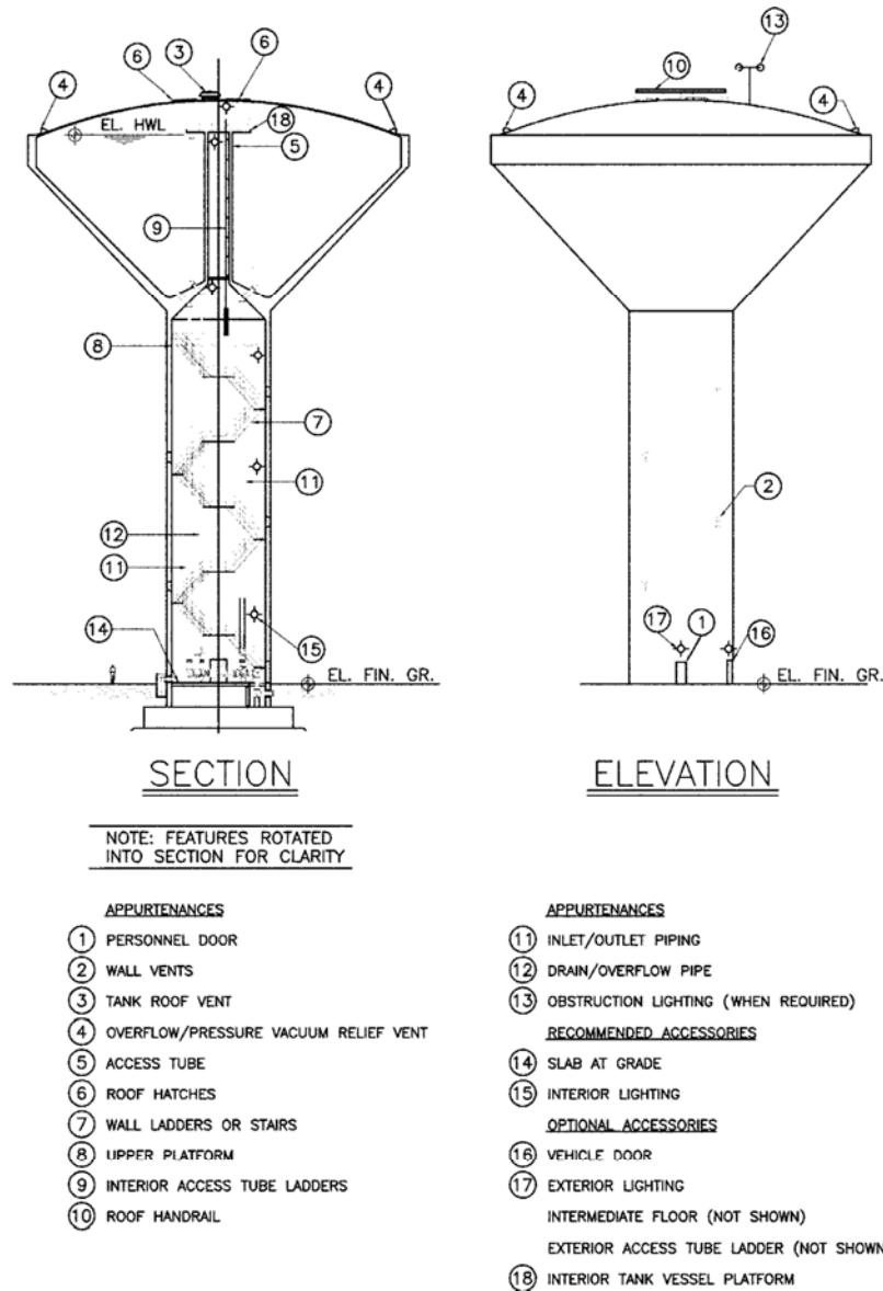
Fig. 7.1—Typical accessories and appurtenances for elevated concrete tanks.
