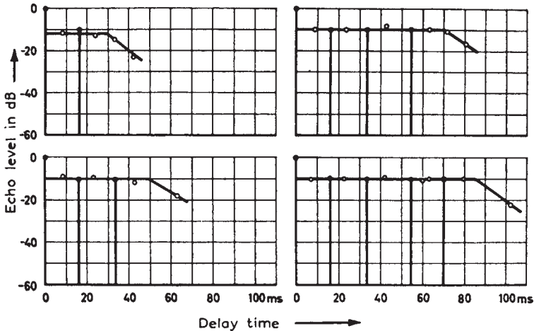
Figure 7.6 Threshold of absolute perceptibility of a delayed signal (reflection) being added to a sound field consisting of direct sound plus one, two, three or four reflections at fixed delay times and relative levels, which are denoted by vertical lines. The original sound signal is speech. All sound components arriving from the front (after Seraphim 7 ).
