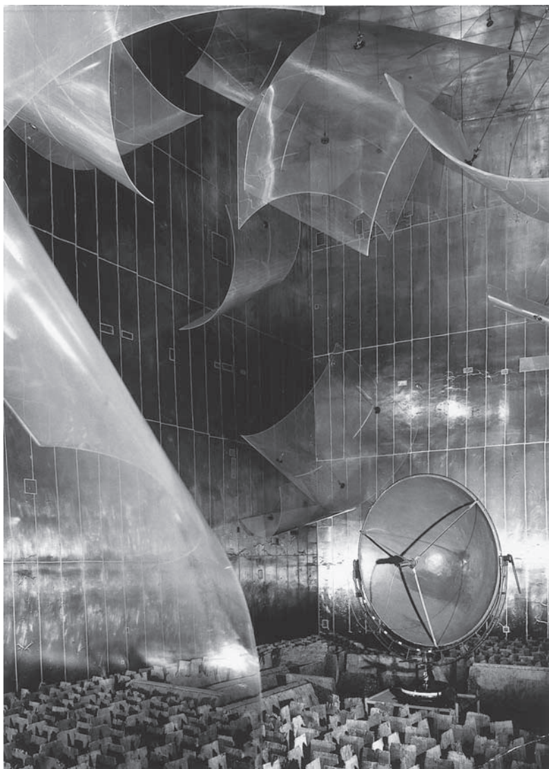
Figure 8.18 Reverberation chamber fitted out with 25 diffusers of perspex (volume 324 \text{ m}^3 ; dimensions of one shell 1.54 \text{ m} \times 1.28 \text{ m} ).
