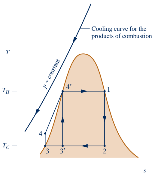
Fig. 8.5 Illustration used to compare the ideal Rankine cycle with the Carnot cycle.
