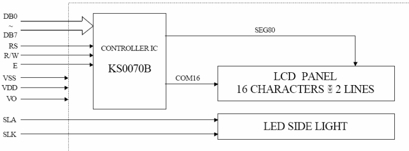
Fig. 8.16 LCD block diagram and pin out
