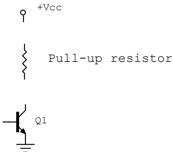
Fig. 4.1 Open-collector configuration
