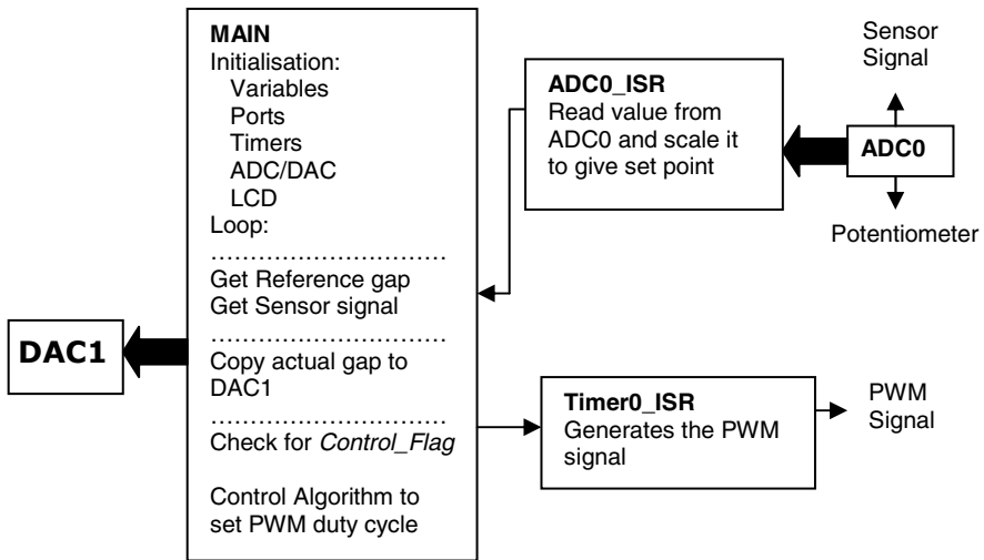
Fig. 7.26 Program structure
