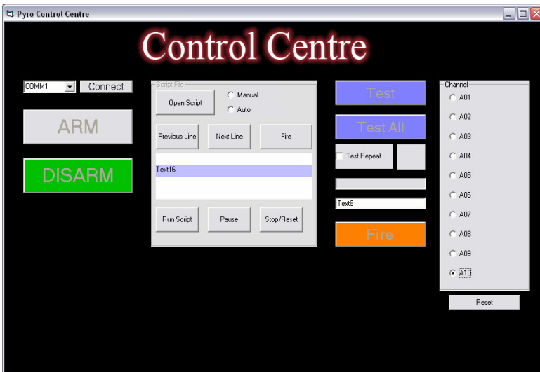
Fig. 8.3 Control software
