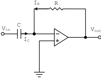
Fig. 1.11 A differentiator
