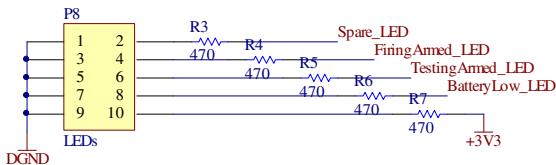
Fig. 8.18 LEDs schematic
