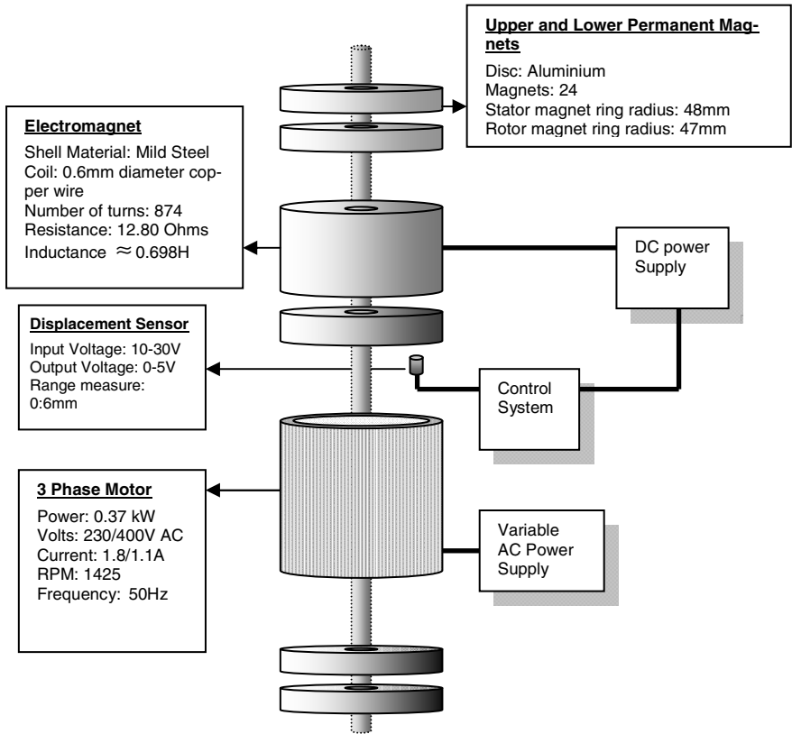
Fig. 7.2 Diagram showing the major components of the fabricated magnetic bearing system
