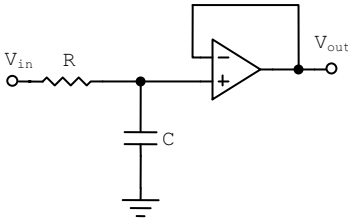
Fig. 1.17 Unity gain low pass filter
