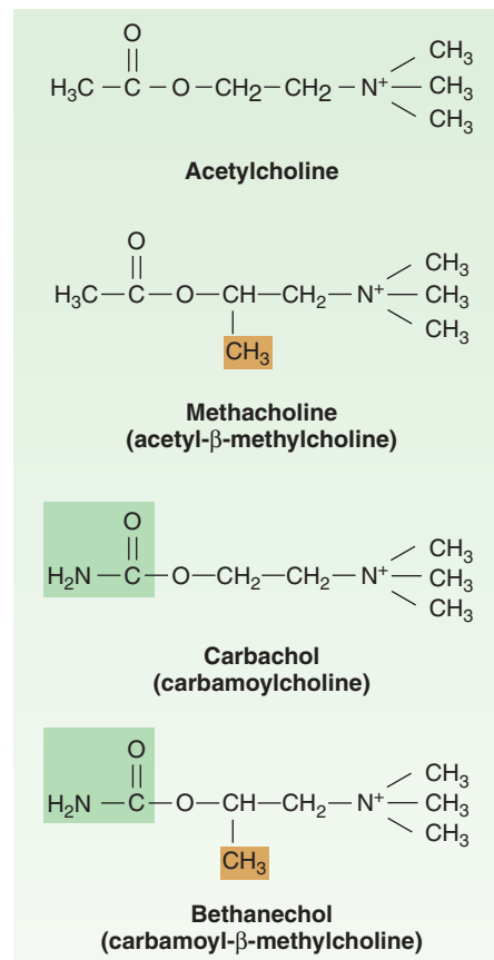
FIGURE 7–2 Molecular structures of four choline esters. Acetylcholine and methacholine are acetic acid esters of choline and \beta -methylcholine, respectively. Carbachol and bethanechol are carbamic acid esters of the same alcohols.
