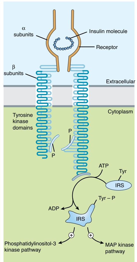
FIGURE 41–3 Schematic diagram of the insulin receptor heterodimer in the activated state. IRS, insulin receptor substrate; MAP, mitogen-activated protein; P, phosphate; Tyr, tyrosine.
