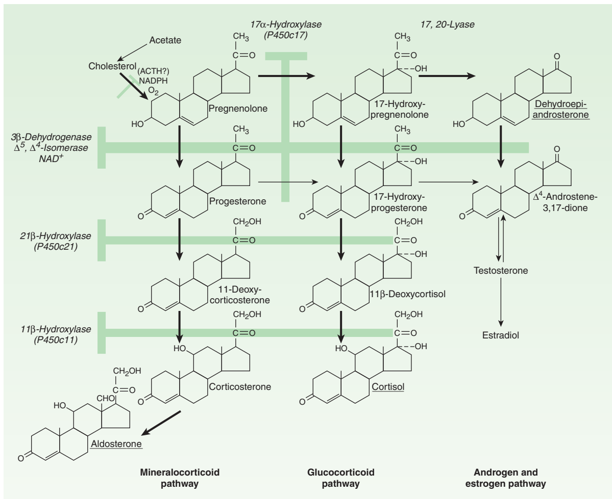
FIGURE 39–1 Outline of major pathways in adrenocortical hormone biosynthesis. The major secretory products are underlined. Pregnenolone is the major precursor of corticosterone and aldosterone, and 17-hydroxypregnenolone is the major precursor of cortisol. The enzymes and cofactors for the reactions progressing down each column are shown on the left and across columns at the top of the figure. When a particular enzyme is deficient, hormone production is blocked at the points indicated by the shaded bars. (Modified after Welikey et al; reproduced, with permission, from Ganong WF: Review of Medical Physiology , 17th ed. Originally published by Appleton & Lange. Copyright © 1995 by The McGraw-Hill Companies, Inc.)
