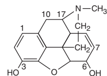
Morphine
