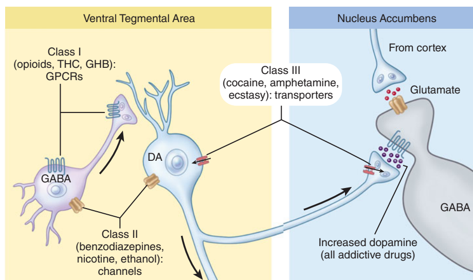
FIGURE 32-2 Neuropharmacologic classification of addictive drugs by primary target (see text and Table 32-1). DA, dopamine; GABA, γ-aminobutyric acid; GHB, γ-hydroxybutyric acid; GPCRs, G protein-coupled receptors; THC, Δ 9 -tetrahydrocannabinol.
