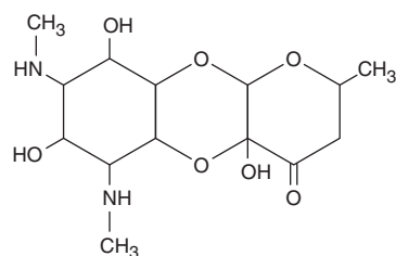
Spectinomycin
