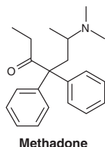
Methadone
