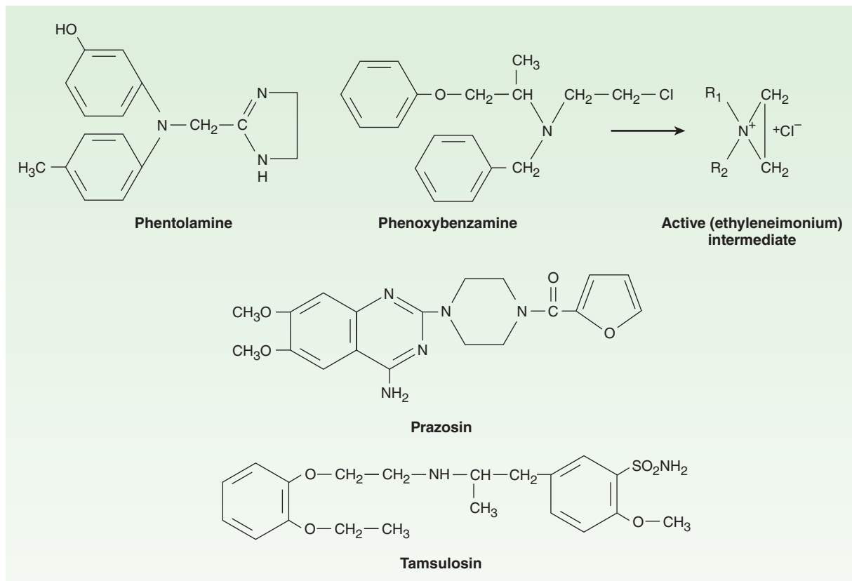
FIGURE 10-1 Structure of several \alpha -receptor-blocking drugs.
