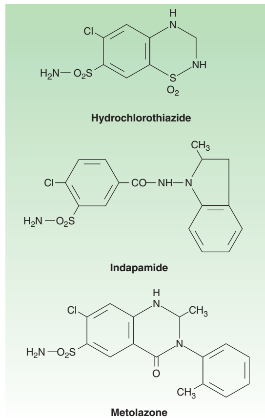
FIGURE 15–8 Hydrochlorothiazide and related agents.
