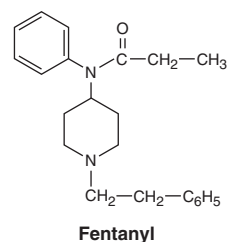
Fentanyl
