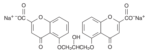
Cromolyn sodium
