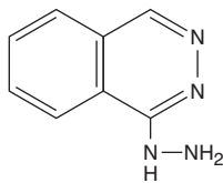
Hydralazine
