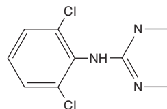
Clonidine
