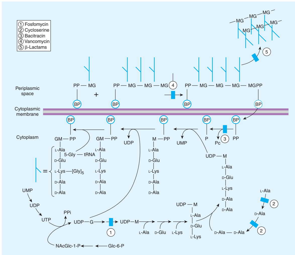
FIGURE 43-5 The biosynthesis of cell wall peptidoglycan, showing the sites of action of five antibiotics (shaded bars; 1 = fosfomycin, 2 = cycloserine, 3 = bacitracin, 4 = vancomycin, 5 = \beta -lactam antibiotics). Bactoprenol (BP) is the lipid membrane carrier that transports building blocks across the cytoplasmic membrane; M, N -acetylmuramic acid; Glc, glucose; NAcGlc or G, N -acetylglucosamine.
