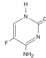
Flucytosine
