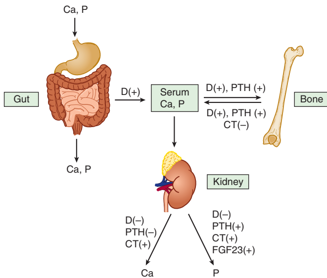
FIGURE 42-1 Mechanisms contributing to bone mineral homeostasis. Serum calcium (Ca) and phosphorus (P) concentrations are controlled principally by three hormones, 1,25-dihydroxyvitamin D (1,25[OH] 2 D, D), fibroblast growth factor 23 (FGF23), and parathyroid hormone (PTH), through their action on absorption from the gut and from bone and on renal excretion. PTH and 1,25(OH) 2 D increase the input of calcium and phosphorus from bone into the serum and stimulate bone formation. 1,25(OH) 2 D also increases calcium and phosphate absorption from the gut. In the kidney, 1,25(OH) 2 D decreases excretion of both calcium and phosphorus, whereas PTH reduces calcium but increases phosphorus excretion. FGF23 stimulates renal excretion of phosphorus. Calcitonin (CT) is a less critical regulator of calcium homeostasis, but in pharmacologic concentrations can reduce serum calcium and phosphorus by inhibiting bone resorption and stimulating their renal excretion. Feedback may alter the effects shown; for example, 1,25(OH) 2 D increases urinary calcium excretion indirectly through increased calcium absorption from the gut and inhibition of PTH secretion and may increase urinary phosphate excretion because of increased phosphate absorption from the gut and stimulation of FGF23 production.
