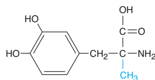
\alpha -Methyldopa ( \alpha -methyl group in color)
