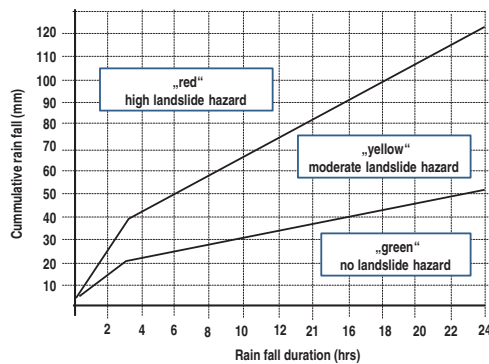
Fig. 3.35 NOAA/USGS empirical “rainfall intensity–duration threshold” for the San Francisco Bay area (Redrawn from USGS 2005c)
