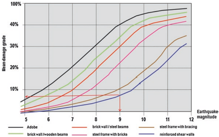
Fig. 3.13 Vulnerability classes according to building/construction type (Based on EMS-98)
