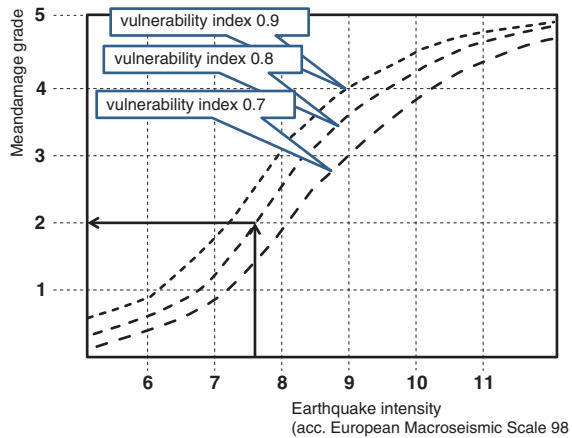
Fig. 6.10 Mean damage grade based on vulnerability curves from relating to vulnerability indices of the Manjil earthquake 1990 (Courtesy Omnidar et al. 2011)
