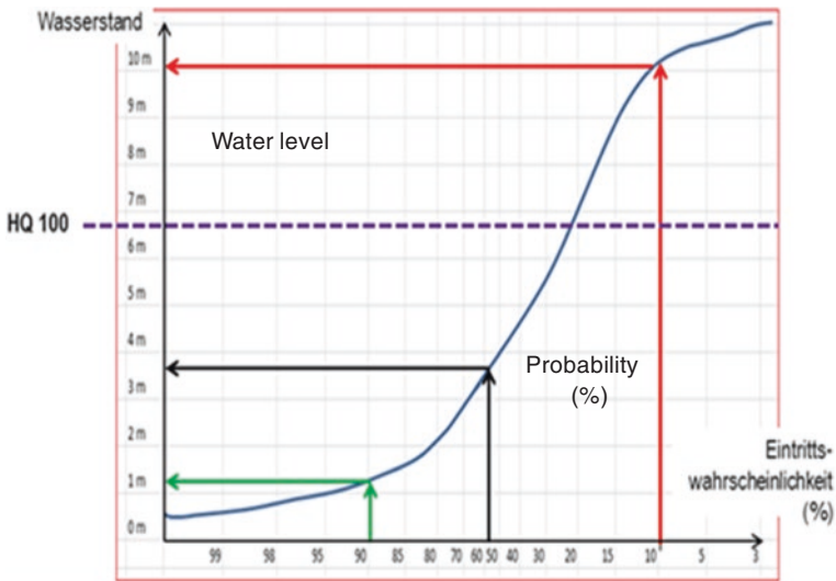
Fig. 6.5 Cumulative curve on probability of exceedance of flood levels (fictitious)
