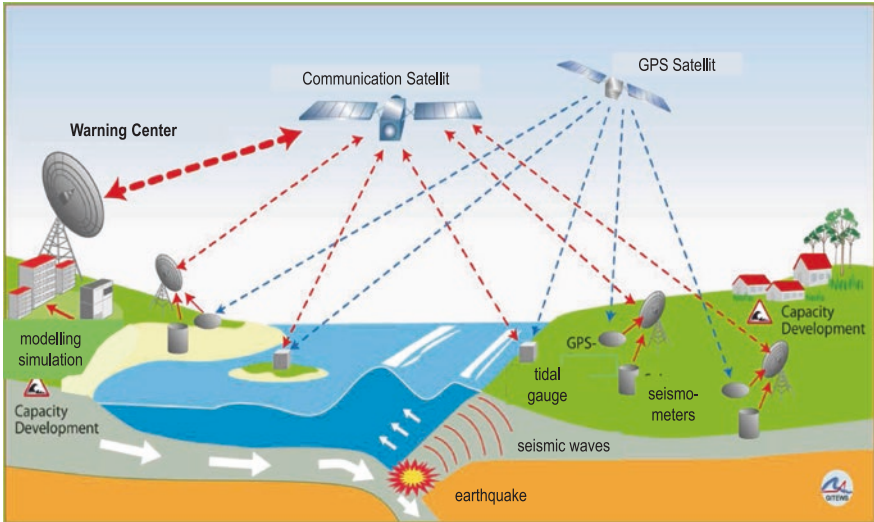
Fig. 9.5 Concept of the GITEWS tsunami early warning communication system (Courtesy Rudloff et al. 2009)
