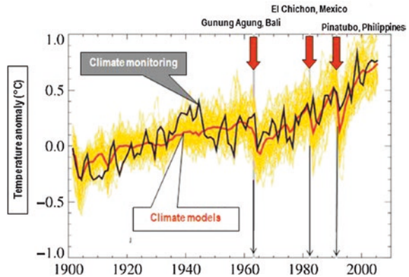
Fig. 3.26 Drop in atmospheric temperature due to volcanic ash emissions from volcanoes Gunung Agung (Bal), El Chichon (Mexico), and Pinatubo (Philippines) (Based on: IPCC 2007)
