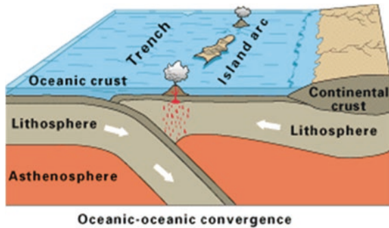
Fig. 3.7 Oceanic–oceanic plate convergence (Courtesy USGS, ibid)
