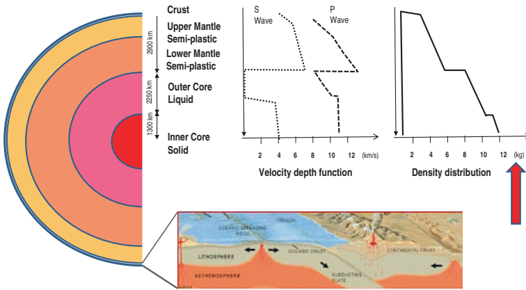
Fig. 3.2 Structure of the Earth and respective seismic velocity and density distribution (Compiled from USGS 2008a; Berckheimer 1990)
