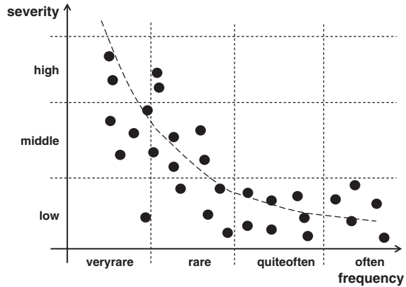
Fig. 6.9 Probability estimate of possible earthquake occurrence from historical magnitude and frequency distribution (fictitious)
