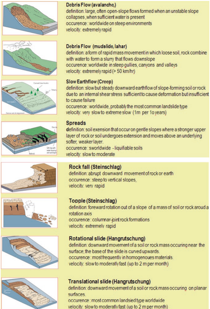
Fig. 3.34 Generalized overview of landslide types (Courtesy USGS 2008c)
