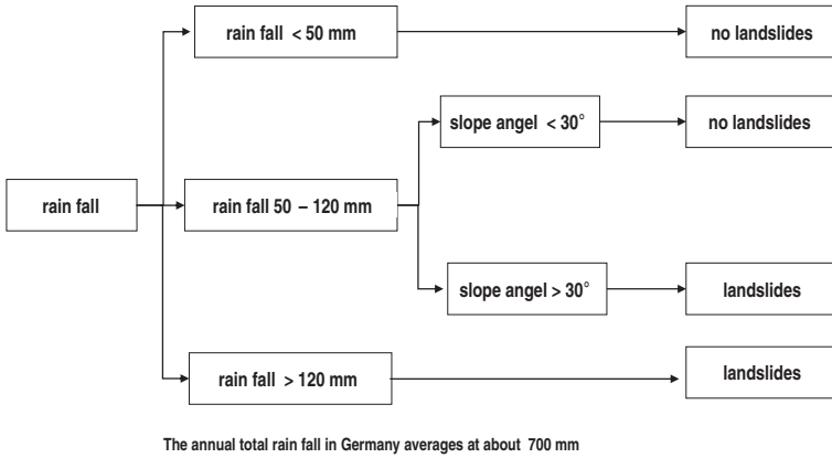
Fig. 3.36 Decision tree for the occurrence of landslides (Generalized after Hamberger 2007)
