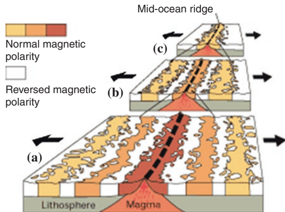
Fig. 3.3 Magnetic striping pattern of the oceanic crust as a result of the reversing of the Earth's magnetic field (Courtesy USGS 2008a)
