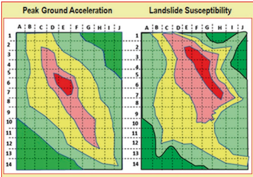
Fig. 5.14 Multiple hazard assessment based on peak ground acceleration and landslide susceptibility (“fictitious”): dark green 1; lush green 2; yellow 3; pink 4; red 5 (Own graph)
