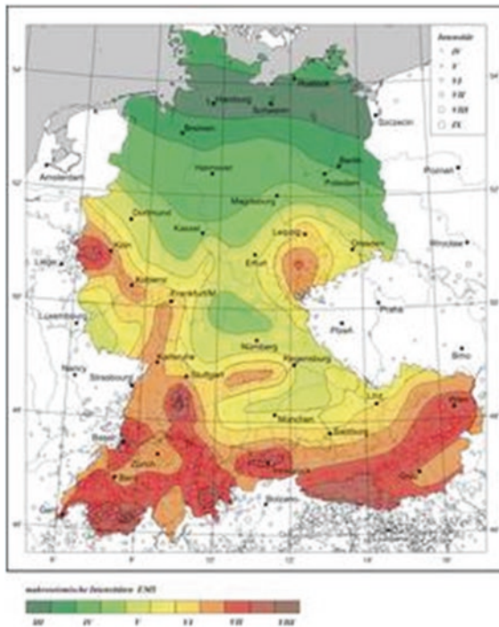
Fig. 3.17 Earthquake Map of Germany, Austria, and Switzerland (D-A-CH), based on earthquake intensities that will not exceed 90 % probability in the next 50 years ( Courtesy Helmholtz Centre Potsdam—GFZ German Research Centre for Geosciences, Annual Report 2011)
