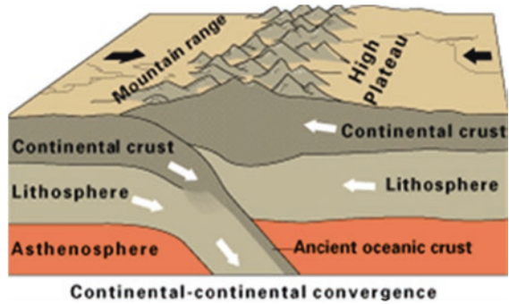
Fig. 3.8 Continental plate–continental plate collision (Courtesy USGS, ibid )
