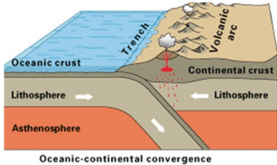
Fig. 3.6 Oceanic–continental plate convergence (Courtesy USGS, ibid)
