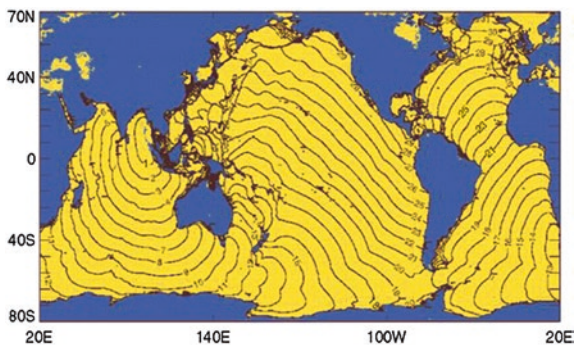
Fig. 3.23 2004 Indian Ocean tsunami travel times (Courtesy Kowalik et al. 2005)
