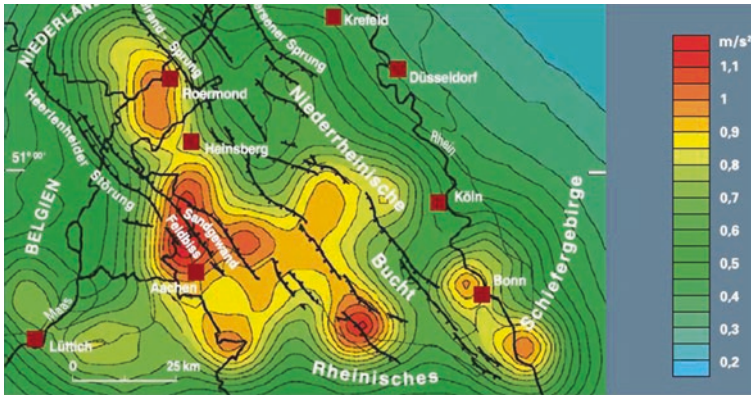
Fig. 3.16 Earthquake hazard of the Niederrheinische Bucht based on maximal horizontal acceleration exceeding one in 500 years ( Courtesy Geological Survey of North Rhine-Westphalia, Germany)
