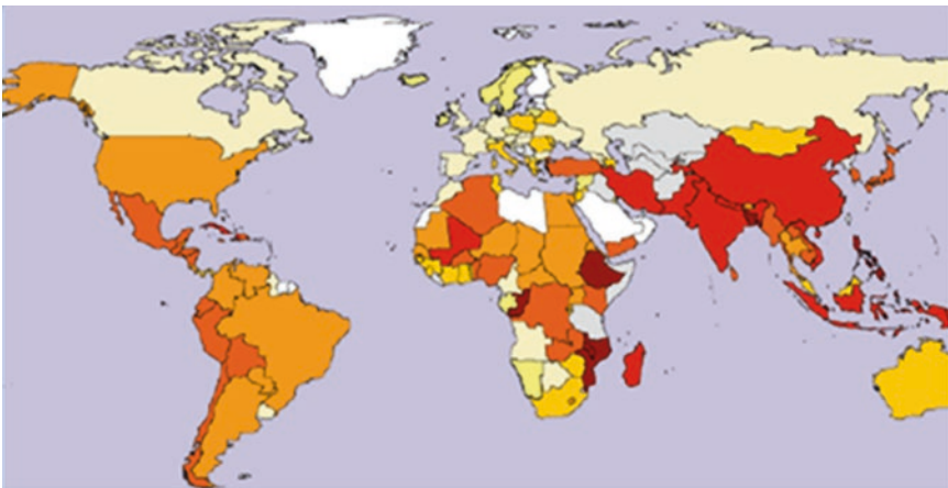
Fig. 3.43 Spatial distribution of risk mortality classes assessed by the Disaster Risk Index (DRI) of the UNDP-GRAVITY Programme (Courtesy Peduzzi et al. 2005)
