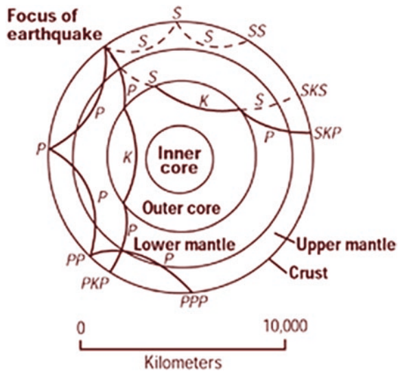
Fig. 3.11 Seismic ray paths through Earth’s interior (Courtesy USGS, ibid)
