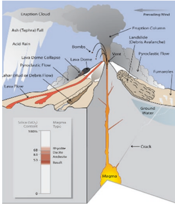
Fig. 3.28 Simplified sketch of typical hazards from strato volcanoes (Courtesy USGS 2008b)
