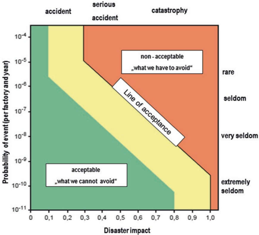
Fig. 8.9 Definition of risk acceptance on Swiss nuclear power generation plants (v. Piechowski, cited in WBGU, Report 1999; Courtesy Springer)
