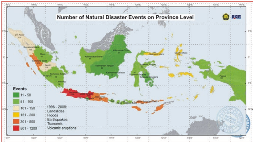
Fig. 5.4 Regional distribution of disaster events of Indonesia at provincial level (Courtesy Badan Geology/Gitews 2005, Indonesia)
