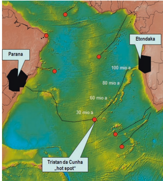
Fig. 3.30 Hotspots in the South Atlantic and their travel paths (Graph based: Duncan and Richards 1991)
