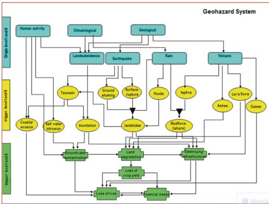
Fig. 5.12 Generalized cause-effect relationship of natural hazards (Own graph)
