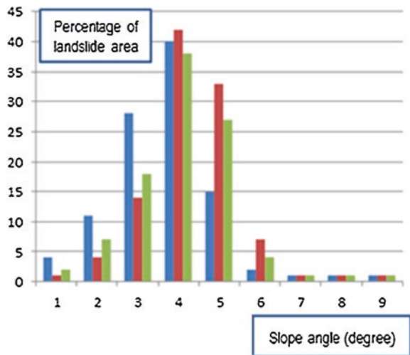
Fig. 3.37 Percentage of landslide areas following the 2008 Wenchuan earthquake (Redrawn from Tang et al. 2011)
