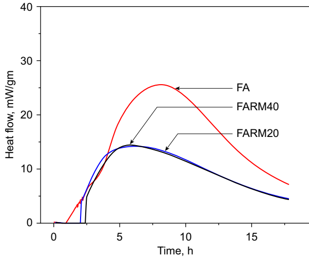
Figure 14.7 Isothermal conduction calorimetric curve of red mud-based geopolymer at elevated temperature (60 °C).
