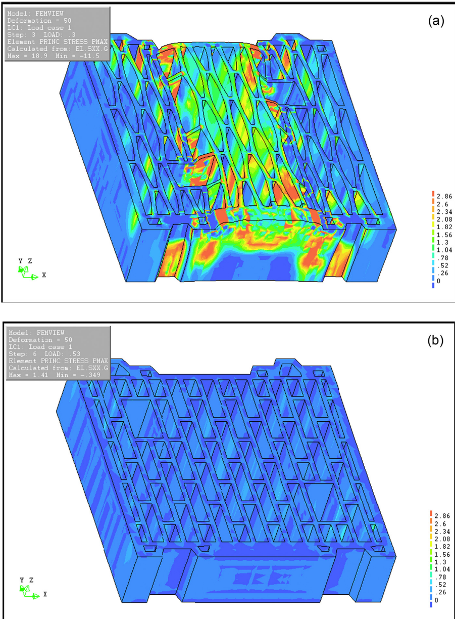
Figure 2.6 Distribution of principal tensile stresses (units in \text{N/mm}^2 ): (a) shell bedded clay unit; (b) full bedded clay unit.
