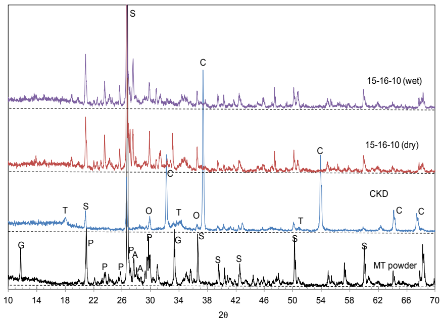
Figure 13.8 XRD patterns of MT and CKD powders and geopolymer blocks prepared at 15 M NaOH, 16% initial water content, 10% CKD, and cured at 90 °C for seven days and before and after immersion in water (A: albite, G: gypsum, P: sanidine, S: quartz, C: CaO, O: CaCO 3 , S: SiO 2 , T: Ca(OH) 2 ).
