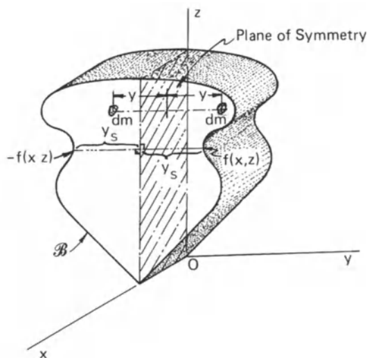
Figure 9.2. A homogeneous body having an xz -plane of symmetry.
