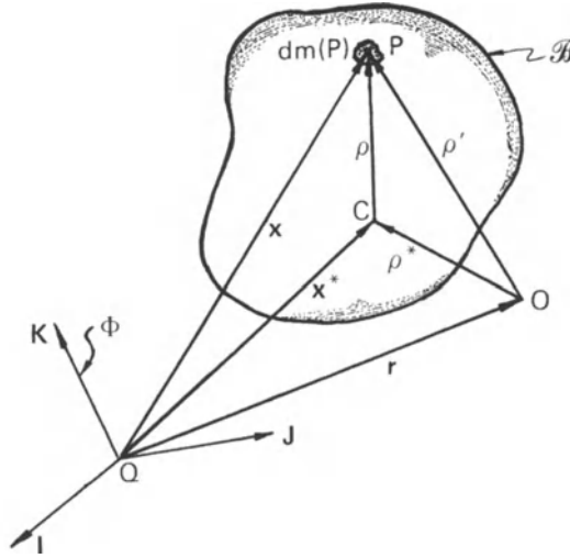
Figure 5.2. Schema for the center of mass properties of a body.
