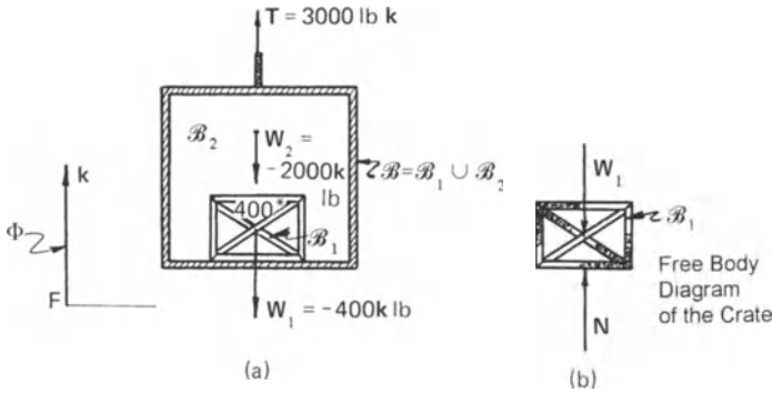
Figure 10.3. Forces on a rigid crate in a moving elevator.
