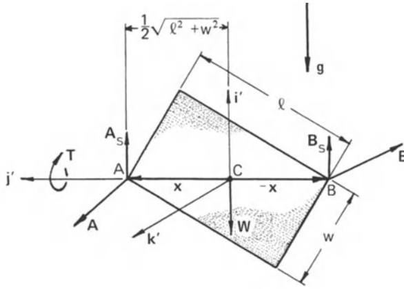
Figure 10.10. Free body diagram of the rotating plate.
