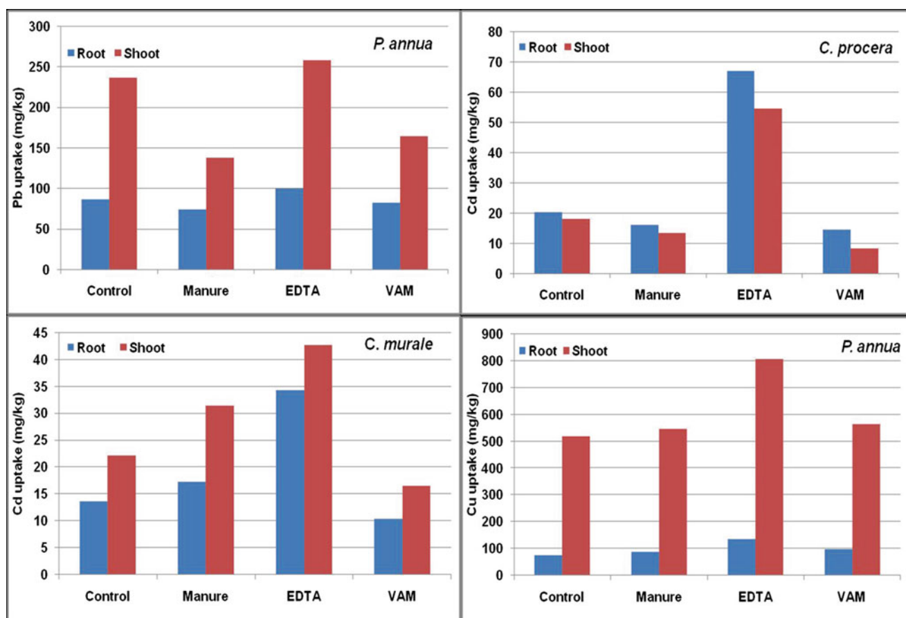
Fig. 13.3 Metal concentrations in test plants (mg kg -1 ) in response to soil amendments
