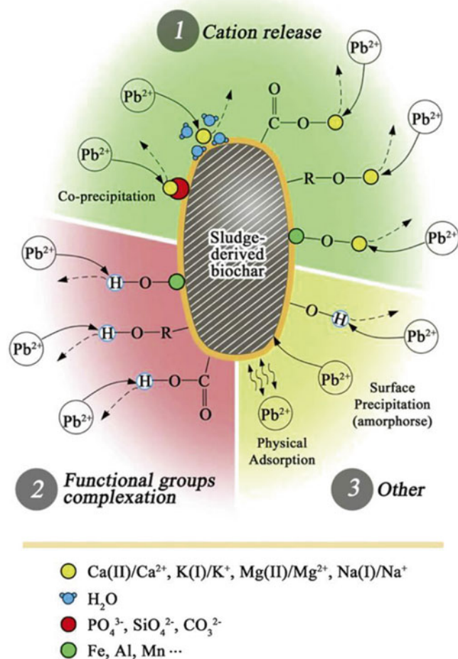
Fig. 17.1 Conceptual illustration of Pb adsorption mechanism on SDBC, including (1) metal exchange with \text{Ca}^{2+} and \text{Mg}^{2+} , attributing to coprecipitation and inner sphere complexation with complexed humic matter and mineral oxides of SDBC; (2) surface complexation with free carboxyl and hydroxyl functional groups and inner sphere complexation with the free hydroxyl of mineral oxides and other surface precipitation; (3) other inner sphere complexation with the free hydroxyl of mineral oxides and other surface precipitation (from Lu et al. 2012)
