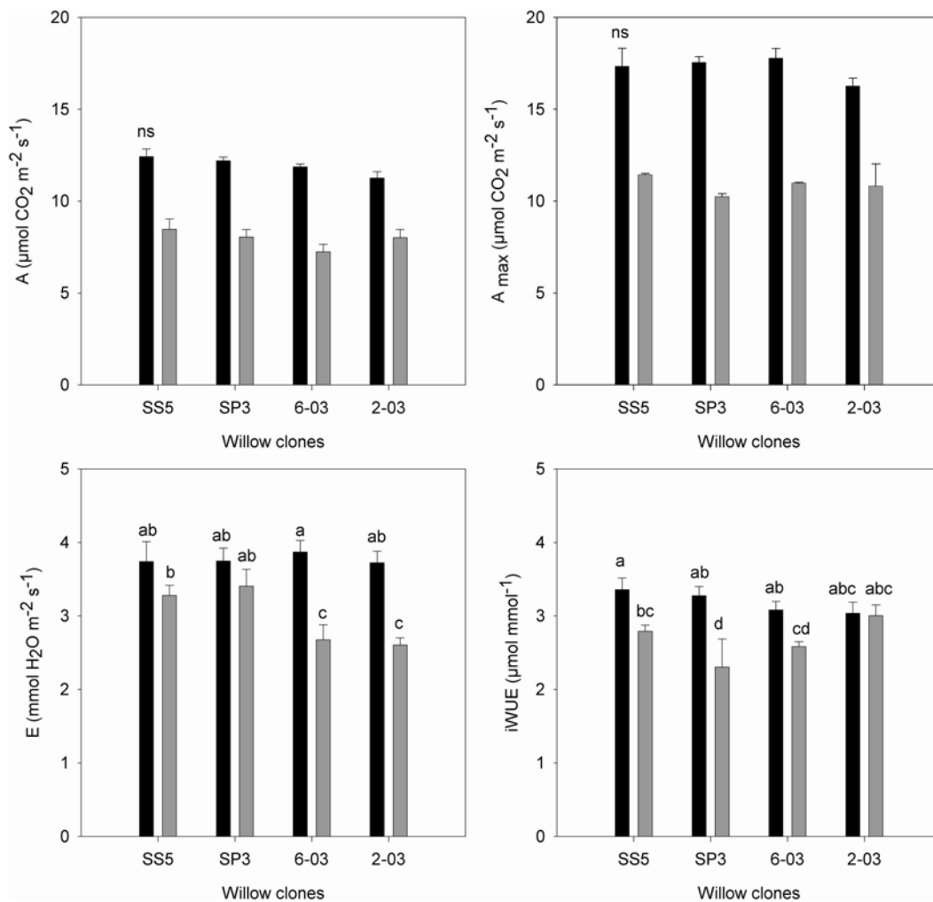
Fig. 7.5 Measurements of net photosynthesis in growth ( A ) and in saturating light conditions ( A_{\text{max}} ), transpiration rate ( E ) and instantaneous water use efficiency ( i\text{WUE} ) in leaves of willow clones grown for 3 weeks in the presence of 0 \mu\text{M} (control, black bars) and 50 \mu\text{M}
