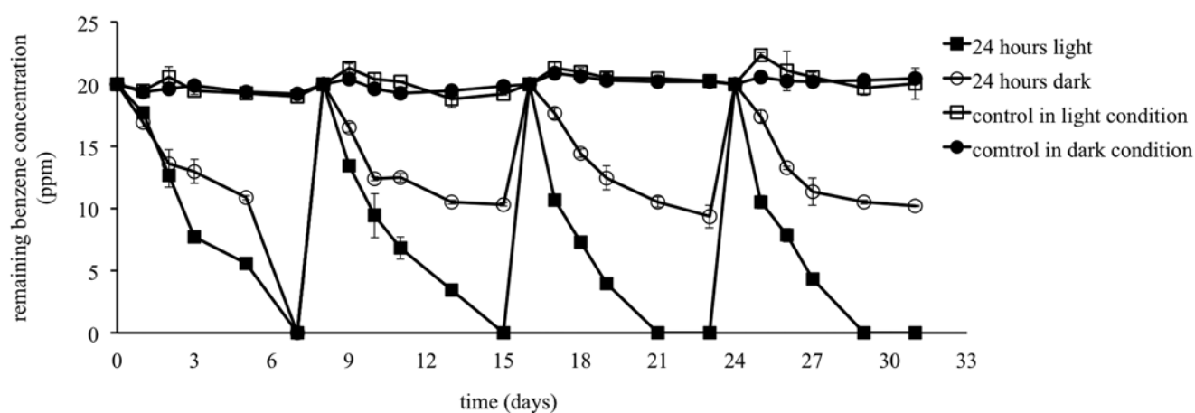
Fig. 20.6 Remaining benzene in 4-cycle experimental system observation of benzene exposure plant growth under 24 h of light and 24 h of dark conditions (Reprinted from Treesubstunorn and Thiravetyan 2012 with permission from Elsevier)
