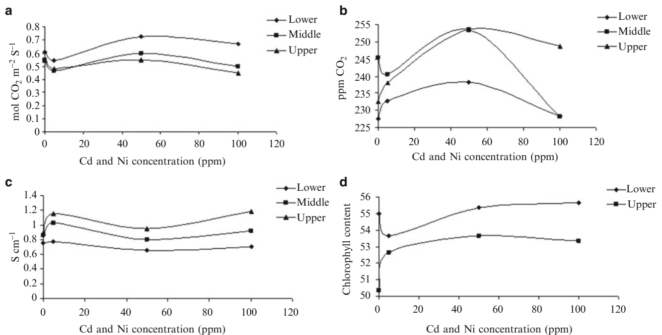
Fig. 1.4 The effect of different concentrations of Cd and Ni on (a) stomatal conductance, (b) intercellular CO 2 concentration, (c) stomatal resistance, and (d) chlorophyll content of lower, middle, and upper leaves of giant reed (modified after Papazoglou et al. 2007)
