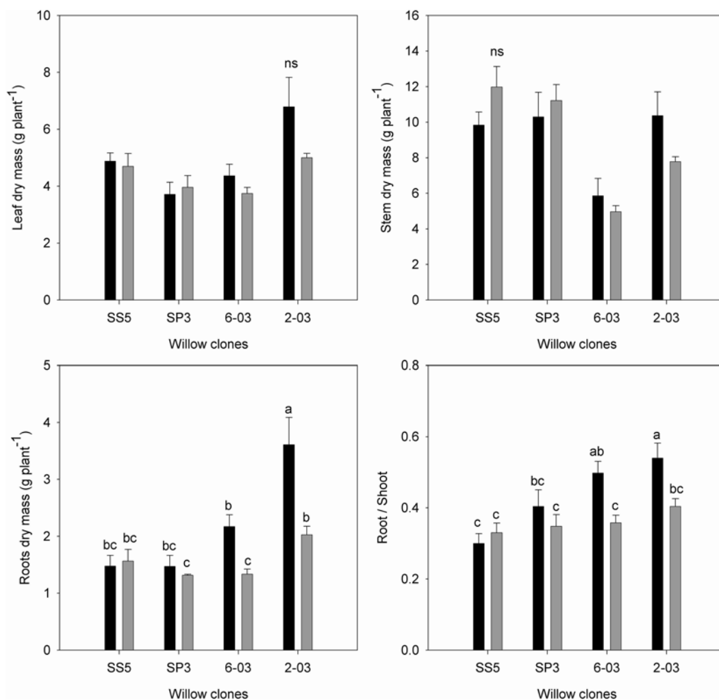
Fig. 7.1 Leaf, stem and root dry mass (g plant -1 ) and root-to-shoot ratio in willow clones grown for 3 weeks in the presence of 0 \mu M (control, black bars) and 50 \mu M (grey bars) CdSO 4 in hydroponics
