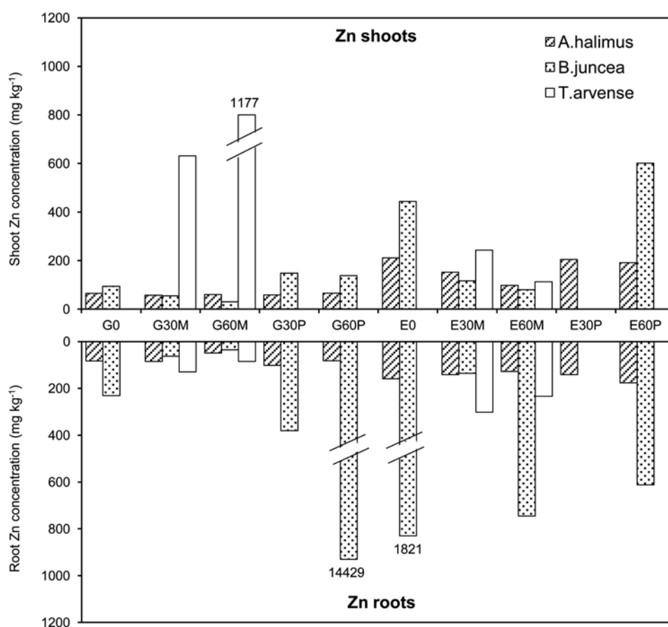
Fig. 22.3 Zn concentrations in shoots and roots of the tolerant plant species in the treatments of mine soils with organic amendments. Soils: G, Garganta; E, El Cuadron. Organic amendments: M, manure; P, pine bark. Application rates ( \text{t ha}^{-1} ): 0, 30, and 60
