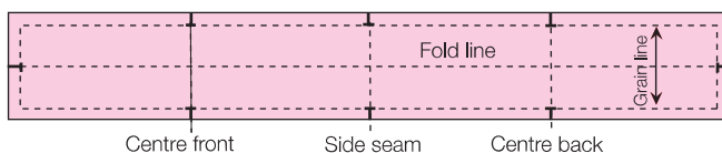
Skirt waistband Size 10 Cut 1 x self + blk fuse 1cm seam allowance
