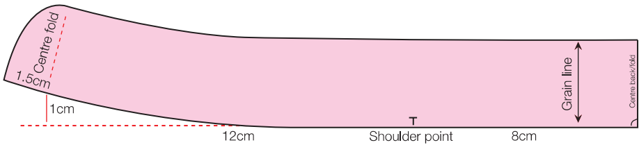
Basic stand-up collar
