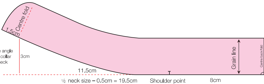
Tighter fitting stand-up collar
