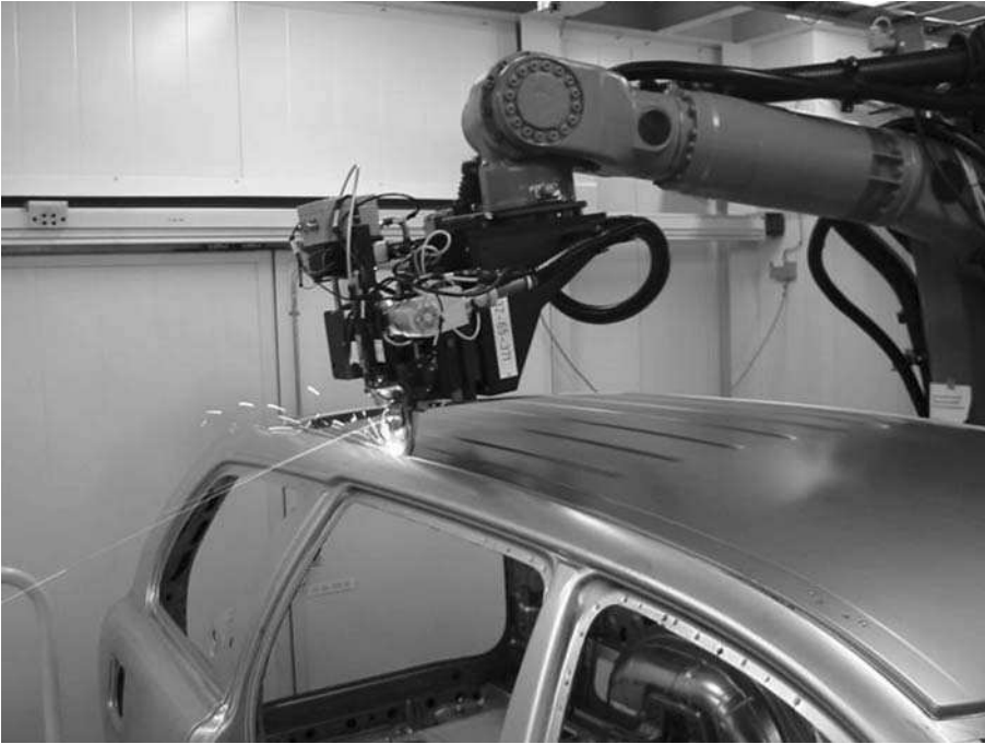
Figure 2.4 Roof edge laser welding of the Volvo XC90. (Source: Johnny Larsson, Volvo Car Corporation, Gothenburg, Sweden)
