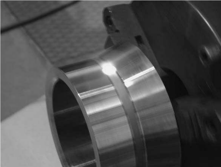
Figure 9.11 Diode laser hardening of an alloy steel machine component: power 2 kW, traverse rate 1 \text{ m min}^{-1} . (Source: Henrikki Panssar, Lappeenranta University of Technology, Finland)
