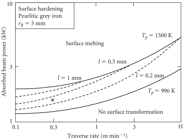
Figure 9.7 Laser hardening diagram for a pearlitic grey iron treated with a beam of width 5 mm: the theoretical operating window is bounded by solid lines, representing the onset of surface melting (1500 K), and surface transformation (996 K); contours of transformed depth ( T_p = 996 K) are shown as broken lines; and the diagram is calibrated using a data point (an experimental measurement) indicated by a star
