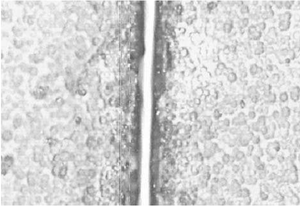
Figure 7.4 Entrance to a slot machined in a piezoceramic of thickness 115\text{ }\mu\text{m} , using 400 pulses of energy density 17\text{ J cm}^{-2} and duration 25 ns made using an ArF excimer laser. (Source: Jan Brune, Lambda Physik AG, Microlas Application Laboratory, Göttingen, Germany)
