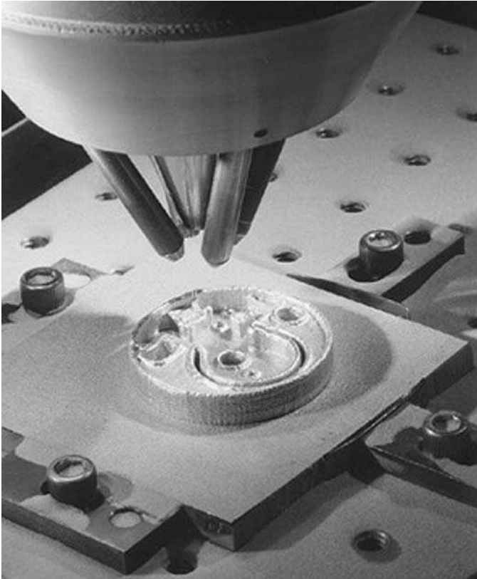
Figure 1.8 Component fabrication using Laser Engineered Net Shaping (LENS TM ) direct metal fabrication process. (Source: Clint Atwood, Sandia National Laboratories, Albuquerque, NM, USA and Sylvia Nasla, MTS, Eden Prairie, MN, USA.) LENS TM is a trademark of Sandia National Laboratories
