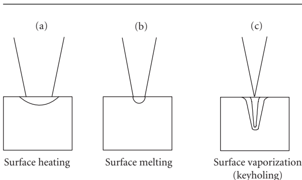
Figure 6.1 The effect of power density on the interaction mechanism between a laser beam and a large block of material under steady state conditions
