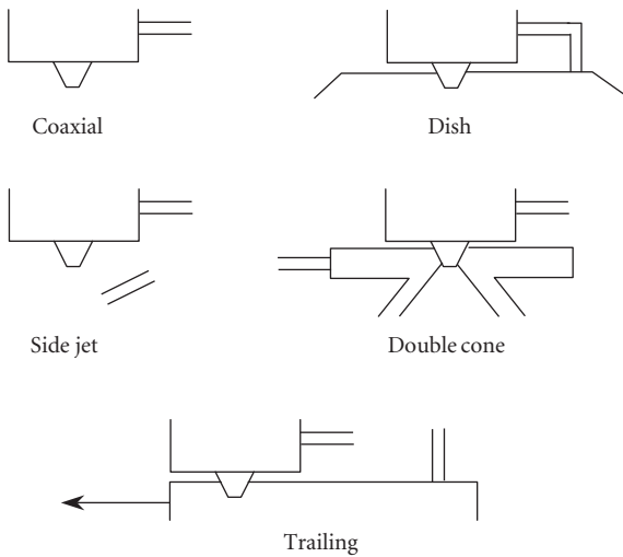
Figure 16.7 Gas delivery nozzles used in laser welding
