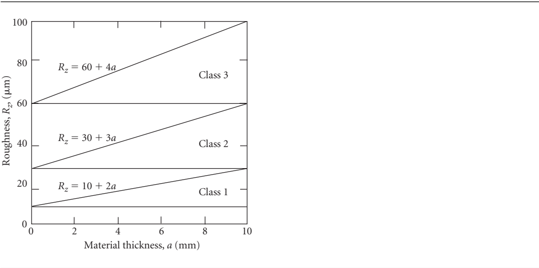
Figure 14.6 Quality classes for thermal cutting based on edge roughness (ISO, 2002)
