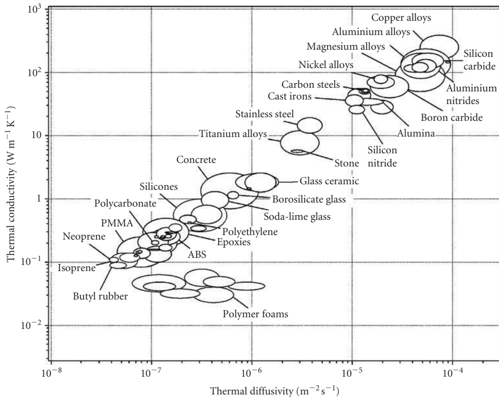
Figure 5.12 Thermal conductivity plotted against thermal diffusivity for engineering materials. (Source: CES 4.1 2003 Granta Design, grantadesign.com)
