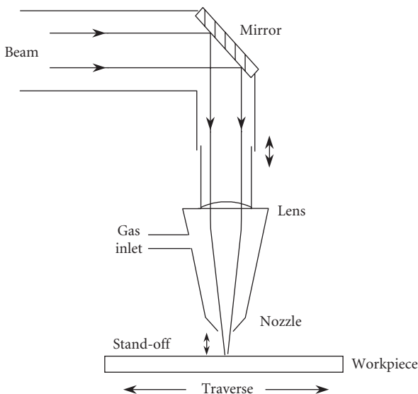
Figure 14.4 Schematic design of a laser cutting head
