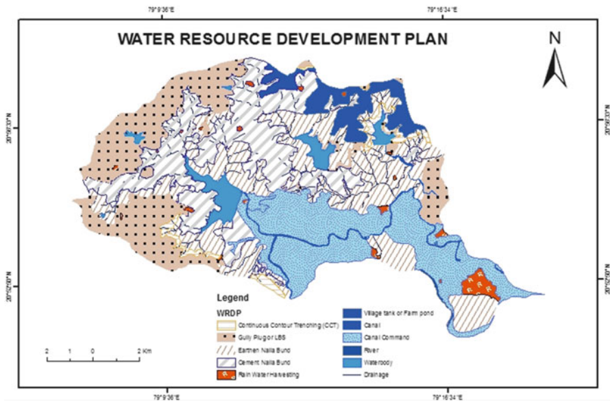
Fig. 18.3 Water resource development map
