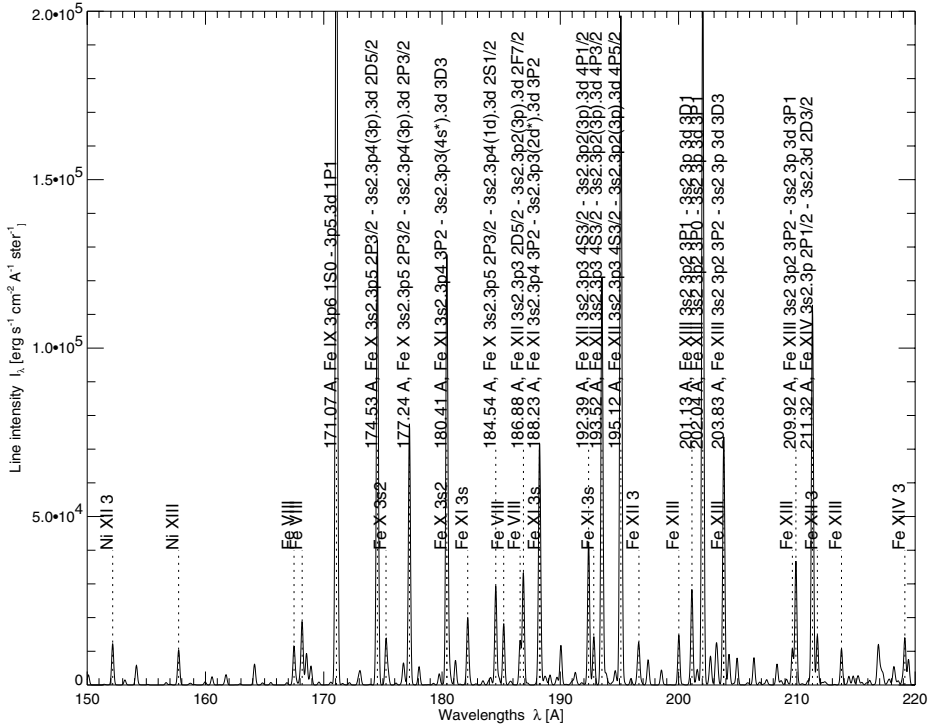
Figure 2.11: A synthetic spectrum calculated in the \lambda = 150\text{--}220 \text{ \AA} wavelength range with the CHIANTI code, using the Feldman (1992) abundances, the Arnaud & Raymond (1992) values for the ionization equilibrium, a DEM for a typical active region, and n_e T = 10^{15} \text{ cm}^{-3} \text{ K} , plotted with a wavelength resolution of 0.2 \text{ \AA} . The strongest lines are identified, mostly Fe lines, and transitions calculated by CHIANTI are indicated. Note the prominent Fe IX at 171 \text{ \AA} and Fe XII at 195 \text{ \AA} that are frequently used in SoHO/EIT and TRACE images.
