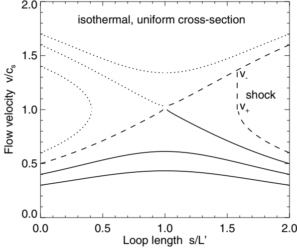
Figure 4.1: The flow speed v(s)/c_s (normalized by the sound speed) as a function of the normalized loop length s/L according to the steady-flow solution of Eq. (4.2.7), for an isothermal loop with uniform loop cross section. Flows at the critical speed (dashed line) become supersonic beyond the loop summit ( s=L ) and are slowed down from v_- to v_+ by a shock wave. Unphysical or fully supersonic solutions are marked with dotted lines (after Cargill & Priest 1980).
