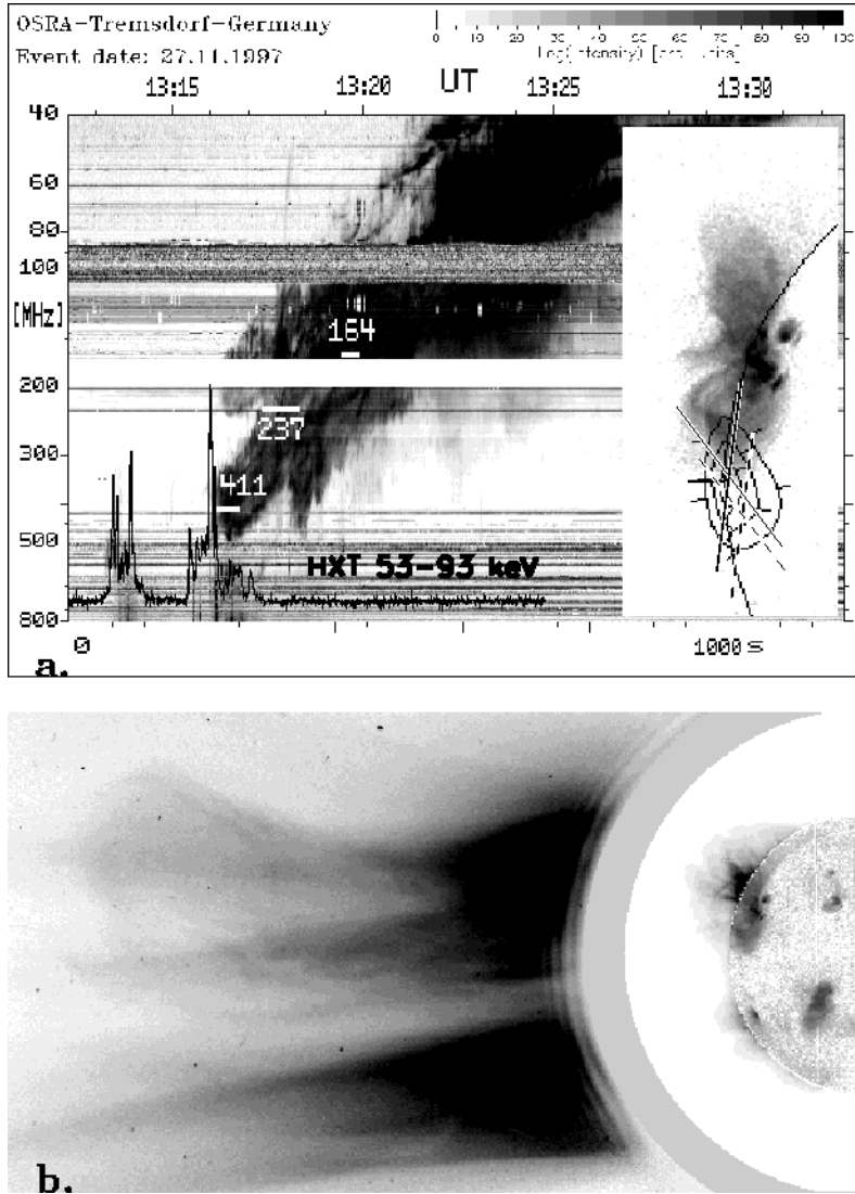
Figure 11.21: (a) Dynamic spectrogram (Tremdsdorf Radio spectrograph) and hard X-ray lightcurve (Yohkoh HXT) during the 1997-Nov-27 type II event. Insert to (a): Yohkoh SXT negative image of AR 8113 (Al.I filter) at 12:40:36 UT and harmonic type II source during the time intervals indicated by horizontal bars at the appropriate frequencies in the spectrogram: contours of equal brightness at 411 MHz (10, 50, 90% of maximum brightness in the image) and source centroid positions and half widths of the harmonic type II sources at 237 (dashed) and 164 MHz (solid). (b) Yohkoh SXT image of (a), superposed on SoHO/LASCO-C1 and C2 images at 1328 and 1330 UT (negative image). Note that the shock waves that produce radio type II emission are imaged in the lower corona very close to the flare site (top right), while the CME bowshock is about 5 solar radii away (bottom left), and thus cannot be responsible for the type II emission (Klein et al. 1999b).
