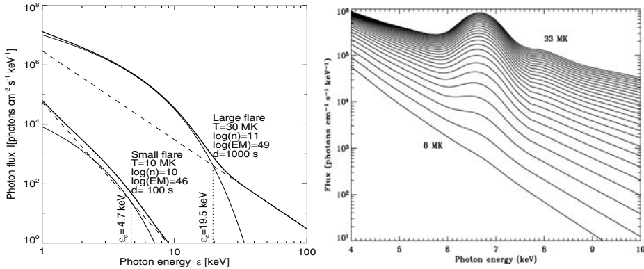
Figure 13.5: (Left) Theoretical hard X-ray spectrum consisting of a thermal and a nonthermal (powerlaw) component with equal energy content above the cutoff energy \varepsilon_c . The parameters are chosen for a large flare with T_e = 30 MK, n_e = 10^{11} cm -3 , EM_V = 10^{49} cm -3 , \gamma = 3 , and duration \tau_{flare} = 1000 s; and for a small flare with T_e = 10 MK, n_e = 10^{10} cm -3 , EM_V = 10^{46} cm -3 , \gamma = 5 , and duration \tau_{flare} = 100 s. (Right) Synthetic spectra between 4 and 10 keV show line features at 6.7 keV (Fe) and at 8.2 keV (Fe/Ni) that become progressively stronger for increasing flare temperatures. The spectra have been calculated with the CHIANTI code, with coronal abundances of Fe and Ni, and smoothed with a Gaussian filter with a width of FWHM=0.8 keV. Spectra are given in 1 MK intervals from 8 to 33 MK. Fluxes are those at the mean solar distance and for a flare with volume emission measure \int_V n_e^2 dV = 10^{49} cm -3 (Phillips 2004).
