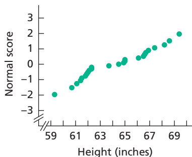
FIGURE 9.12 Normal probability plot of the heights in Table 9.9
