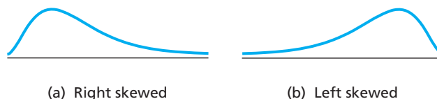
FIGURE 2.13 Generic skewed distributions: (a) right skewed and (b) left skewed
