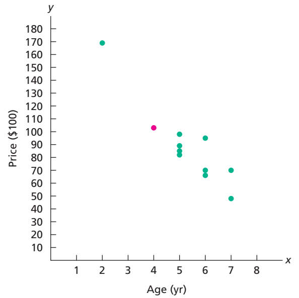
FIGURE 14.7 Scatterplot for the age and price data of Orions from Table 14.2
