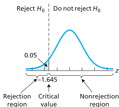
FIGURE 9.3 Rejection region, nonrejection region, and critical value for the golf-driving-distances hypothesis test
