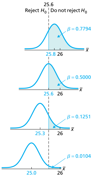
FIGURE 9.36 Type II error probabilities for \mu = 25.8 , 25.6, 25.3, and 25.0 ( \alpha = 0.05 , n = 30 )
