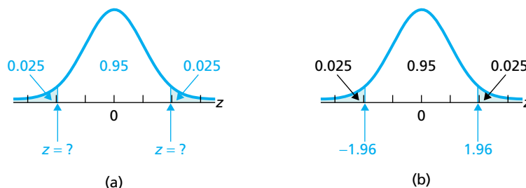
FIGURE 6.23 Finding the two z -scores that divide the area under the standard normal curve into a middle 0.95 area and two outside 0.025 areas
