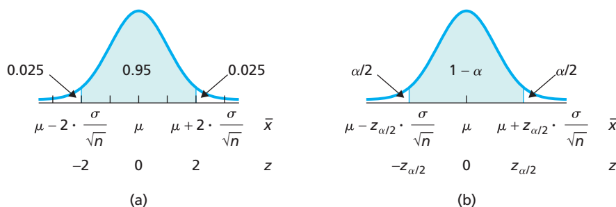
FIGURE 8.3 (a) Approximately 95% of all samples have means within 2 standard deviations of \mu ; (b) 100(1 - \alpha)\% of all samples have means within z_{\alpha/2} standard deviations of \mu
