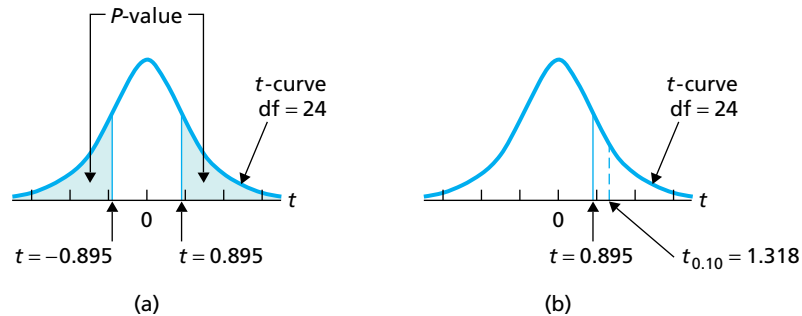
FIGURE 9.20 Estimating the P -value of a two-tailed t -test with a sample size of 25 and test statistic t = -0.895
