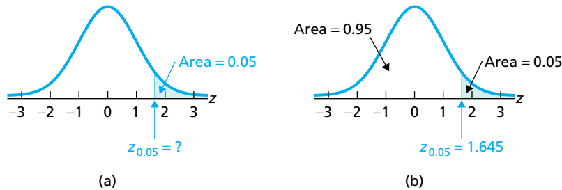
FIGURE 6.22 Finding z_{0.05}
