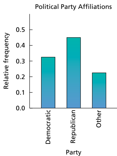
FIGURE 2.3 Bar chart of the political party affiliation data in Table 2.1
