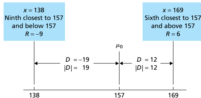
FIGURE 9.24 Meaning of signed ranks for the observations 138 and 169
