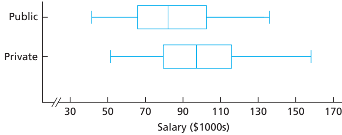
FIGURE 10.3 Boxplots of the salary data for faculty in private institutions and public institutions
