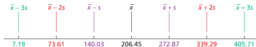
FIGURE 3.11 The mean and one, two, and three standard deviations to either side of the mean for the PCB-concentration data
