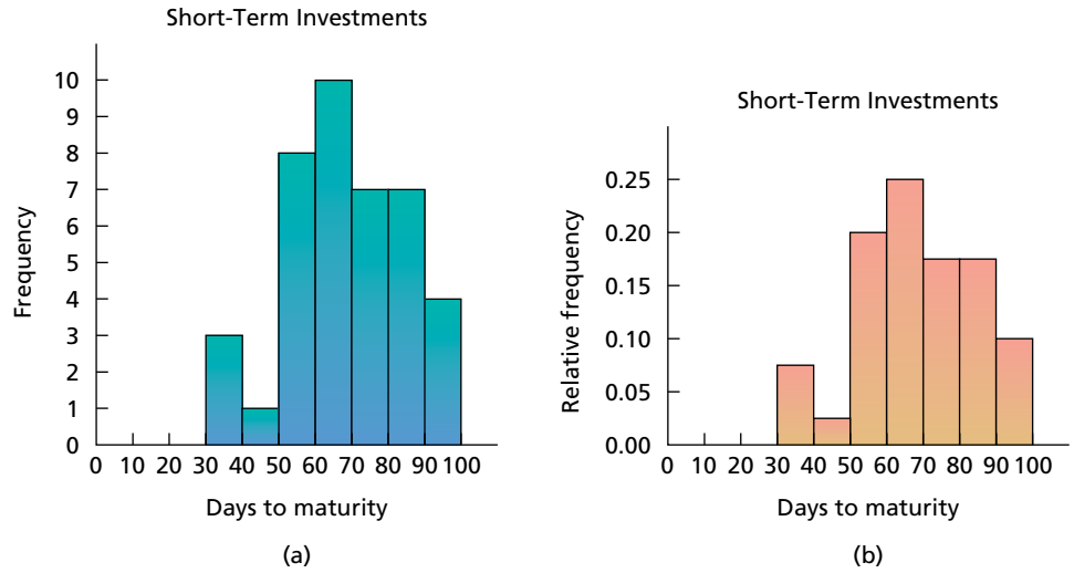
FIGURE 2.5 Limit grouping. Days to maturity: (a) frequency histogram; (b) relative-frequency histogram
