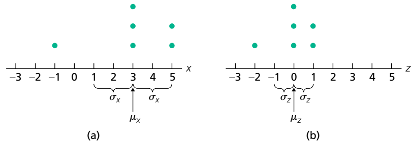
FIGURE 3.19 Dotplots of the distributions of x and its standardized version z
