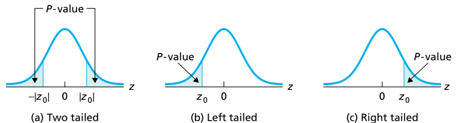
FIGURE 9.8 P-value for a one-mean z -test if the test is (a) two tailed, (b) left tailed, or (c) right tailed
