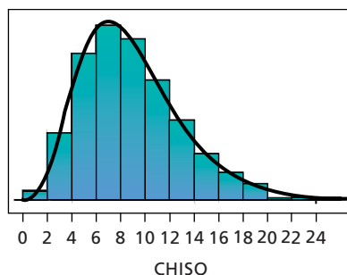
OUTPUT 11.1 Histogram of \chi^2 for 1000 samples of 10 capsule weights with superimposed \chi^2 -curve
