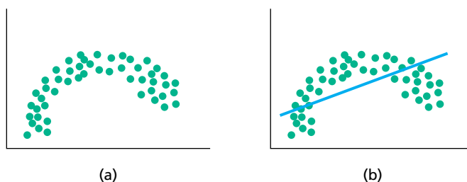
FIGURE 14.14 (a) Data points scattered about a curve; (b) inappropriate line fit to the data points
