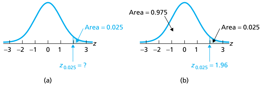
FIGURE 6.21 Finding z_{0.025}
