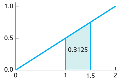
FIGURE 6.5 Area under the density curve between 1 and 1.5
