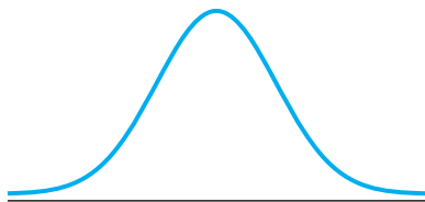
FIGURE 6.7 A normal curve
