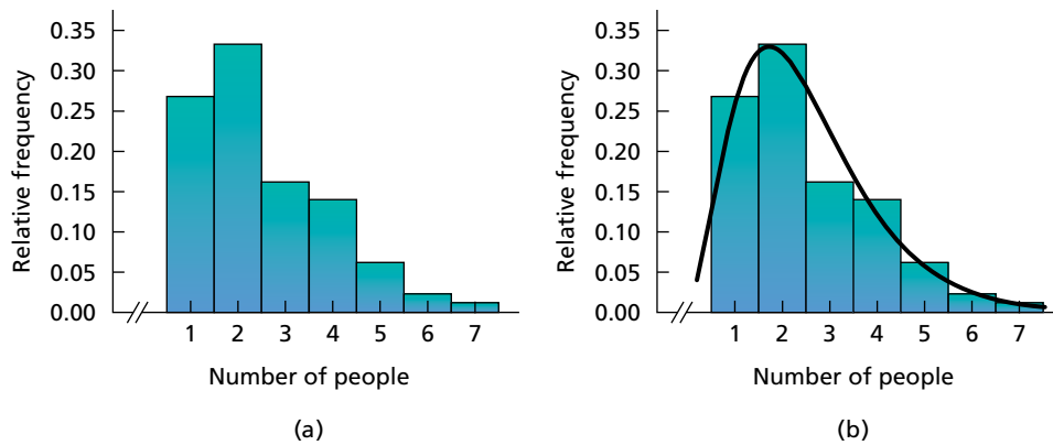
FIGURE 2.15 Relative-frequency histogram for household size
