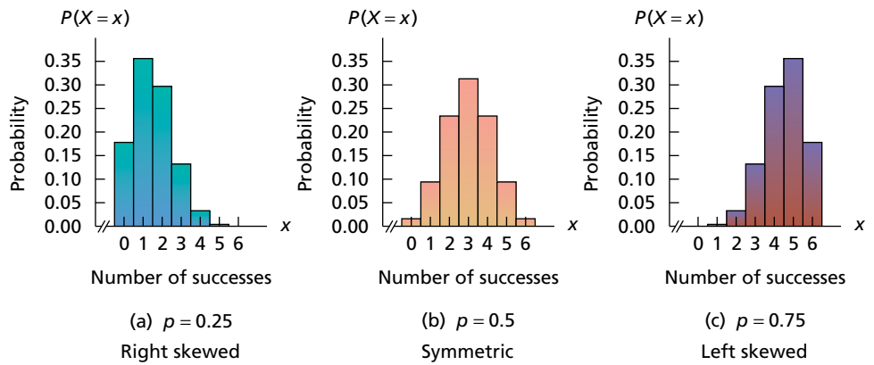
FIGURE 5.6 Probability histograms for three different binomial distributions with parameter n = 6
