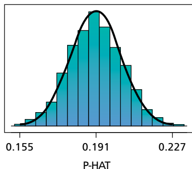
OUTPUT 12.1 Histogram of \hat{p} for 2000 samples of size 1010 with superimposed normal curve
