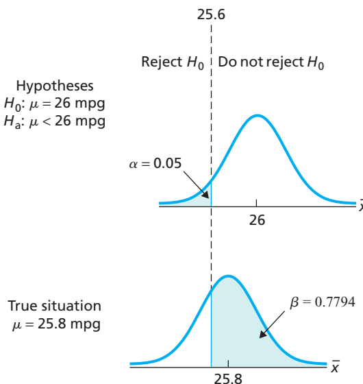
FIGURE 9.32 Decision criterion and Type II error probability when true mean is 25.8 mpg ( \alpha = 0.05, n = 30 )
