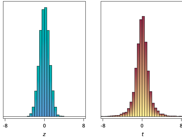
OUTPUT 8.2 Histograms of z (standardized version of \bar{x} ) and t (studentized version of \bar{x} ) for 5000 samples of size 4
