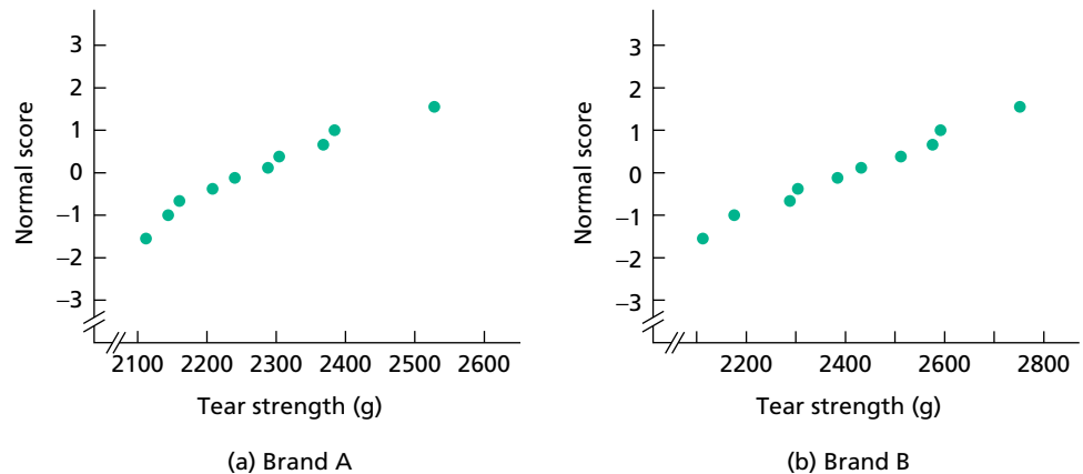
FIGURE 11.11 Normal probability plots of the sample data for (a) Brand A and (b) Brand B
