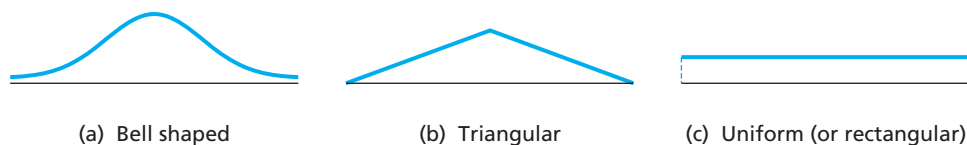
FIGURE 2.12 Examples of symmetric distributions: (a) bell shaped, (b) triangular, and (c) uniform
