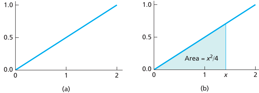
FIGURE 6.3 (a) Density curve for crystal side length, in mm (b) Area under the density curve to the left of x
