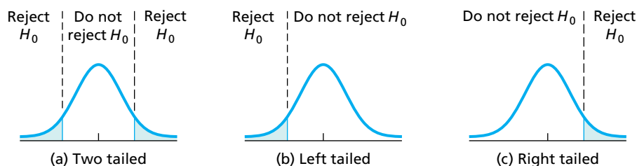
FIGURE 9.4 Graphical display of rejection regions for two-tailed, left-tailed, and right-tailed tests
