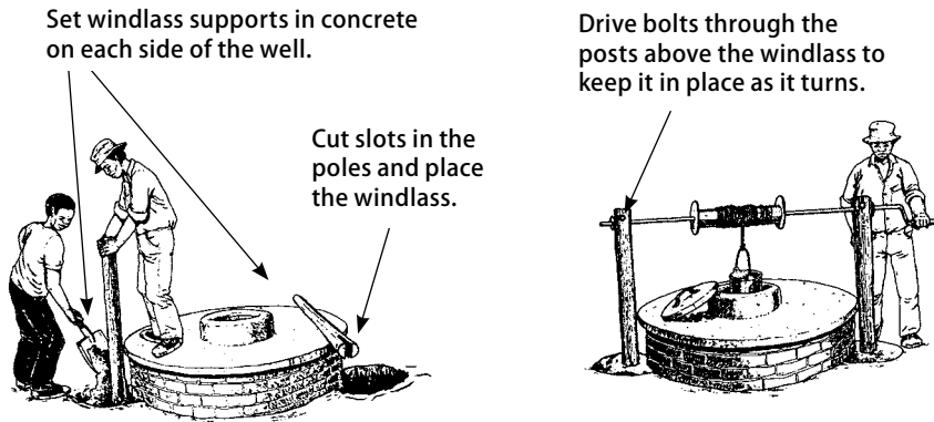
This design shows wooden windlass supports set in the ground. Windlass supports may also be made of bricks.
