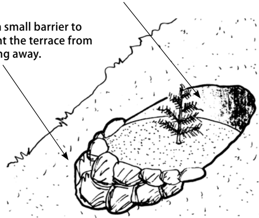
Dig a 1 meter circle above where the tree will be planted and form a flat terrace.
