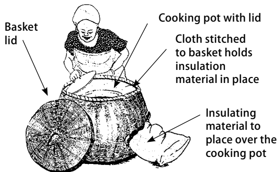
A haybox cooker made with a basket.
