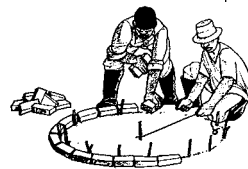
Make a mold for the slab.
