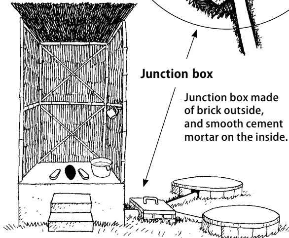
Above ground chamber allows wastewater to flow down to pits. With regular care, this toilet will last many, many years.
