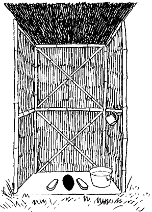
One lined pit underground, 2 meters deep. A family of 5 will fill this pit in about 5 years time.
