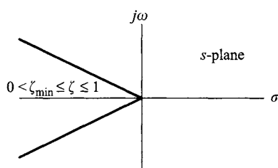
FIGURE 10.5: Minimal damping ratio \zeta of the closed-loop system: the poles lie in the sector \{\lambda \in \mathbb{C} : |\operatorname{Im}(\lambda)| \leq -\operatorname{Re}(\lambda)\sqrt{\zeta^{-2} - 1}\} .
