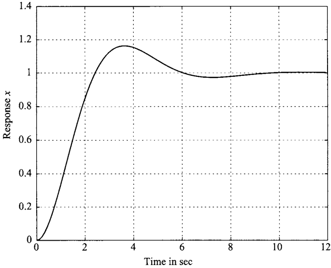
FIGURE 10.3: Unit step response when \zeta = 0.5 and \omega_n = 1 .
