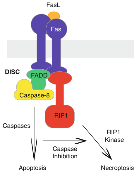
Fig. 16.1 Model of Fas receptor-stimulated pathways resulting in cell death. FasL binding induces dimerization of Fas in the cell membrane to recruit RIP1, FADD, and caspase-8 to form the DISC. Caspase-8 is activated to induce apoptosis; however, when caspases are inhibited, cell death occurs via RIP1 kinase-mediated necroptosis
