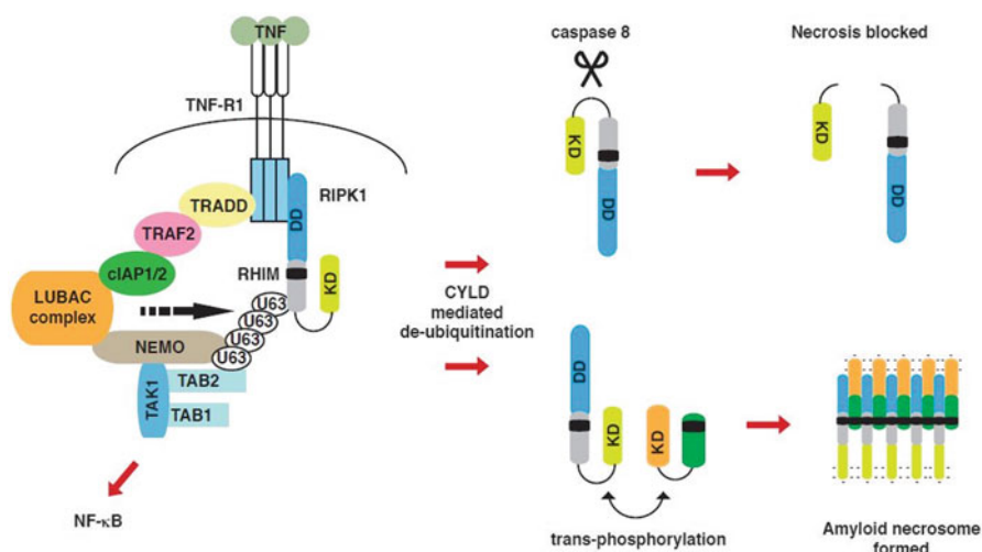
Fig. 10.1 The necrosis signaling pathway is regulated by protein ubiquitination, phosphorylation, and proteolytic cleavage. The TNFR-1-associated membrane complex (Complex I) is composed of many adaptors. Many of the molecular interactions within this complex require protein ubiquitination. RIPK1 ubiquitination through K63 linkage (U63), which is crucial for downstream NF- \kappa B activation, is highlighted . Removal of ubiquitin chains from RIPK1 by the de-ubiquitinase cylindromatosis (CYLD) is important for transition of Complex I to the cytosol and assembly of Complex II. In the presence of active caspase 8, RIPK1, RIPK3, and CYLD are cleaved and inactivated (only RIPK1 cleavage is shown for simplicity sake). Cleavage of RIPK1 removes the kinase domain, thereby preventing phosphorylation of downstream substrates (e.g., RIPK3) that are important for necrosis induction. When the integrity of RIPK1 and RIPK3 is preserved, they trans-phosphorylate each other. The resulting negative charge may be critical in “opening up” the RHIM domain to facilitate amyloid fibril assembly and recruitment of downstream RIPK3 substrates
