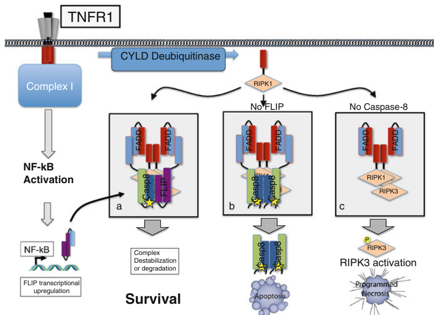
Fig. 6.2 TNF-induced complexes and their effects. TNFR1 ligation leads to NF-κB activation. Thereafter, RIPK1 translocates from the receptor-proximal complex into the cytosol, through the action of the deubiquitinase CYLD. In the cytosol, RIPK1 can interact with RIPK3, caspase-8, and FLIP; the relative abundance and activity of these proteins determine cell fate. (a) If both caspase-8 and FLIP are present, RIPK1/RIPK3 signaling is inhibited, and the cell survives. (b) If FLIP is absent, caspase-8 activation proceeds unchecked, resulting in apoptosis. (c) If caspase-8 is absent, RIPK3 signaling dominates, leading to RIPK3-dependent necroptosis
