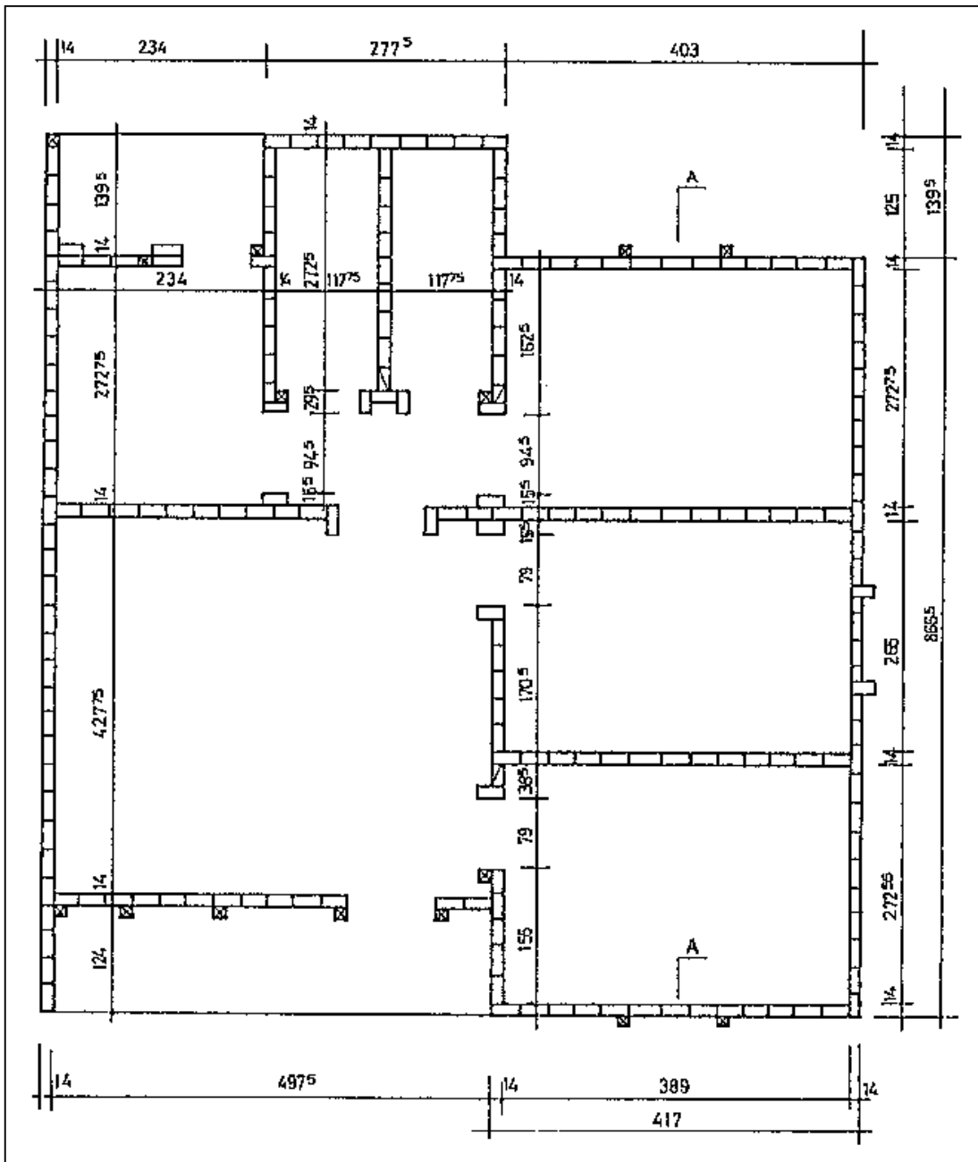
FIGURE COURSING ELEVATIONS
