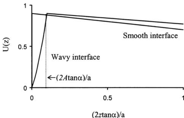
Fig. 7.3. Energy change as a function of interface position for smooth and wavy liquid–air interfaces, d\gamma_{LA}(\cos \theta_0 + 1) = 0.9 , \gamma_{LA}(\cos \theta_0 + \cos \alpha) / \sin \alpha = -0.2 , \gamma_{LA}(\cos \theta_0 + (kL_0/2\pi) \cos \alpha) / \sin \alpha = -0.15 , E_0 = 0.015 , A = 0.1 [241]
