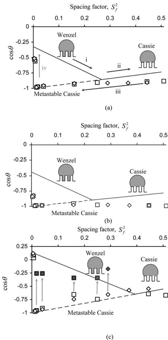
Fig. 8.6. Theoretical ( solid and dashed ) and experimental ( squares for the 1st series, diamonds for the 2nd series) a contact angle as a function of the spacing factor, b advancing contact angle, and c receding contact angle and values of the contact angle observed after the transition during evaporation ( shaded ) [250]
