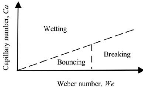
Fig. 9.6. Schematic of various regimes of a droplet impacting a hydrophobic surface. For high We , droplet will break into parts, whereas for high Re = We/Ca , the energy will be dissipated due to the viscosity and the droplet can wet the surface
