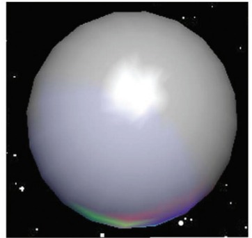
Sphere
