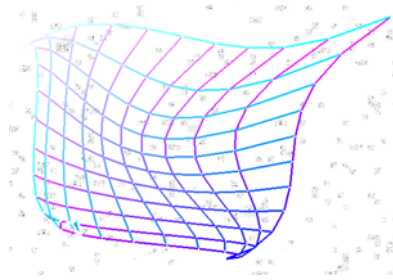
Fig. 5.8 Bezier surfaces
