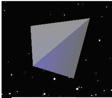
Tetrahedron
