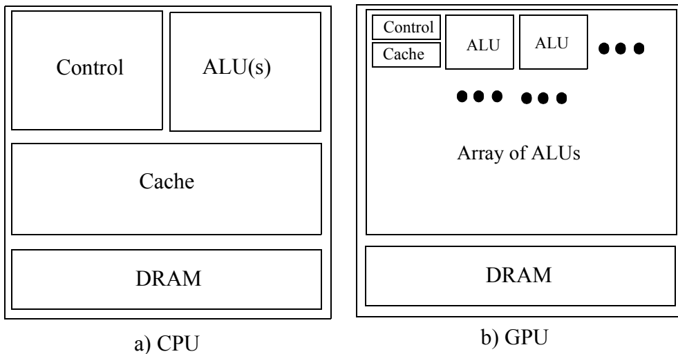
Fig. 6.3 GPU has more transistors for data processing
