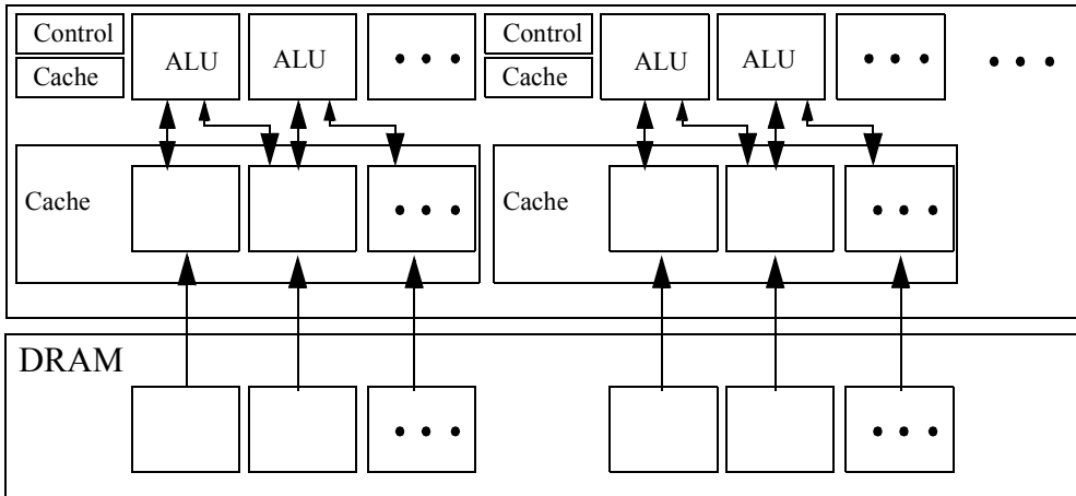
Fig. 6.4 GPU shared cache memory
