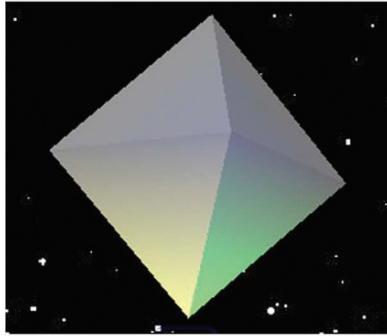
Octahedron
