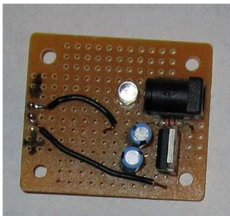
Figure B-1. A small voltage regulator circuit
