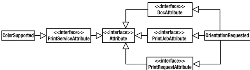
Figure 11-2. The class hierarchy of a portion of the javax.print.attribute package
