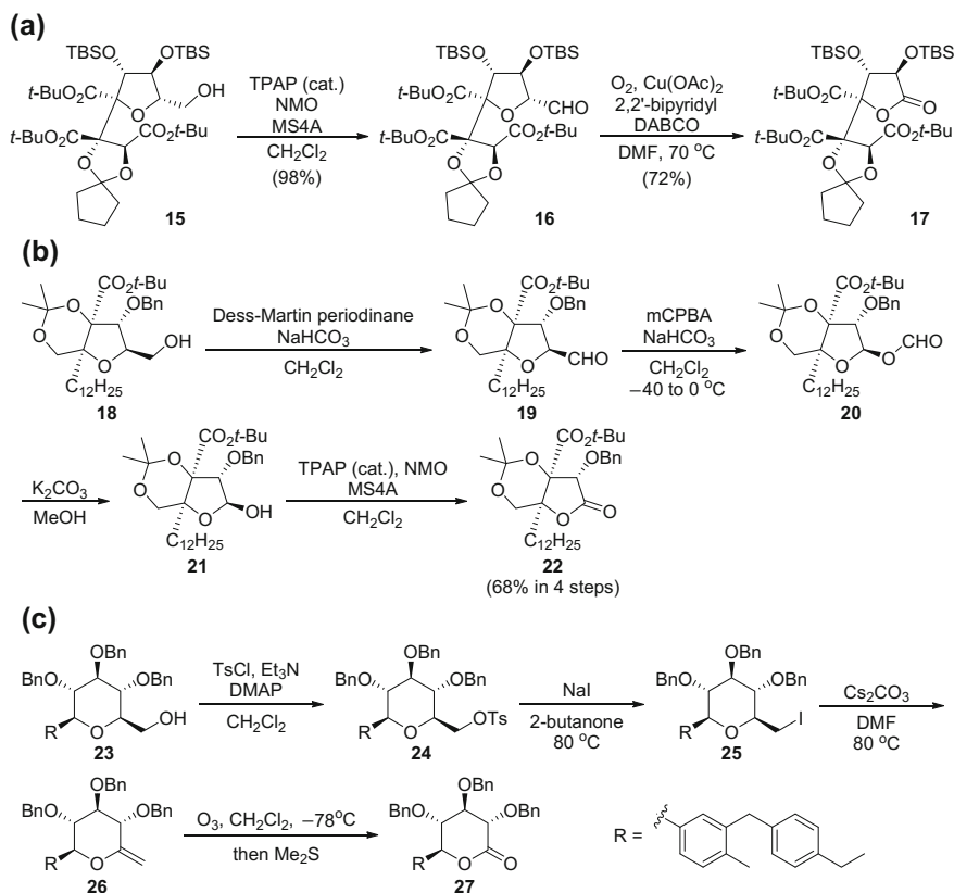
Scheme 3 Multistep conversions
