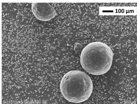
Fig. 3 SEM image of 0.5% Pd/SC after its second use test at 200 magnification
