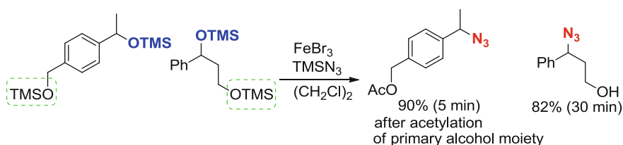
Fig. 4 Chemoselective azidation
