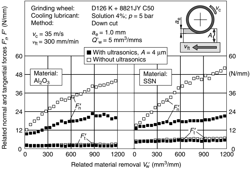
FIGURE 17.15 Related process forces during creep feed grinding with and without ultrasonic assistance.
