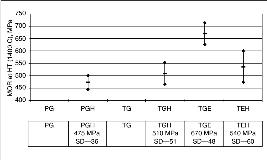
FIGURE 5.38 The effect of ELID grinding on the strength of Si 3 N 4 (at elevated temperature).
