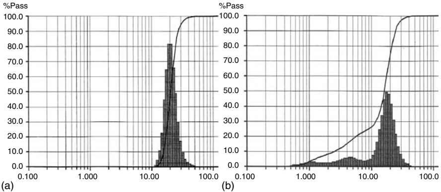
FIGURE 10.7 Grain size distribution for 25 \mu\text{m} monocrystalline diamond: (a) before lapping; (b) after lapping.
