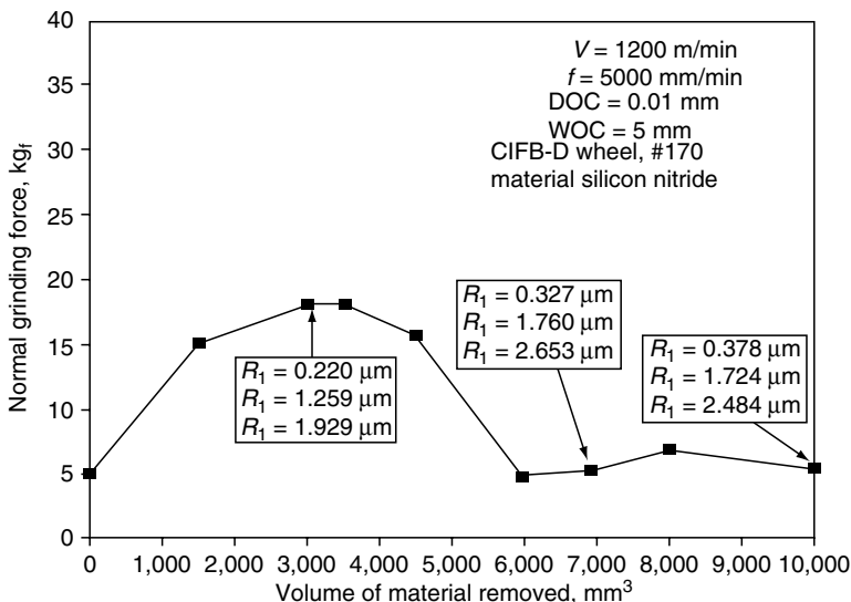
FIGURE 5.19 Relationship between the volume of material removed and the normal grinding force (ELID grinding); V = 90 V; I_p = 24 A; \tau_{on} = \tau_{off} = 4 μsec.
