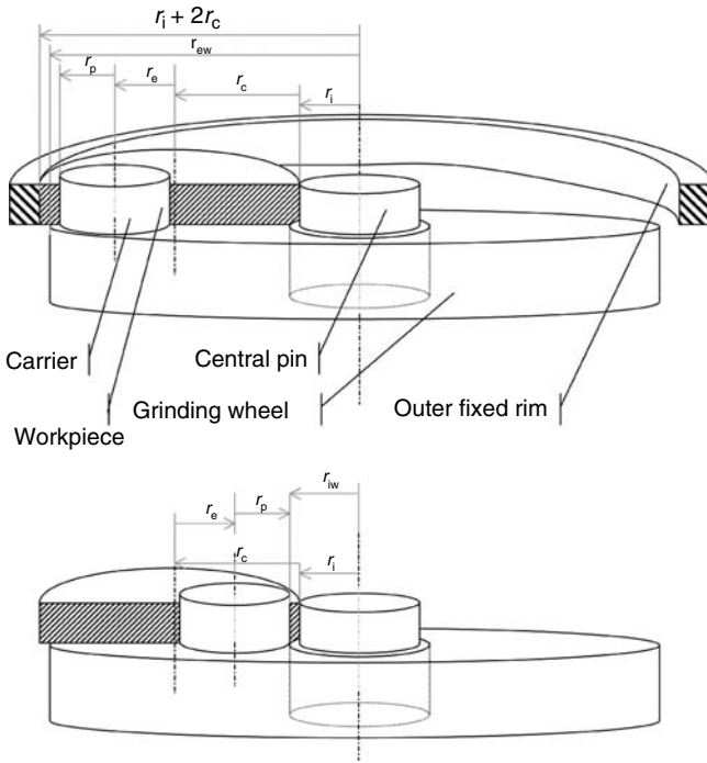
FIGURE 12.3 Dimensional chains for the workpiece offset value with respect to the center of carrier.
