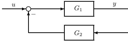
Figure 12.13.3 Feedback Interconnection of Linear Systems
