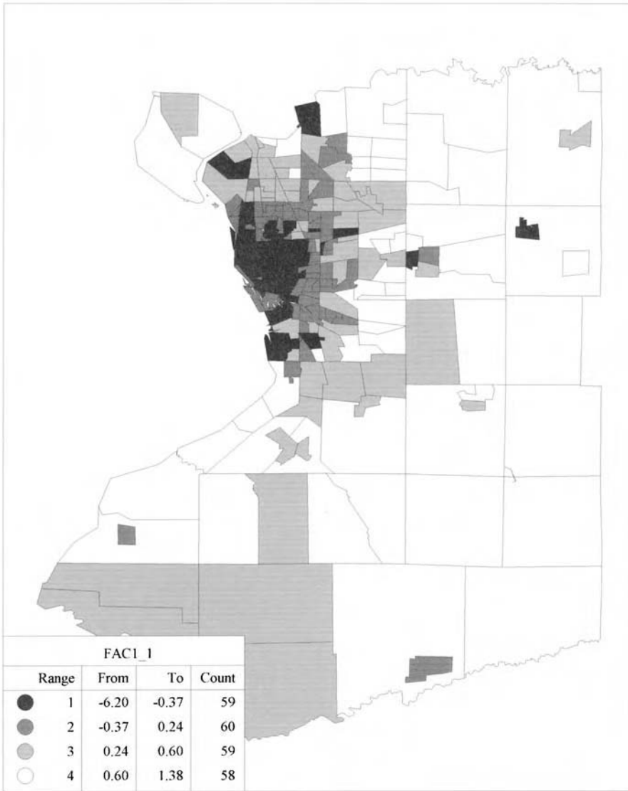
Figure 10.3 Factor 1 scores
