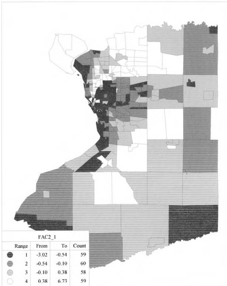
Figure 10.4 Factor 2 scores
