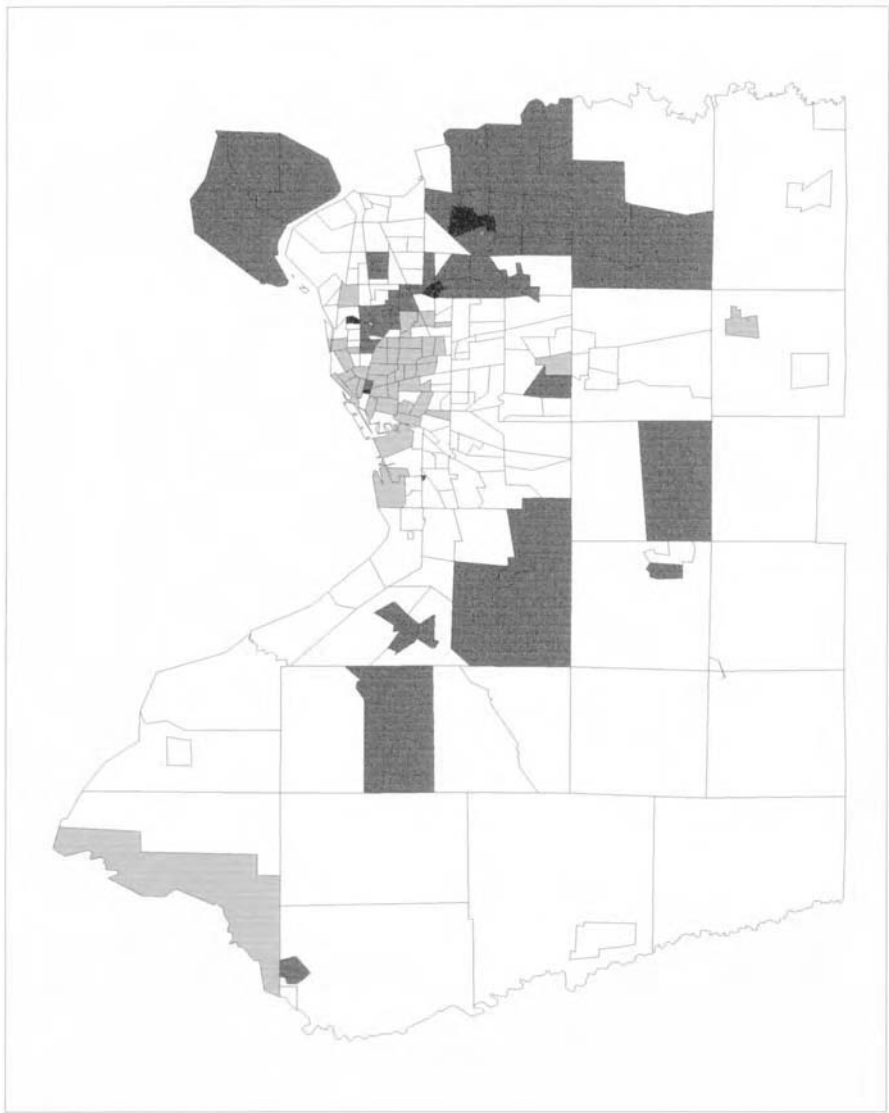
Figure 10.6 Three-cluster solution
