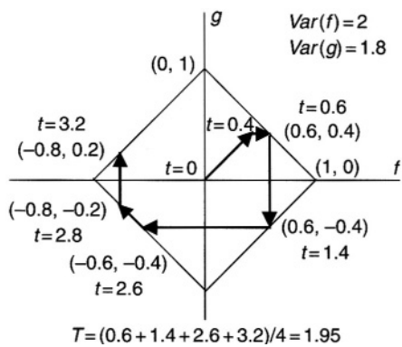
Figure 17.3. Optimal strategy, a = 2, b = 1.8
