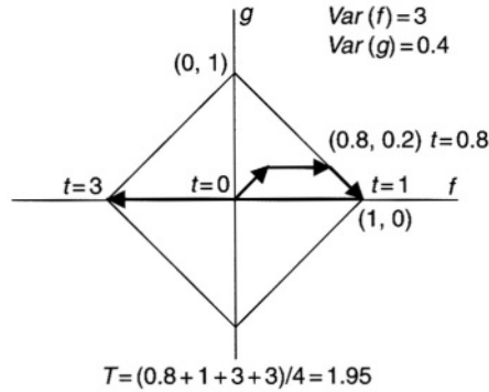
Figure 17.5. Optimal strategy for a \geq 3 , b = 0.4
