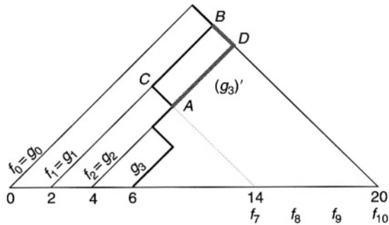
Figure 13.4. Modification of original strategy
