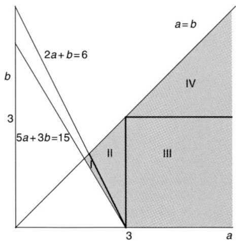
Figure 17.2. Regions I-IV in ab space
