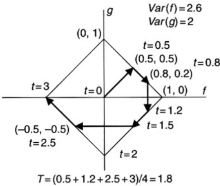
Figure 17.4. Optimal strategy for a = 2.6, b = 2
