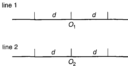
Figure 16.2. Double linear search problem
