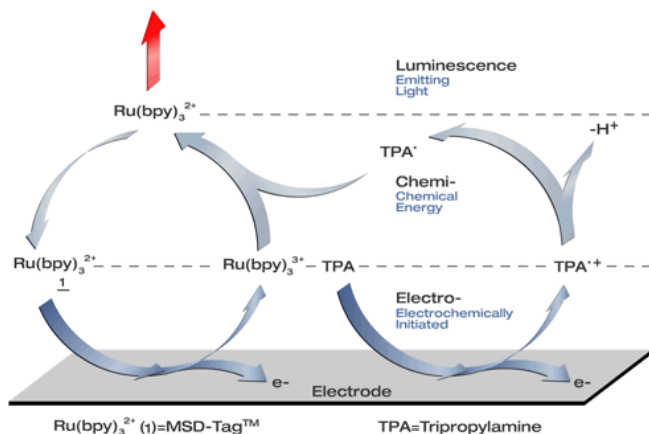
FIGURE H-8 Representation of the electrochemical light generating reporter system for MesoScale technology.
