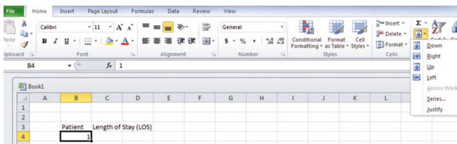
Fig. 1.2 Home/Fill/Series commands
