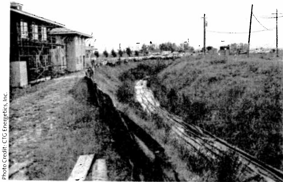
Example of Structural Control. Silt fence: fabric filter media removes sediment from stormwater volumes flowing through the fence.
