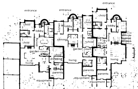
11 Single-family courtyard houses
