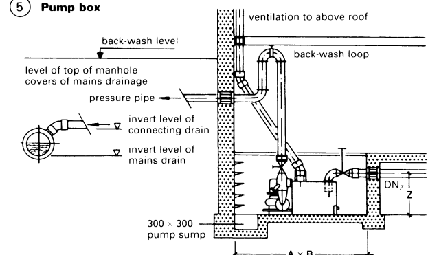
⑤ Pump box
