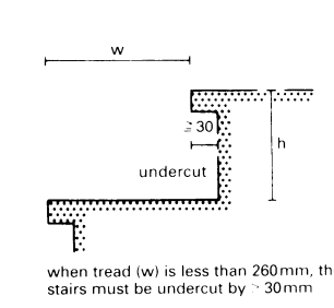
⑯ The proportions of the stair rises must not change as you go up
