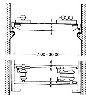
⑭ Double-girder gantry crane (capacity: 2-20t)
