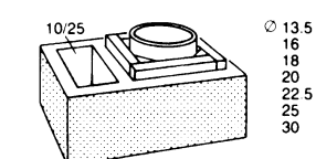
⑧ Modular flue with ventilation duct
