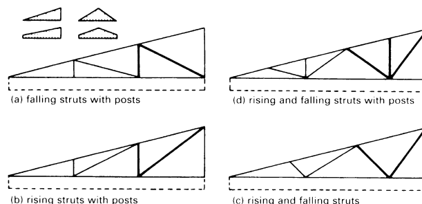
⑧ Timber construction forms and reinforcements
