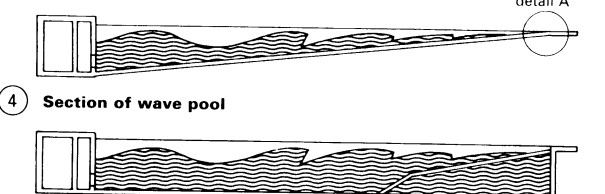
4 Section of wave pool
