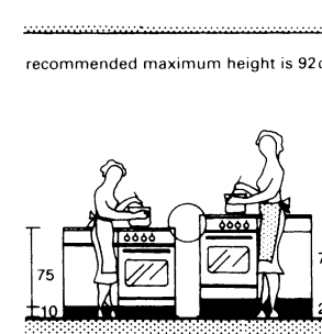
⑲ Plinth depth varies height of work surface
