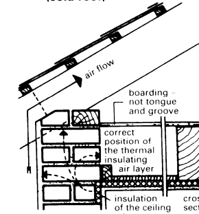
⑩ Pitched roof with timber beam ceiling
