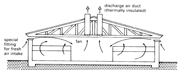
9 Extract ventilation
