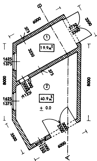
③ Standard method of dimensioning an oddly shaped plan (measurements given are structural dimensions)
