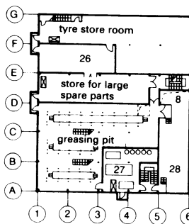
3 Workshop for transport vehicles, ground floor
