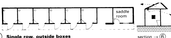
6 Single row, outside boxes
