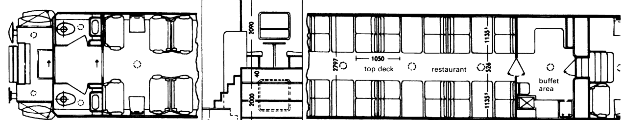
⑤ Top deck: 4-axle double-decker carriage
