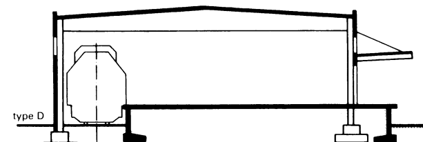
④ Examples of goods sheds: A, B, and C with siding outside, D with siding inside
