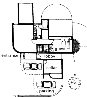
3 Ground floor, house in California → 4 + 5
