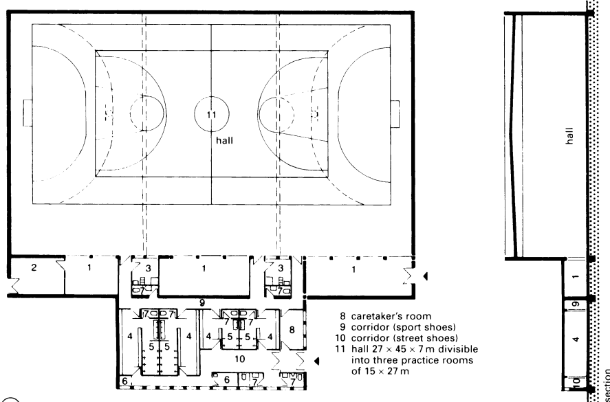
② Plan layout of a triple sports hall
