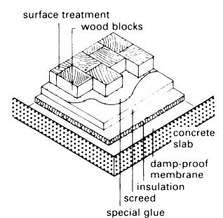
⑩ Construction of surface treated, glued wood-block floor
