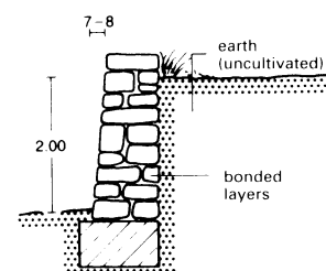
㉔ Dry wall, special drainage unnecessary
