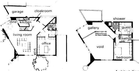
5 Ground floor → 6 6 Upper floor Architect: Kargel
