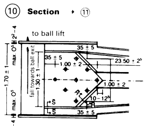
⑩ Skittle area
