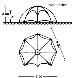
② Domed construction
