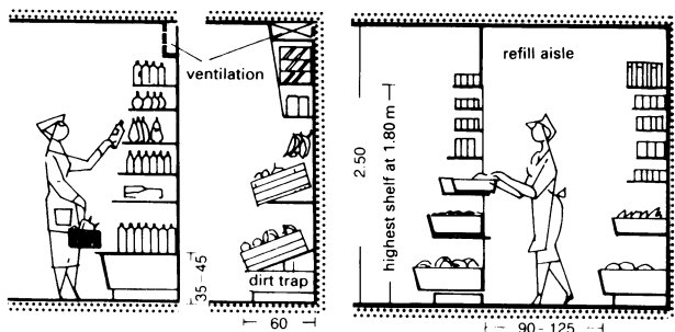
① Shelves for bottles Shelves for fruit, vegetables and loose goods ② Partition allowing replacement of containers from refill aisle
