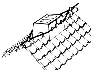
7 Chimney on ridge with angled steel strips as lightning conductor
