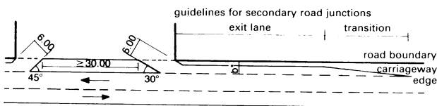
5 Filling station entrance and exit off an open road
