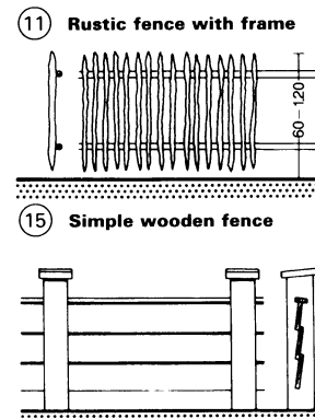
⑮ Simple wooden fence
