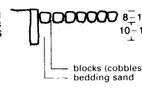
⑰ Small paving blocks, expensive but durable
