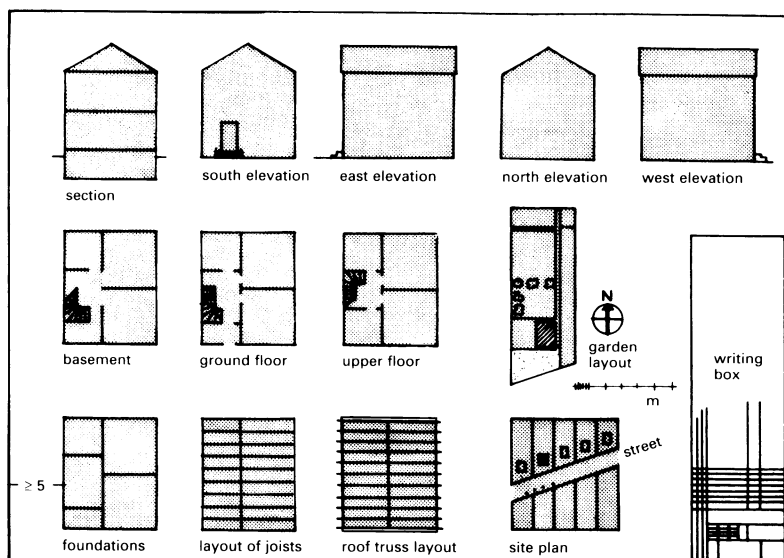
① Suitable arrangement of a construction drawing
