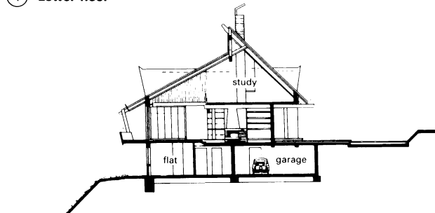
⑥ Section
