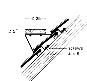
⑭ Crawling boards are fixed more firmly to rafters than to the tile battens
