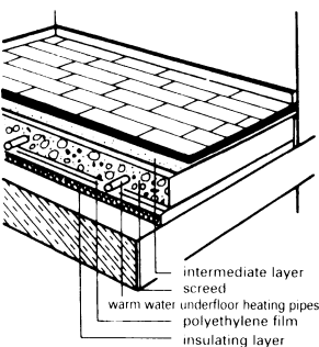
⑪②① Finished parquet flooring elements on underfloor heating
