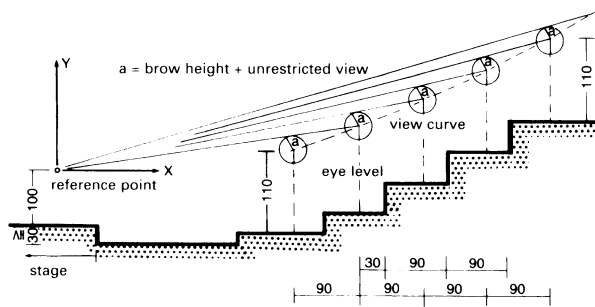
② Drawing for calculating view curve
