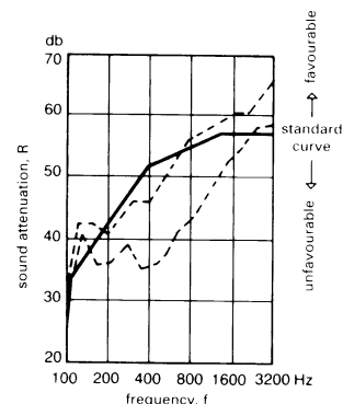
⑦ Airborne sound insulation of the wall \rightarrow ① from measurements by Prof. Gäsele: sound insulation without covering -7 dB; with covering +2 dB
