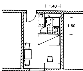
⑮ Shower cubicle in the smallest flat
