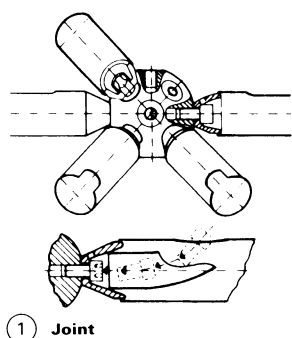
① Joint
