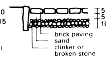
⑱ Brick paving
