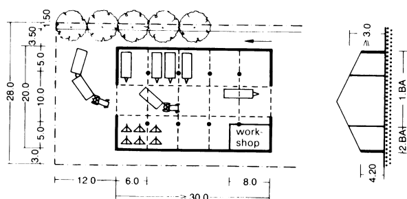
⑦ Large machine shed with central gangway: supported structure
