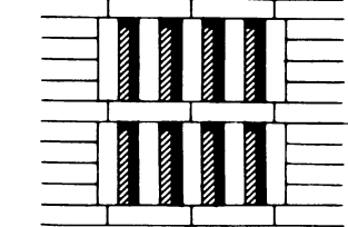
㉗ As 25 (holes 1 x 1/4 brick)
