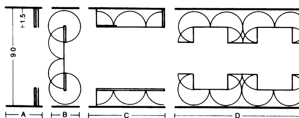
⑧ Exhibition room with folding screens (design: K. Schneider) allows great variety of room arrangements
