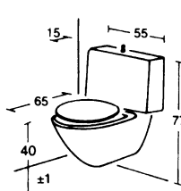
⑦ Wall-mounted deep-flush toilet bowl and cistern
