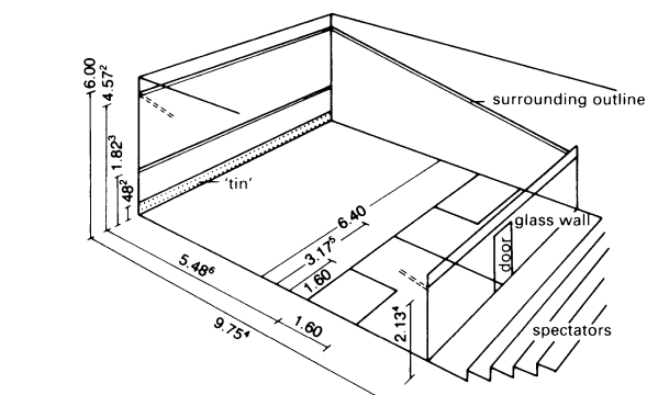
③ Basic dimensions for squash courts
