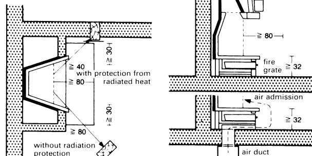
6 Separation of fireplace opening from combustible materials
