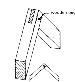
⑬ Simple tenon joint connecting two rafters
