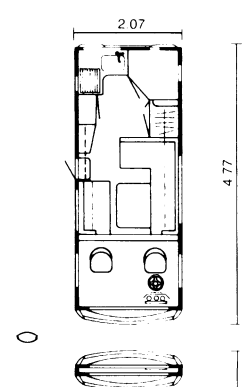
⑮ Camper: Lyding ROG2
