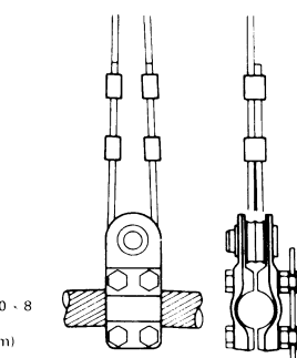
⑬ Cable network; edge cable clamp
