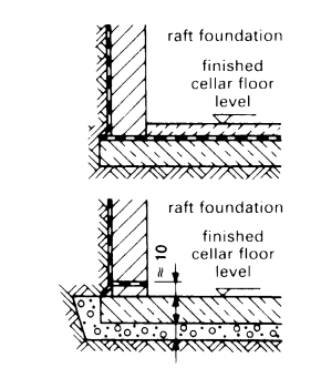
⑫ Damp-proofing and tanking of building with cellar; masonry walls on a raft foundation
