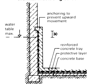
⑩ Tanking over expansion joint in reinforced concrete slab; thermal insulating screed
