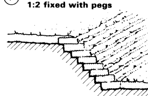
⑧ Binding with stepped turf
