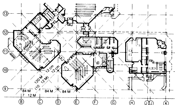
⑥ Application of rotation about 45° using 12M in the plan view
