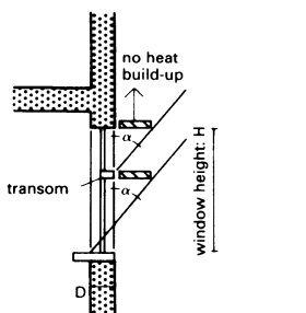
⑧ Double sun shades
