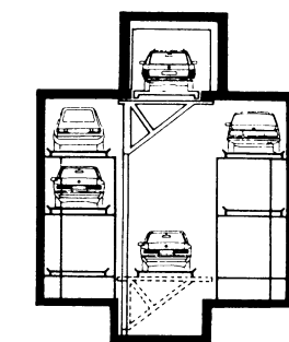
⑭ Parksafes system
