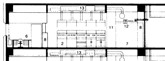
⑤ BASF plastics laboratory: section
