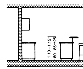
⑯ A breakfast bar arrangement
