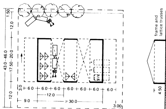
⑩ Large machine and equipment shed with through-gangways
