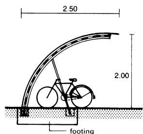
⑬ Weather protection roof - curved roof
