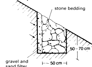
⑪ Drainage and support of slope base
