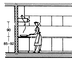
⑭ Extractor hood: better than just a fan
