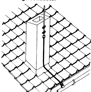
10 Lightning conductors on chimneys close to the eaves connected to the roof guttering
