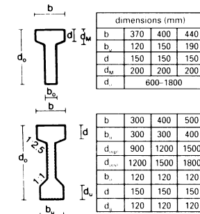
⑬ Pre-cast concrete elements - roof beam: T section I section
