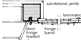
house door, old condition (horizontal section)
