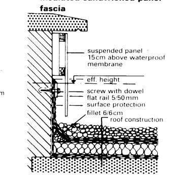
21 Chimney connection with suspended fascia panel
