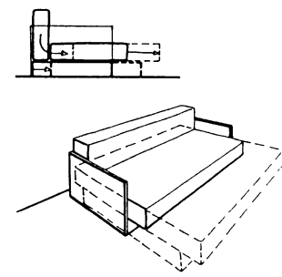
8 Sofa-bed: pull-out mattress
