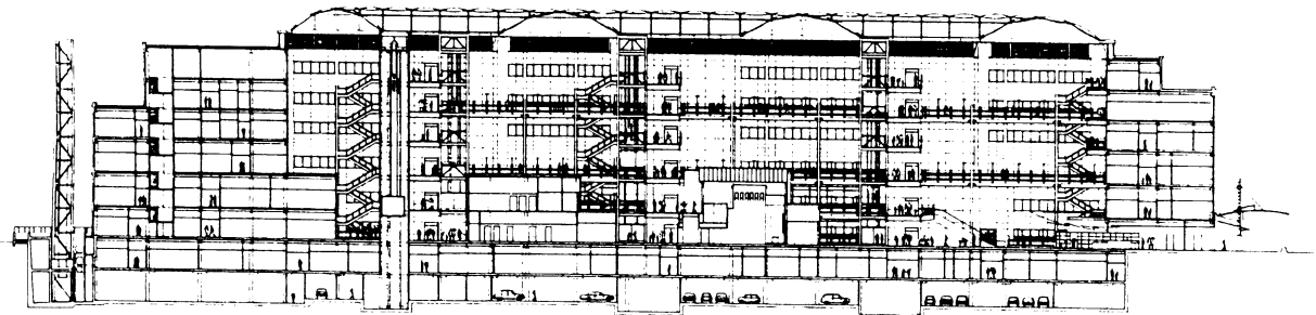
② Section
