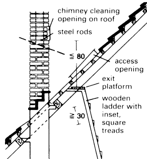
⑪ Access opening with ladder and platform
