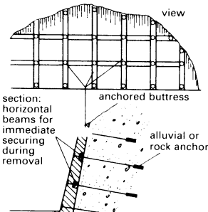
10 Retention considerations: multi-strata slope
