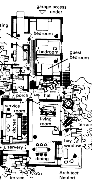
④ Improved design for ③: better room plans; bedrooms 2.5m above ground, using the site's natural slope; garage at ground level
