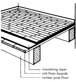
⑪②② Finished parquet flooring elements on old wooden floor
