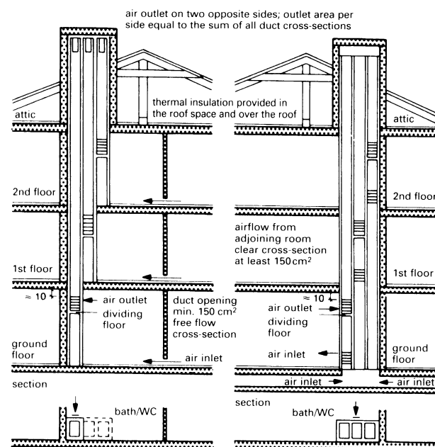
7 Single duct convection ventilation system 8 Supply and extract convection ventilation system
