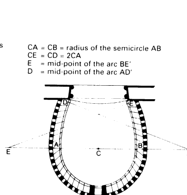
⑩ Design of the curve of the auditorium in the Teatro alla Scala in Milan
