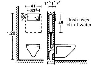
⑨ Deep-flush toilet bowl; built-in cistern
