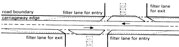
6 Filling stations on both sides of open road
