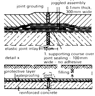
⑨ Details: tanking between two walls
