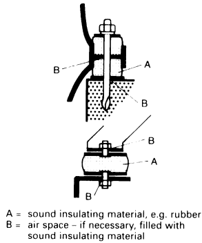
③ Metal/rubber element
