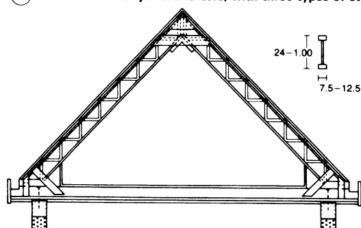
③ Couple close roof in timber framing with lifetime guaranteed glued joints with 45^\circ inclined struts as twinned supports over span < 25\text{m}
