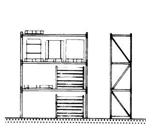
⑭ Pallet racks of prefabricated components (longitudinal transverse shelving)
