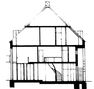
12 Section
