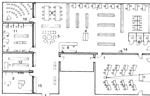
② Example of school library/media centre
