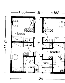
12 Pavilion with 14 beds
