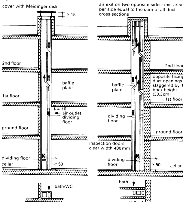
11 Branching duct ventilation system with one main and one auxiliary duct 12 Example of system with one main duct and two auxiliary ducts
