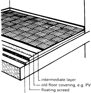
⑪⑨ Finished parquet elements on old floor covering
