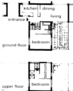
10 Courtyard house on two floors
