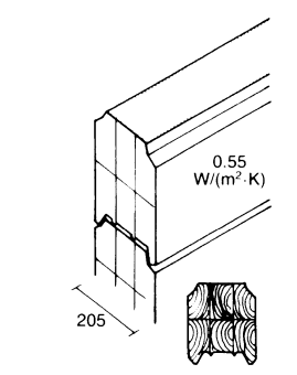
13 Profiled laminated timber log construction
