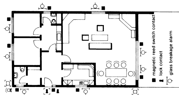
3 Outer perimeter security on private premises
