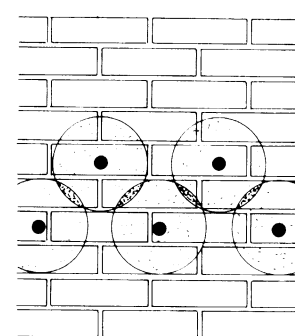
9 Injected damp-proofing
