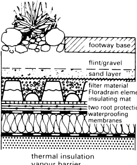
6 Zinco Floradrain roof cultivation system
