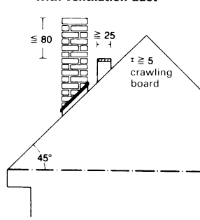
⑫ A crawling board is necessary for roof slopes above 15^\circ
