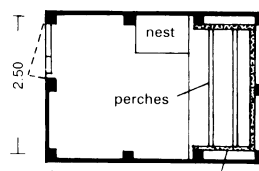
6 Laying nest with flap
