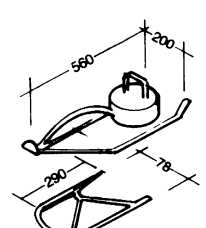
⑭ Lawn sprinklers
