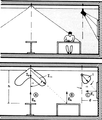
⑤ Illuminance at a point (A) E_h = \frac{I_0}{r^2} (B) E_h = \frac{I_{ct}}{r^2} \cdot \cos^3 \alpha (C) E_v = \frac{I_{ct}}{d^2} \cdot \cos^3 (90 - \alpha)
