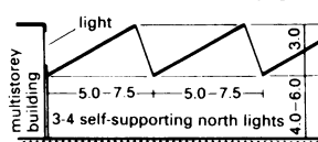
section through north light roof (self-supporting) like lattice girder
