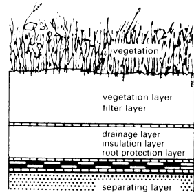
3 Layer construction of a cultivated roof
