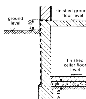
⑪ Damp-proofing and tanking of building with cellar; walls of concrete
