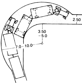
④ Minimum space required for traffic
