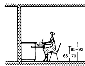
⑪ Pull-out worktop for use when seated
