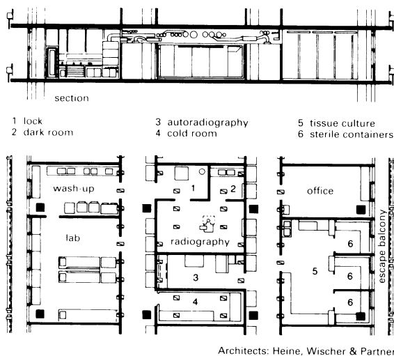
① Part of plan of cancer research centre in Heidelberg
