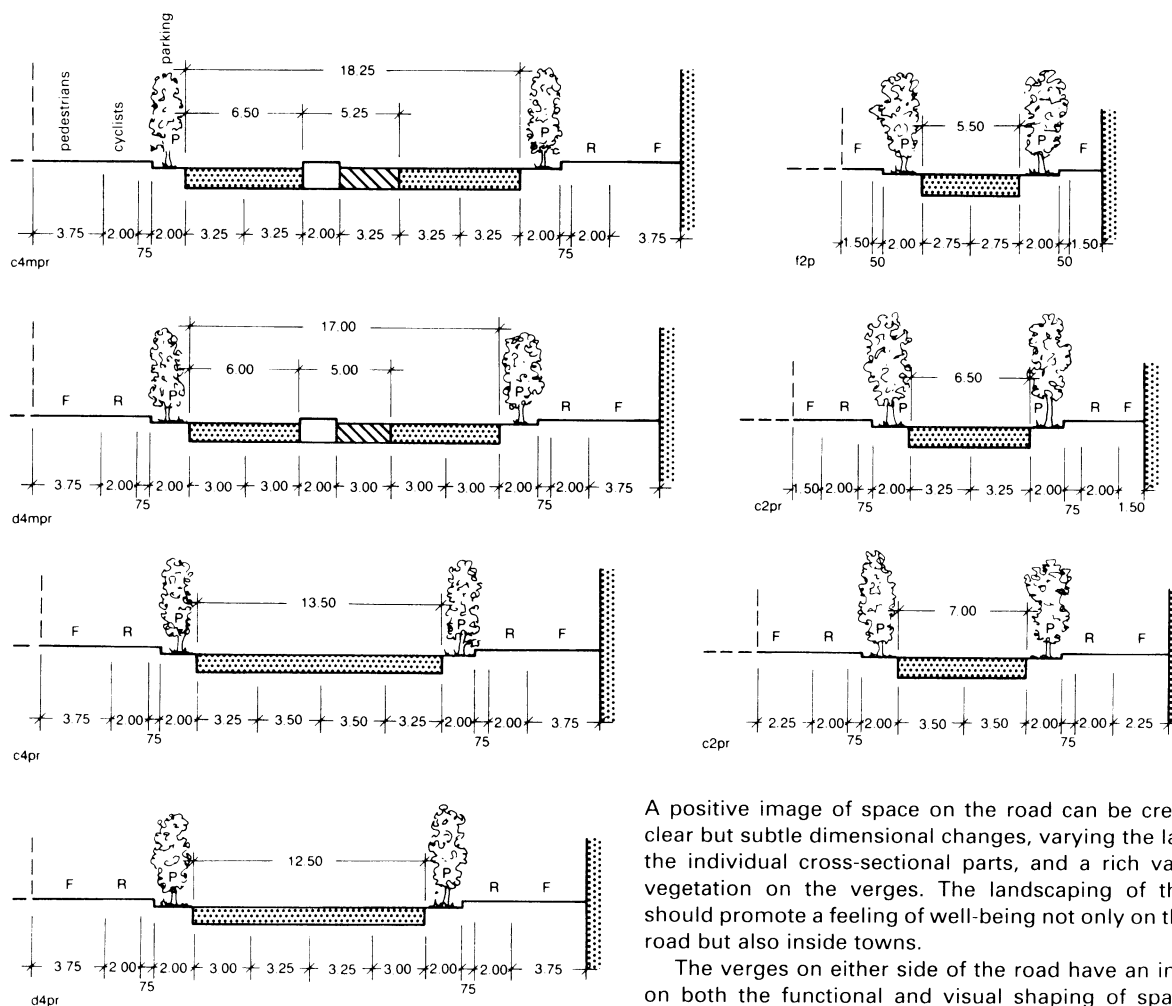
2 Standard cross-sections for roads in built-up areas
