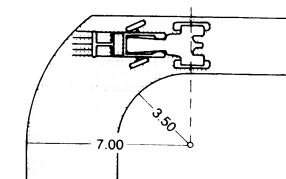
② Tractor with front loader
