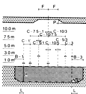
7 Cross-section
