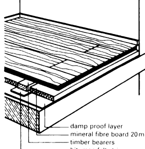
⑪⑩ Finished parquet elements on timber battens
