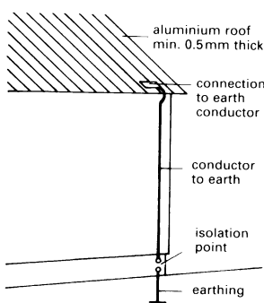
4 Aluminium roof decking used as a lightning conductor
