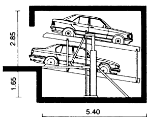
② Suspended parking (no pit)
