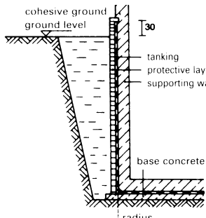
⑥ Continuous water pressure resistant tanking
