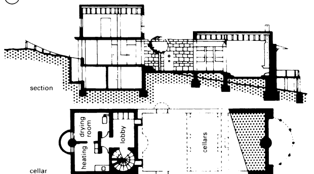
⑩ Section and cellar
