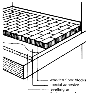
⑪③ Wooden floor blocks, glued down, with surface treatment (living area)
