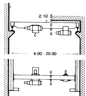
⑬ Simple-girder gantry crane (capacity: 0.5-6.0t)
