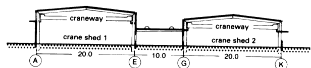
7 Cross-section, axis 16
