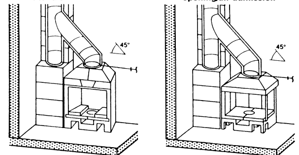
9 Fireplace open on one side
