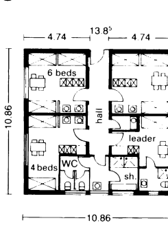
11 Uslar youth hostel; pavilion with 18 beds
