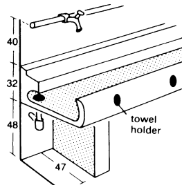
② Row washing trough (Rotter system)
