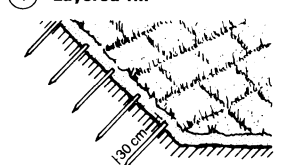
⑦ Turf on slopes of more than 1:2 fixed with pegs
