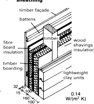
11 Timber frame with lightweight clay elements
