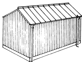
2 Sheeted roof with wooden walls: roof connected to ridge conductor and the conductor to earth
