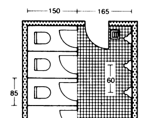
⑧ As ⑦ but with doors opening inwards
