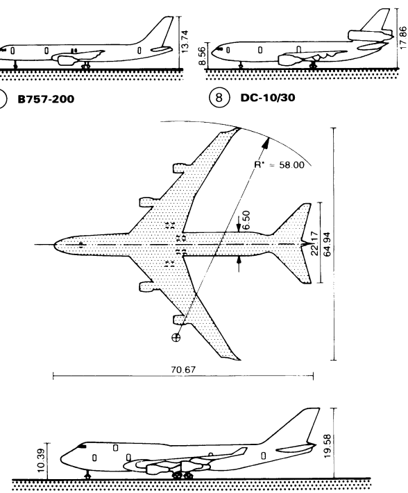
9 B747-400
