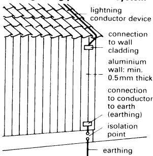
5 Aluminium wall cladding used as a conductor to earth
