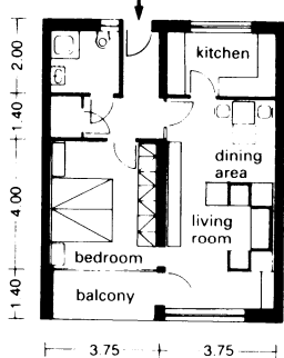
⑤ Two-person apartment 58 m²
