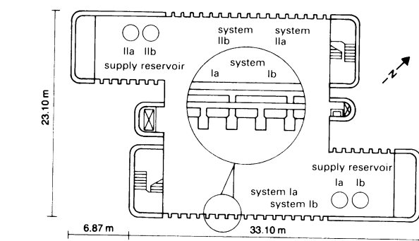
③ Water cooling scheme
