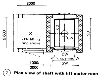
2 Plan view of shaft with lift motor room
