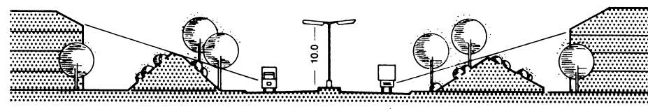
9 Sound protection is good with side embankments
