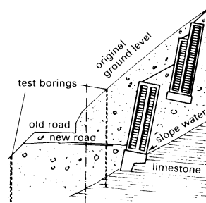
15 Wall with land anchors (Lüdenschaid example)
