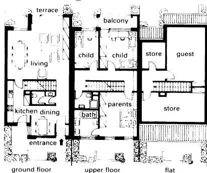
9 Terraced houses with transverse stairs
