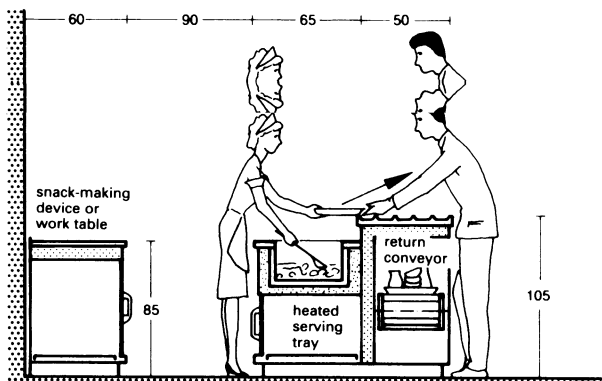
9 Cafeteria: meal servery → ⑧
