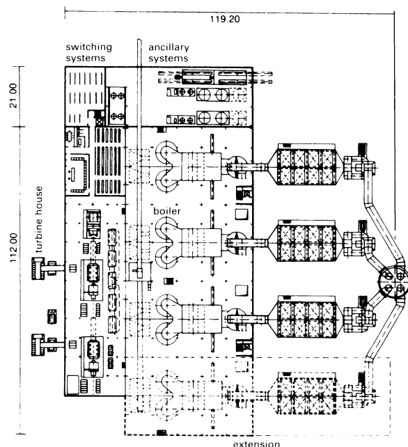
④ Plan of power station with fluidised bed firing
