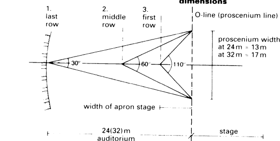
⑦ Proportions of the traditional auditorium (view)
