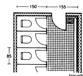
⑥ Doors opening inwards; with urinal trough
