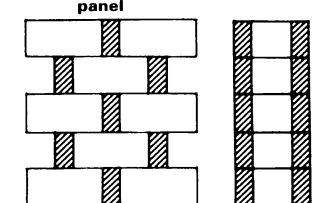
⑳ Cavity wall of 2x1/4 brick leaves bonded by header bricks on edge
