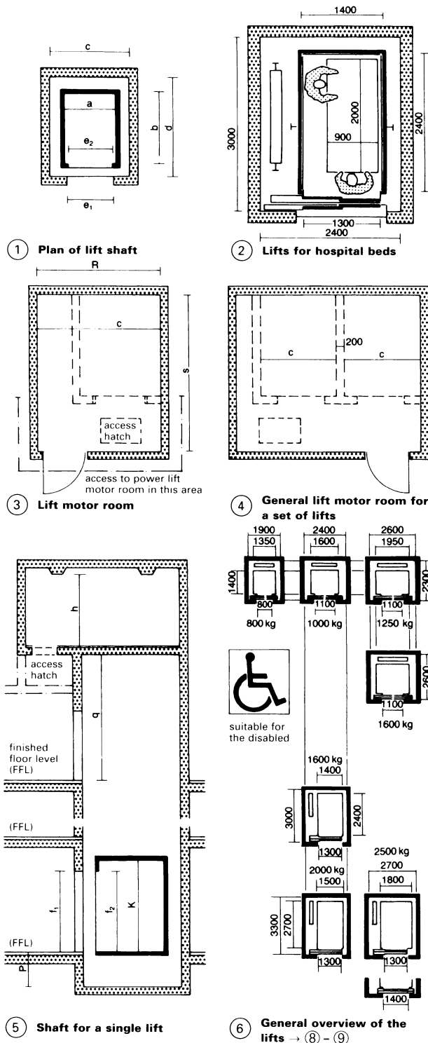
8 Structural dimensions (mm) → (1) - (6): lifts allow wheelchair access
