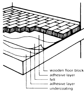
⑪④ Wooden floor blocks, glued down on even, smoothed concrete underlayer (specialised finish)
