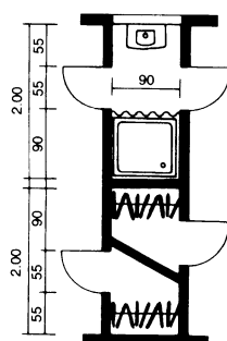
8 Cupboard space and shower between two children's bedrooms
