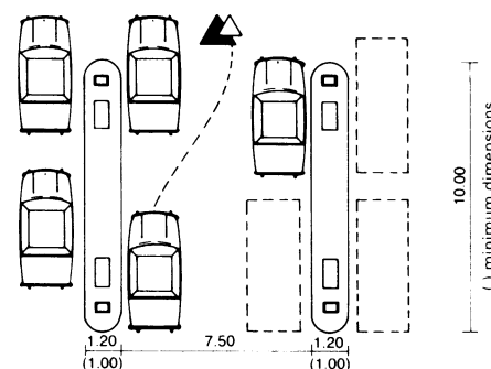
8 2 long islands parallel to the roadway (this requires good driving skills)
