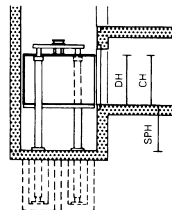
7 Tandem arrangement 1:1
