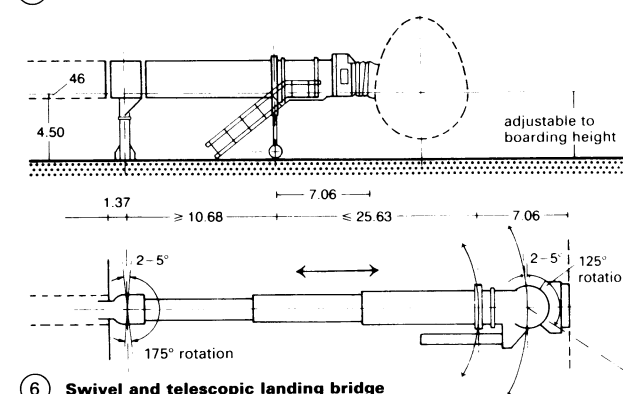
6 Swivel and telescopic landing bridge
