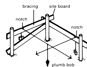
⑨ Corner site boards
