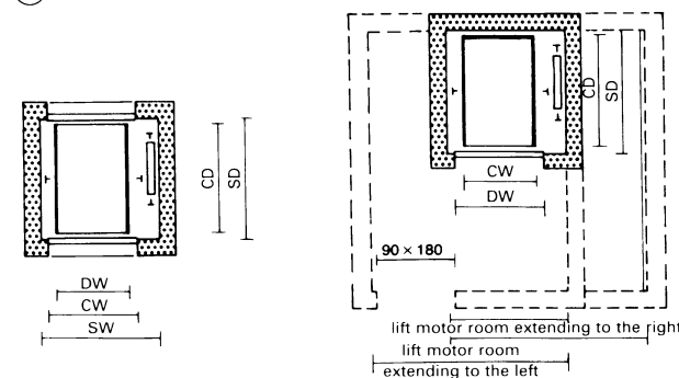
⑧ Goods lift with loading from both sides
