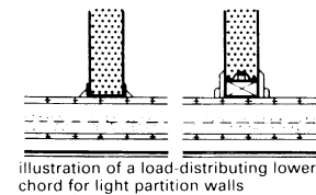
illustration of a load-distributing lower chord for light partition walls
