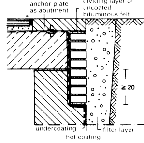
⑬ Tanking at junctions of slab bearing on retaining wall
