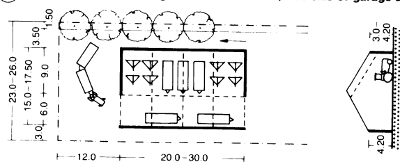
⑥ Small machine shed with side gangway
