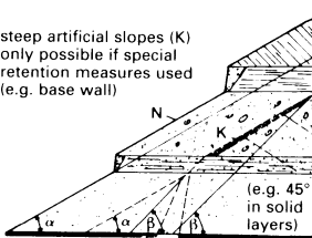
12 Geological influence on slope retention
