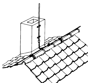
8 Chimneys with lightning conductor connected to the ridge conductor
