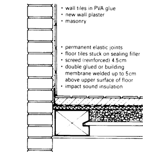
13 Floor/wall structure in damp areas in a masonry building with wooden beam floors
