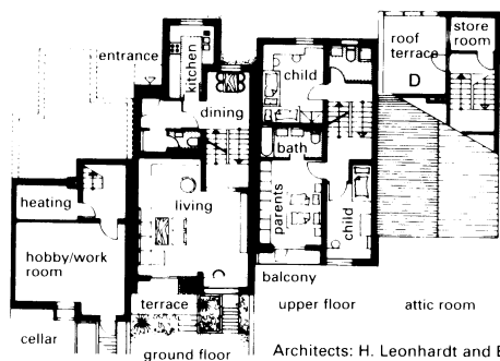
1 Row of terraced houses with offset levels
