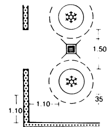
⑧ Space requirement for circular wash-basins
