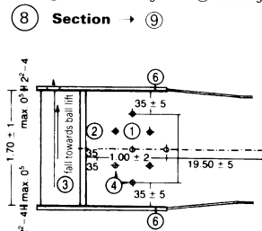
⑨ Normal arrangement of skittle area
