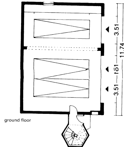
④ Fire station for two appliances
