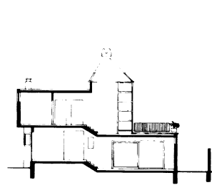
15 Section → 13 + 14
