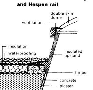
15 Double skin dome with ventilation gap → p. 159
