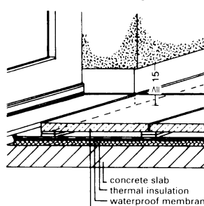
10 Wall connection zinc sheet angle and flashing
