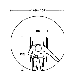
⑫ Minimum turning circle
