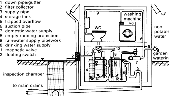
9 Rainwater system
