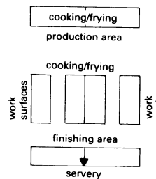
⑧ French system for hotel kitchens; cooking area at right angles to the servery; split production/finishing
