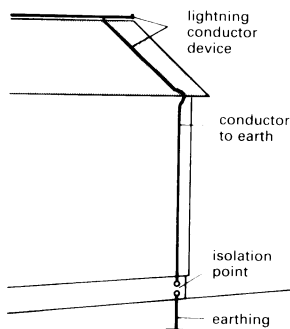
3 The main components of a lightning protection system
