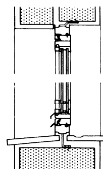
③ Profiled steel tube windows
