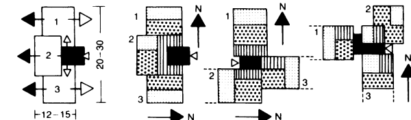
③ Three dwellings per floor, staircase access
