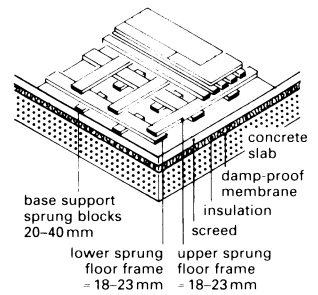
⑦ Sprung floor construction
