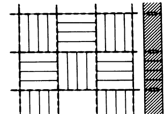
⑯ Reinforced brick wall, 1/2 brick thick with 4 brick panel
