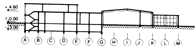
6 Cross-section, axis 5
