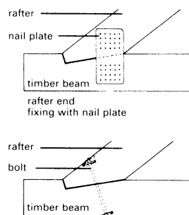
⑨ Rafter end fixing with bolts
