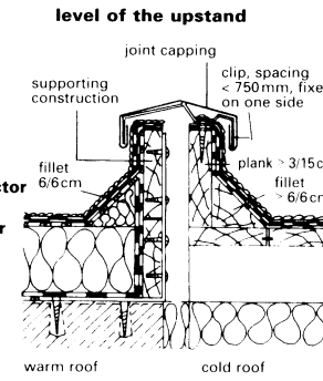
19 Movement joint with supporting construction and capping
