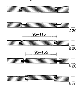
17 Vertical cladding
