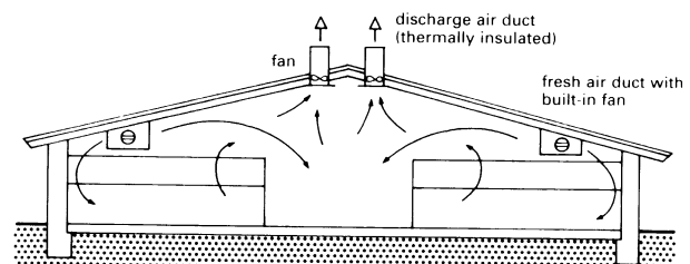
11 Balanced pressure ventilation
