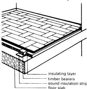
⑪⑧ Finished parquet elements on timber battens
