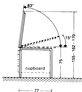
⑪ Section → ⑫
