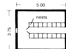
15 Plan of stall
