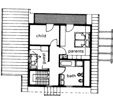
⑧ Attic floor Iller Haus
