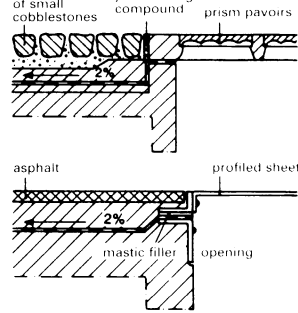
⑫ Subsequently constructed tanking
