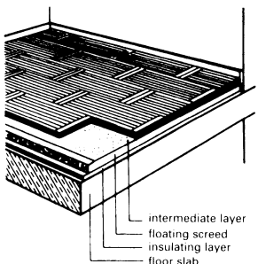
⑪⑦ Finished parquet elements on floor screed
