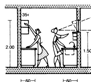
④ Worktops and storage 60cm deep
