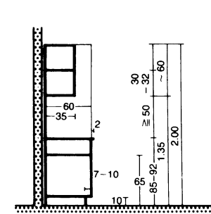
⑰ Section through kitchen units: preferred measurements
