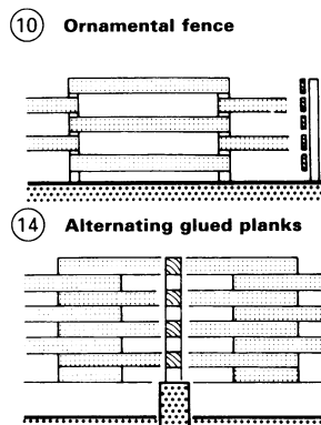
⑭ Alternating glued planks
