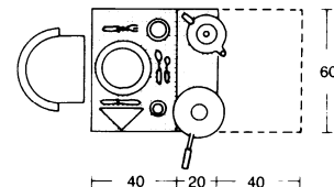
⑯ Dining room and living room, as ⑮, on common patio giving good natural lighting
