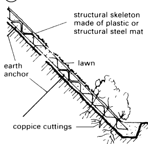
⑩ Preserving bank surface with structural skeleton
