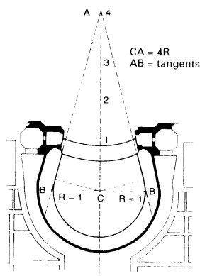
⑨ Design of the contours of the auditorium in the Grand Theatre in Bordeaux
