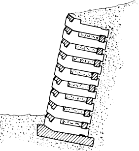
14 RGS 80 wall
