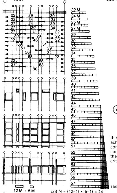
⑤ Combination of component dimensions without a common divisor
