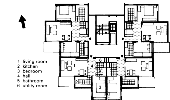
⑧ High-rise block of flats
