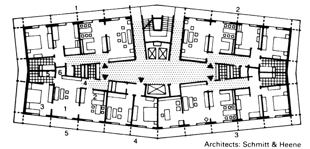
⑦ Standard floor with five residential units
