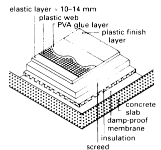
⑨ Impact absorbing floor
