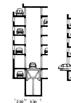
⑫ Transverse stacking
