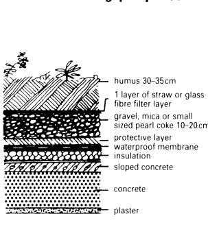
20 Roof garden on a warm roof – protective layer could be replaced by shredded rubber sheet
