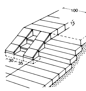
㉕ Concrete block steps with ramp
