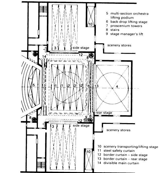
7 Typical opera building (plan view)
