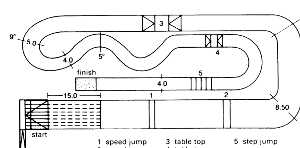
⑬ BMX track at the IFMA '84 in Cologne
