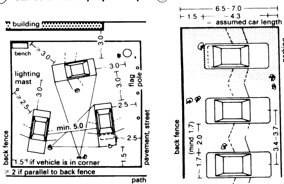
② Average space requirement for a car showroom
