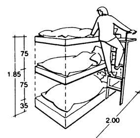
11 Bunk for railway sleeping cars, holiday homes etc.
