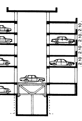
⑬ Cross-section → ⑪
