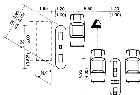
5 2 short islands, < 60^\circ to the roadway ( ) minimum dimensions
