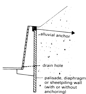
6 Lattice support wall (Krainer wall) made of concrete (Ebensee system)
