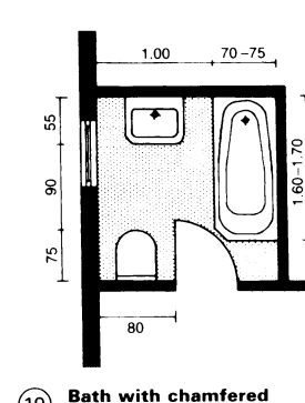
⑲ Bath with chamfered corner (necessitated by limited space)
