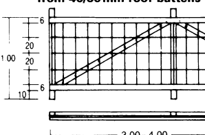
7 Dividing fence: roof battens and knotted network
