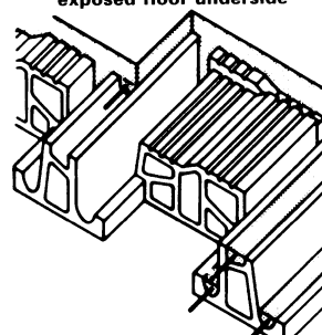
④ Floor assembled from reinforced concrete ribs with cellular clay infill components
