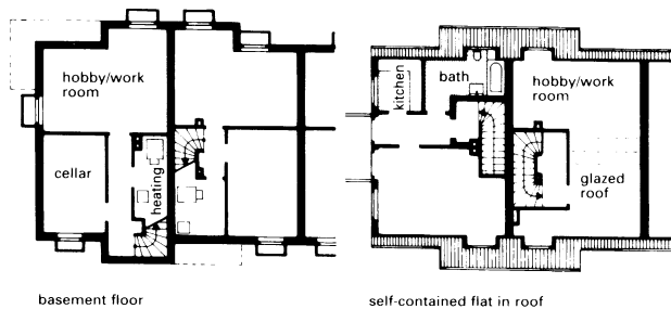
8 Basement and top floor → 7
