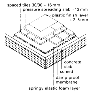
⑧ Flexible floor
