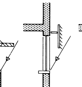
⑲ Cantilevered screen
