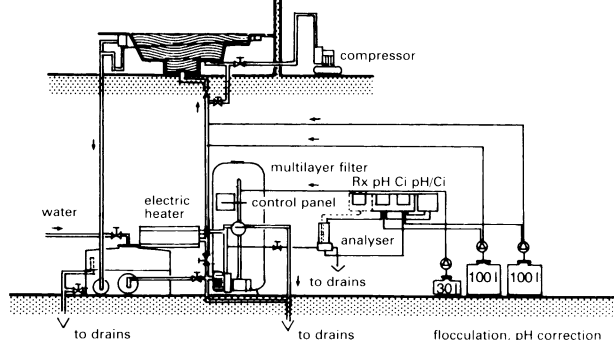
4 Whirlpool servicing diagram
