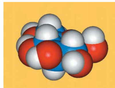
\beta -D-Glucopyranose
