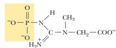
Creatine-P
