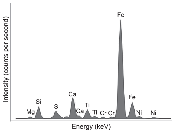
Fig. 4.11 Typical output from XRF analyses. Intensity at each X-ray wavelength indicates the relative amount of an element present
