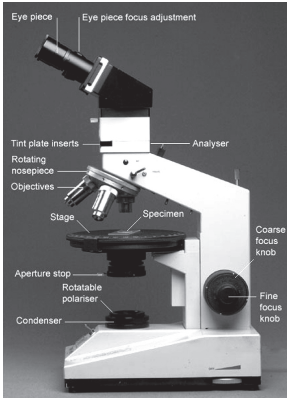
Fig. 4.38 A petrographic microscope with component parts labeled. Image courtesy of the University of Cambridge DoITPoMS Micrograph Library
