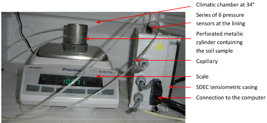
Figure 8.6. Photo of a laboratory device which allows us to measure the hydric conductivity of the soil [PRA 05]
