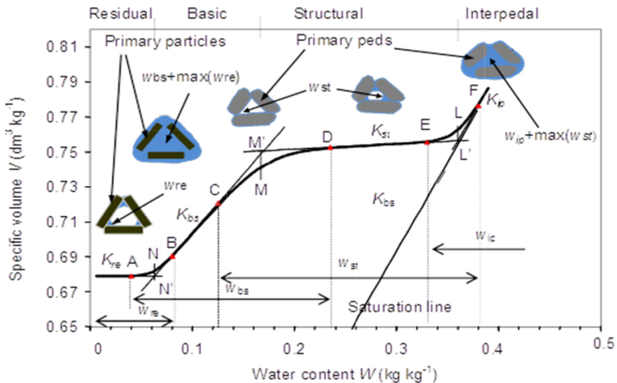
Figure 8.1. A typical soil shrinkage curve of a well-developed and a fine-aggregate soil structure (pedostructure shrinkage curve). The different configuration of water and air distribution in both the inter- and intra-aggregates' spaces of pedostructure, in relation to the different shrinkage phases of the shrinkage curve.
