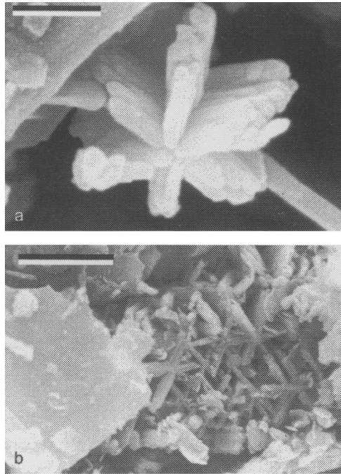
Fig. 3. Powder ores from the Magor Pill boat. (a) Stacked '6-pointed stars' of goethite. Secondary electron image of stew mounted ochre. Scale bar 1 \mu\text{m} . Sample M117. (b) Lattice of '6-pointed stars' of goethite, together with other goethite grains. Secondary electron image of stew mounted ochre. Scale bar 5 \mu\text{m} . Sample M115.
